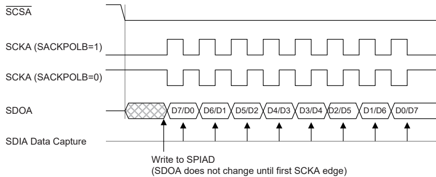
SPIA Master Mode Timing – SACKEG=0
