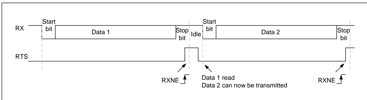
Figure 24-22 RTS flow control
