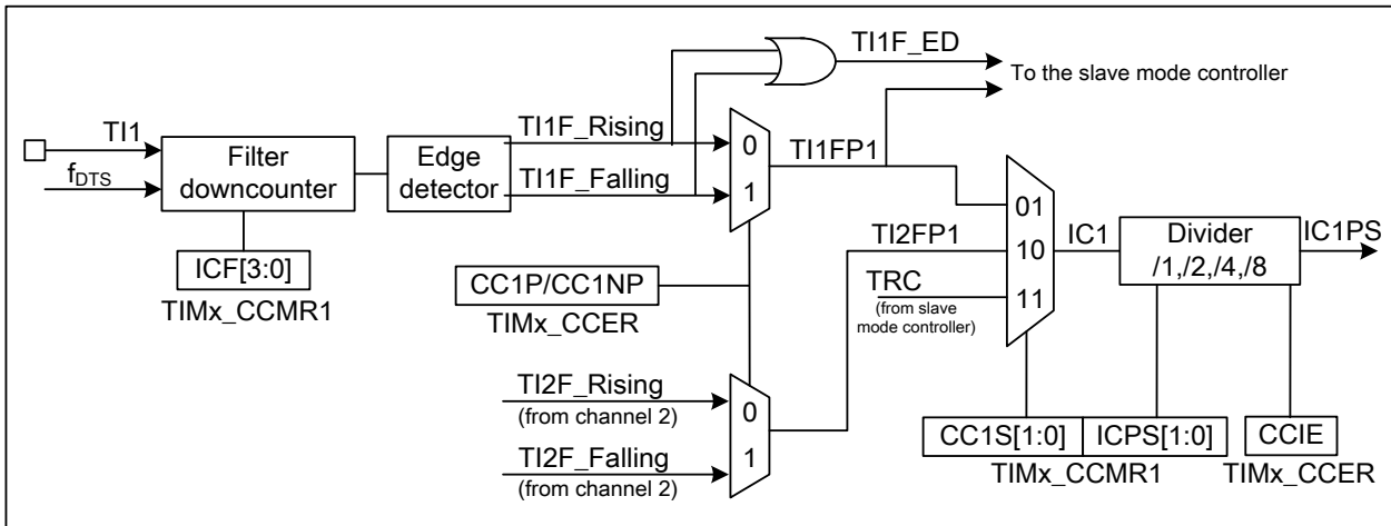
Figure 12-27 Capture/compare channel (example: channel 1 input stage)
