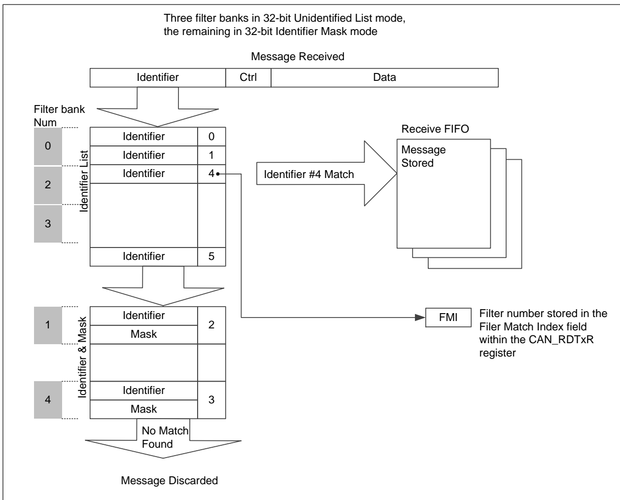
Figure 21-10 Filtering mechanism - Example
