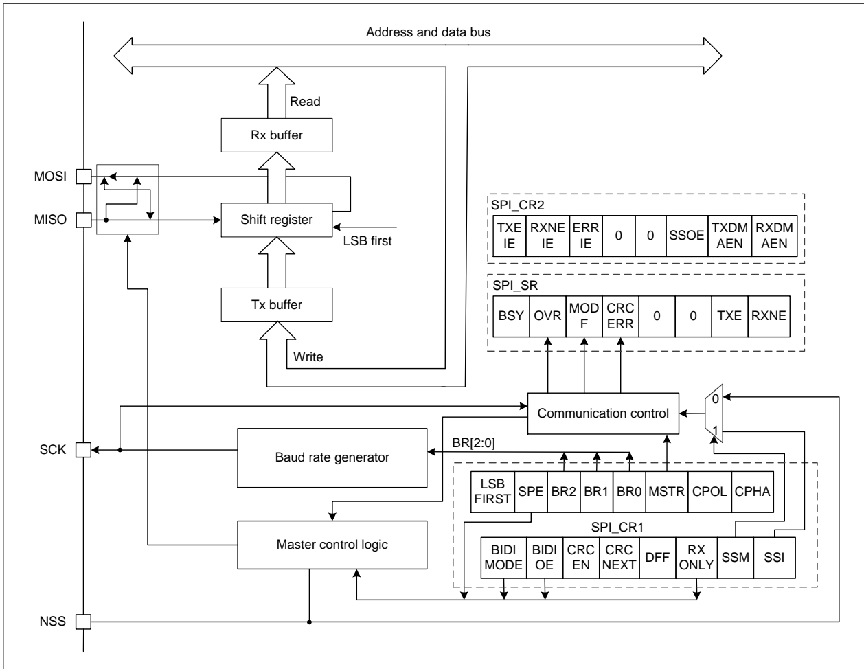
Figure 22-1 SPI block diagram
