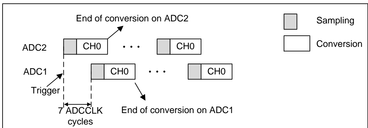
Figure 9-11 Regular simultaneous mode on 16 channels
