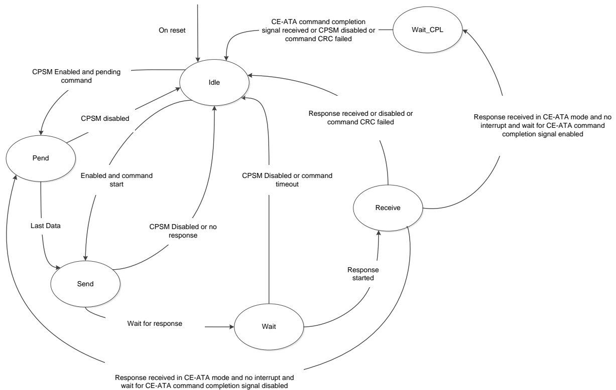
Figure 19-10 Command path state machine (CPSM)
