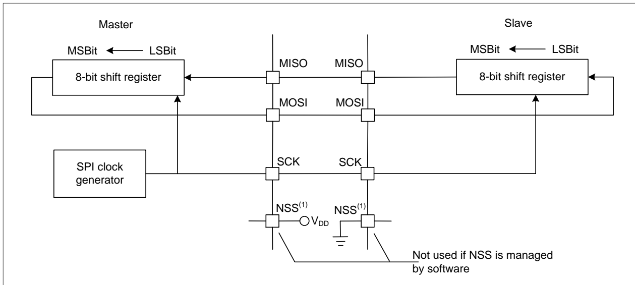
Figure 22-2 Single master/ single slave application
