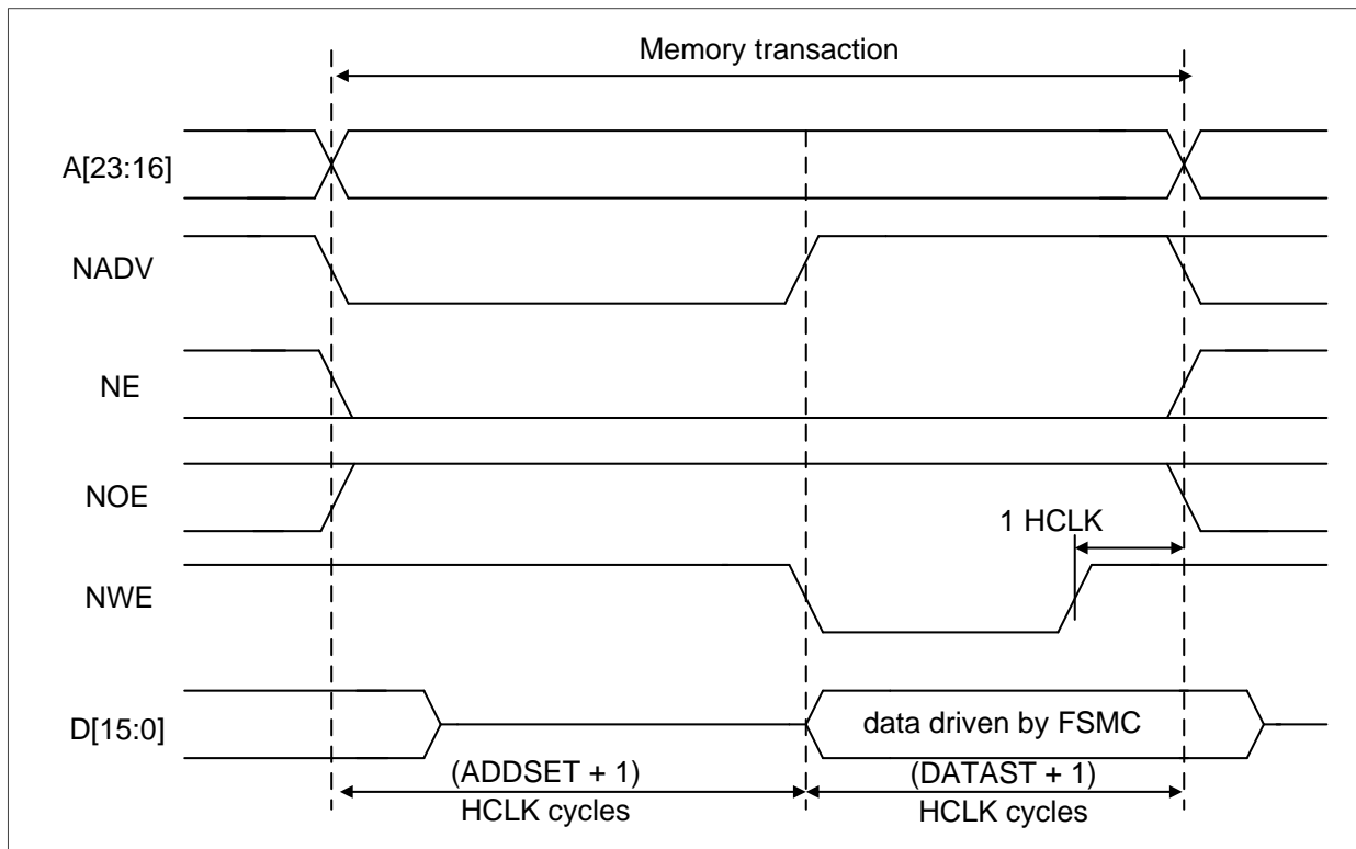
Figure 18-8 Mode2 write accesses
