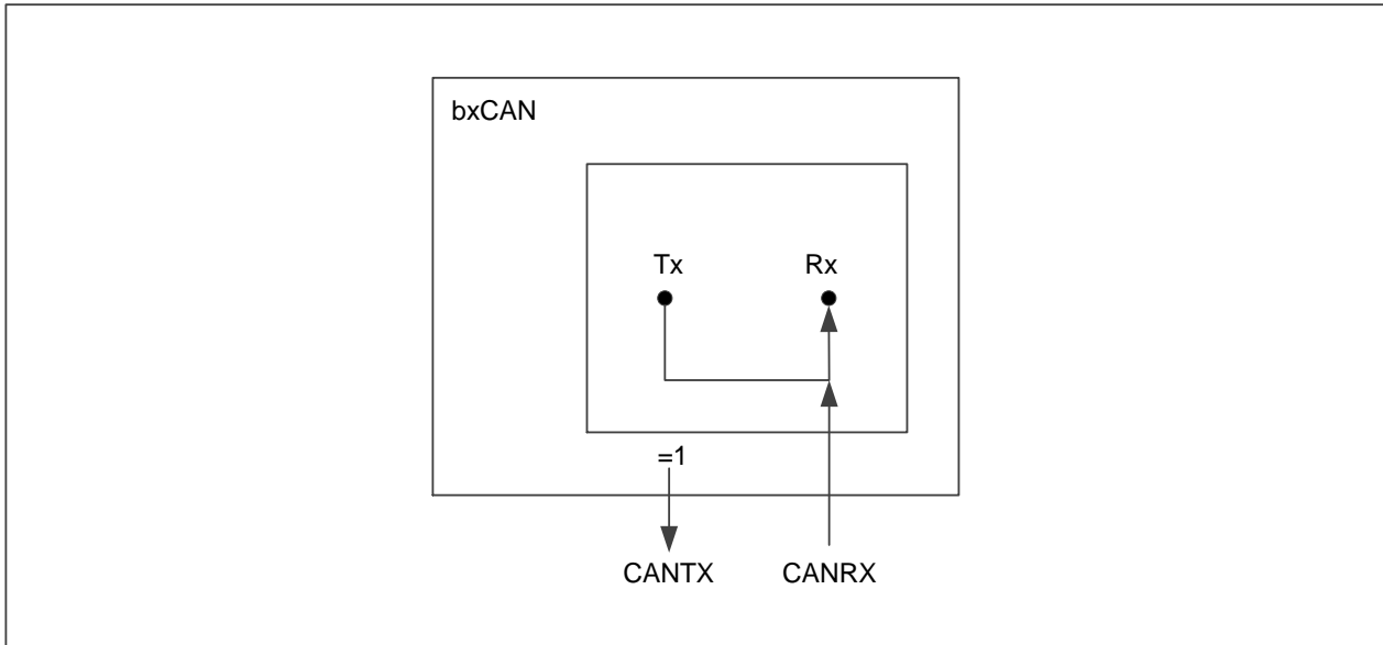
Figure 21-3 bxCAN in silent mode
