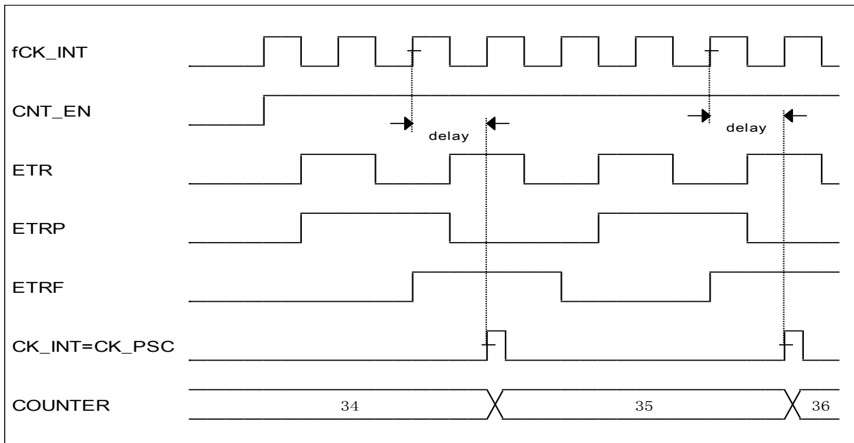
Figure 12-26 Control circuit in external clock mode 2
