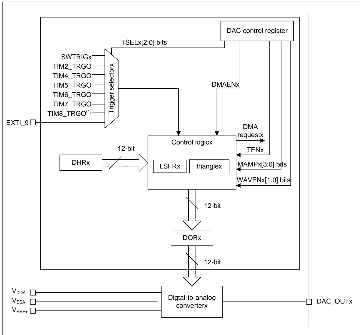
Figure 10-1 DAC channel block diagram
