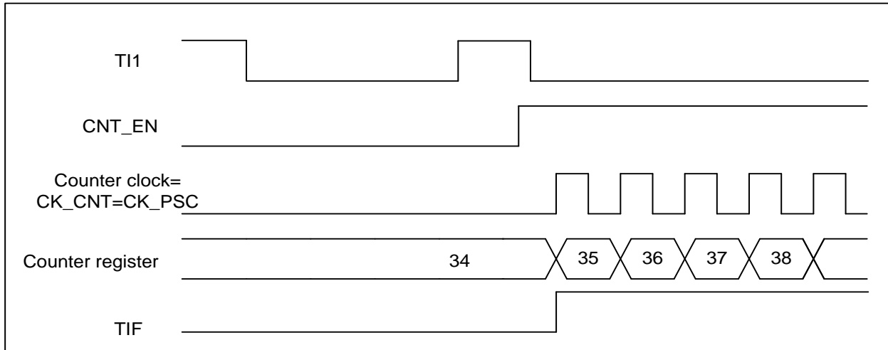
Figure 13-39 Control circuit in trigger mode
