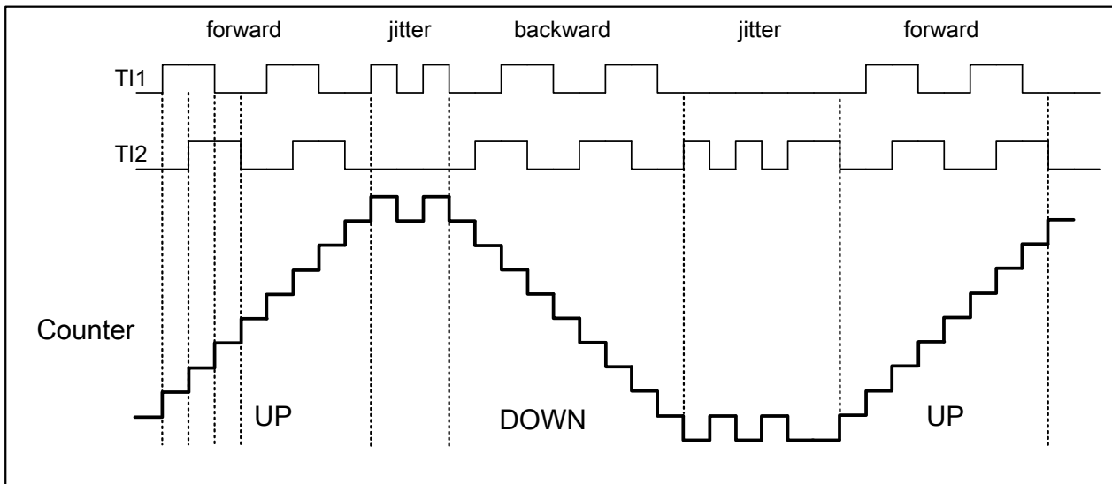
Figure 13-35 Example of counter operation in encoder interface mode.
