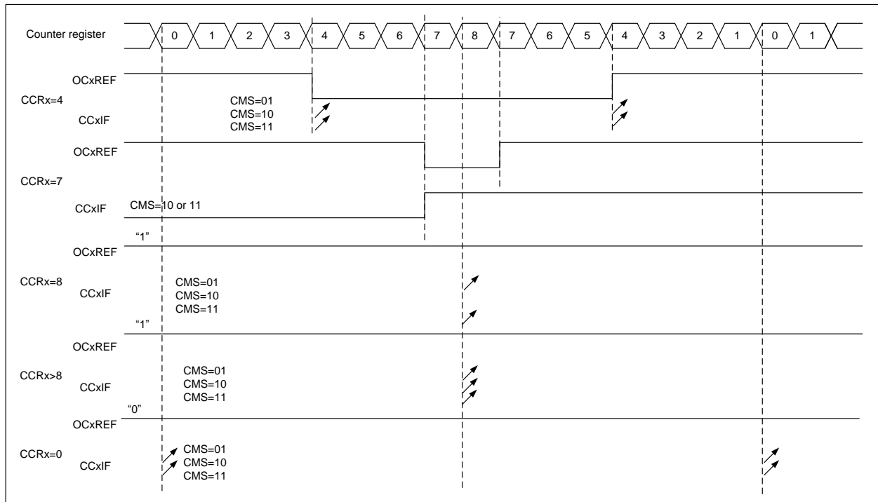
Figure 12-34 Center-aligned PWM waveforms (ARR=8)
