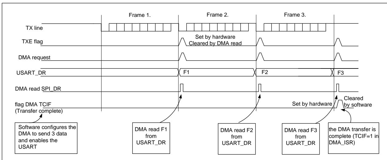
Figure 24-20 Reception using DMA
