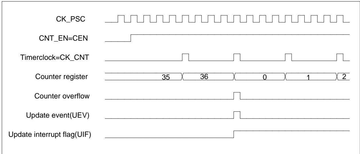
Figure 12-6 Counter timing diagram, internal clock divided by 4
