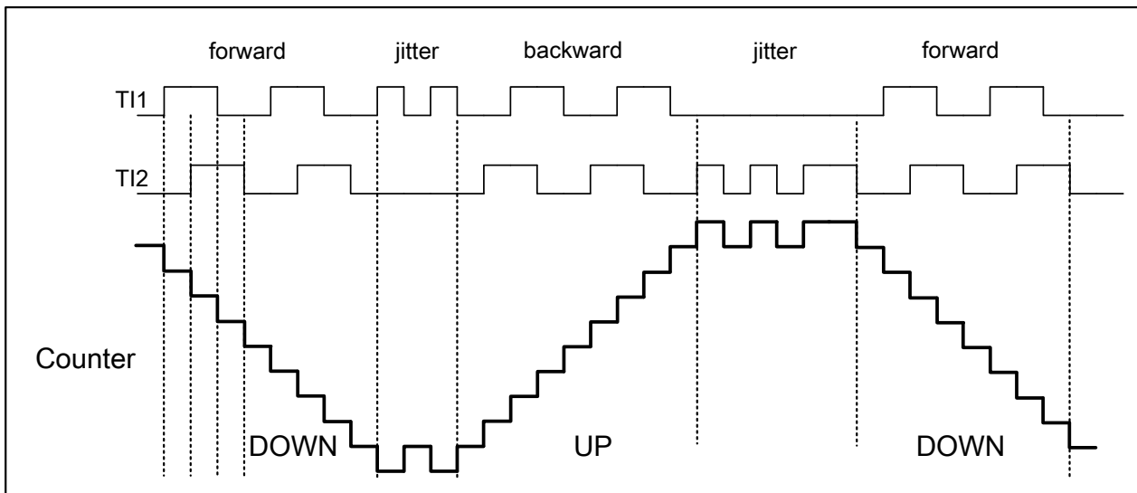
Figure 12-43 Example of encoder interface mode with TI1FP1 polarity inverted
