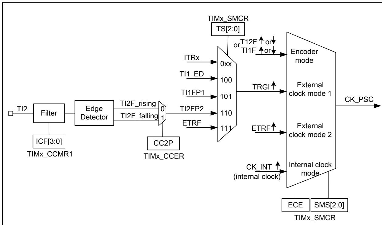
Figure 13-22 TI2 external clock connection example
