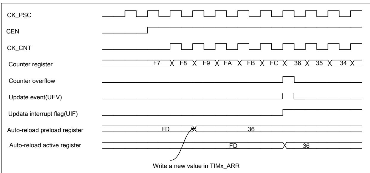
Figure 12-20 Counter timing diagram, Update event with ARPE=1 (counter overflow)
