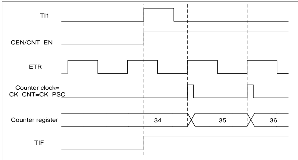
Figure 13-40 Control circuit in external clock mode 2 + trigger mode
