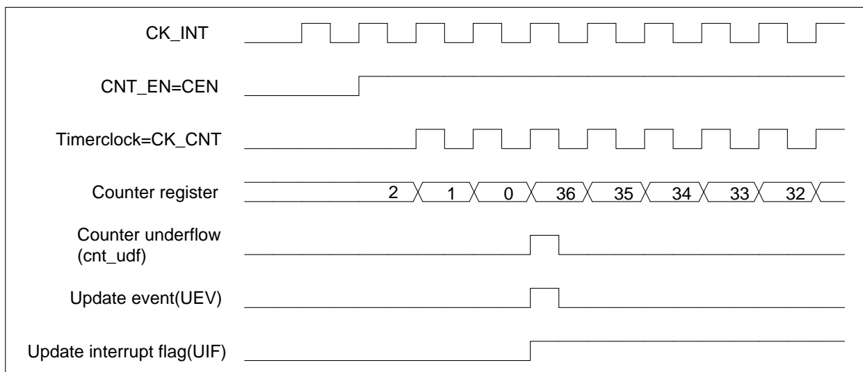
Figure 13-10 Counter timing diagram, internal clock divided by 1
