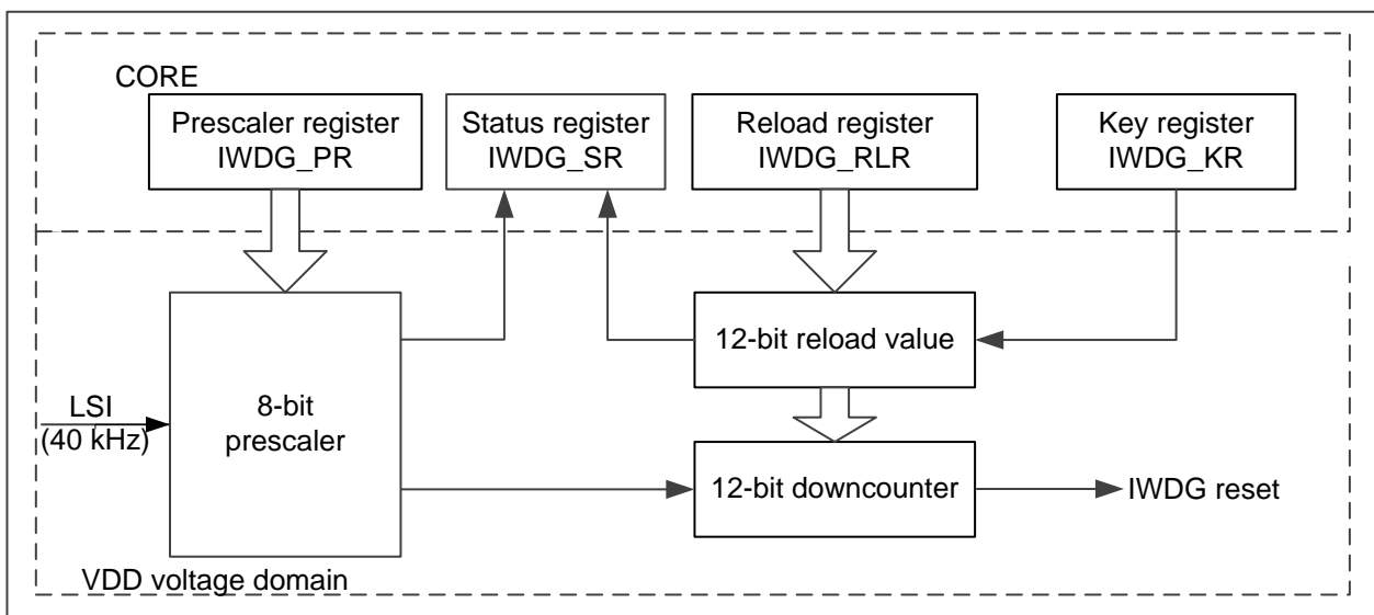
Figure 16-1 Independent watchdog block diagram
