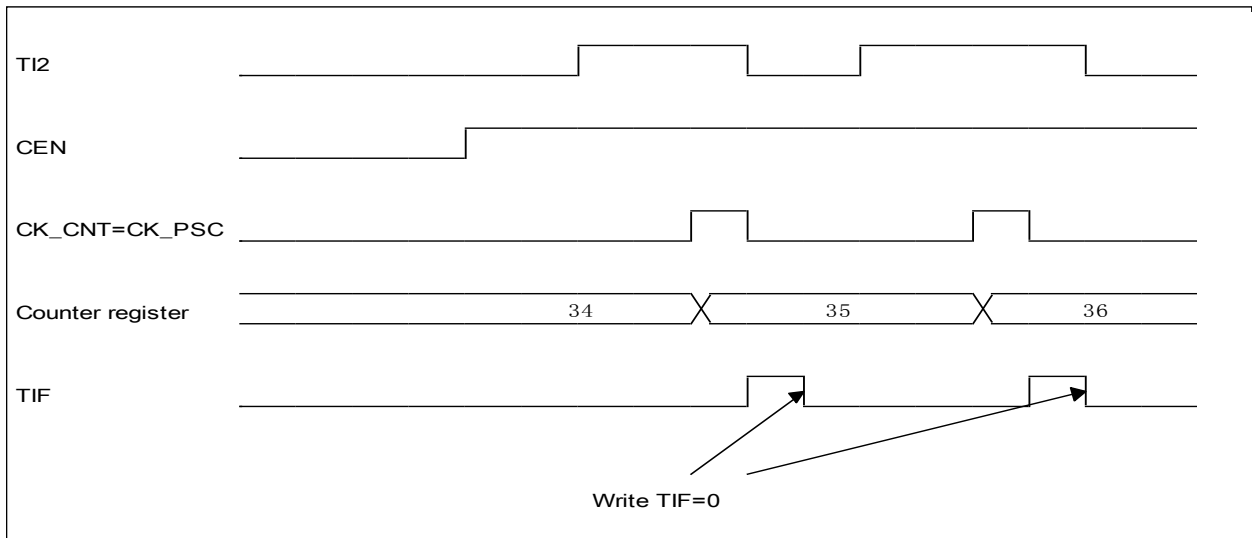
Figure 12-24 Control circuit in external clock mode 1
