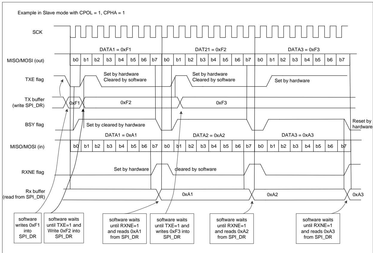
Figure 22-5 TXE/RXNE/BSY behavior in Slave / full-duplex mode (BIDIMODE=0, RXONLY=0) in case of continuous transfers
