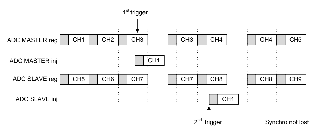
Figure 9-15 Alternate + Regular simultaneous
