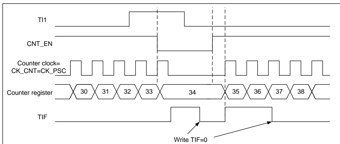
Figure 13-38 Control circuit in gated mode
