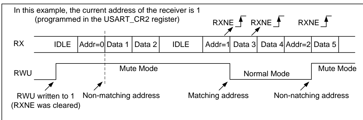
Figure 24-8 Mute mode using address mark detection
