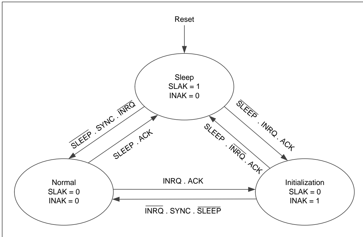
Figure 21-2 bxCAN operating modes
