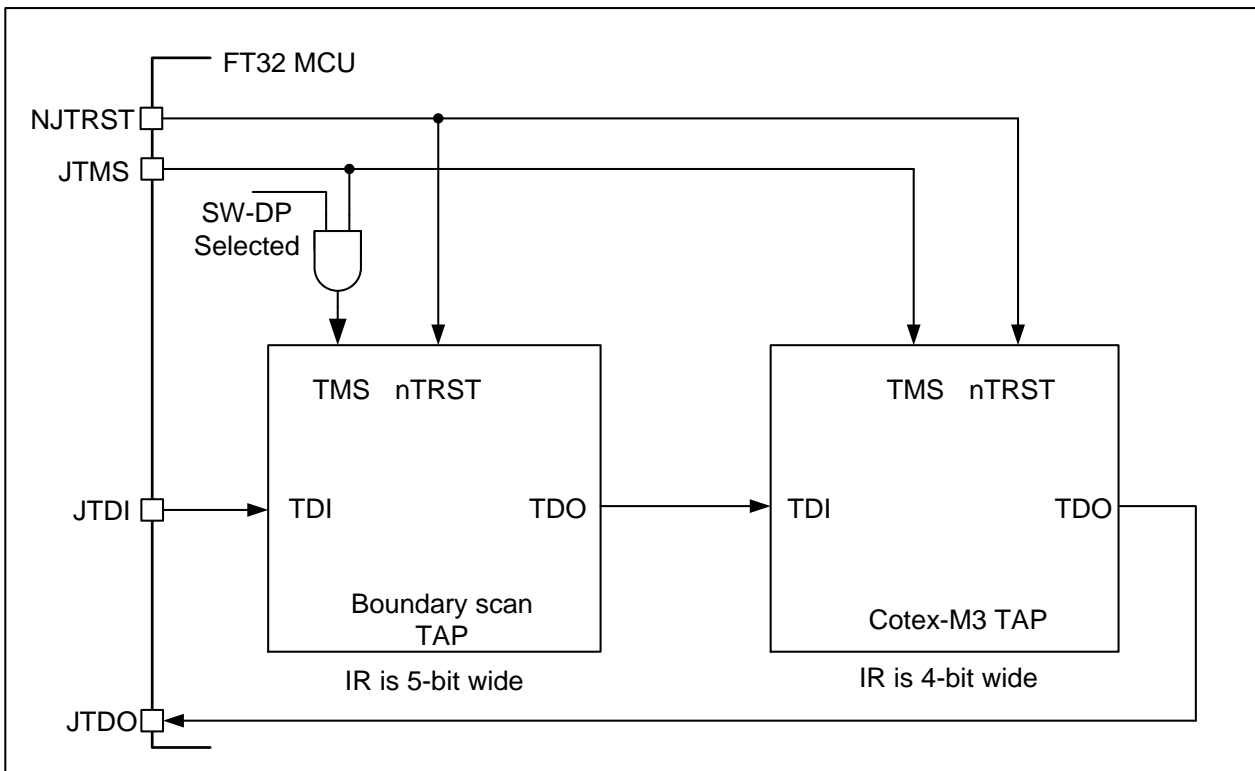
Figure 26-3 JTAG TAP connections
