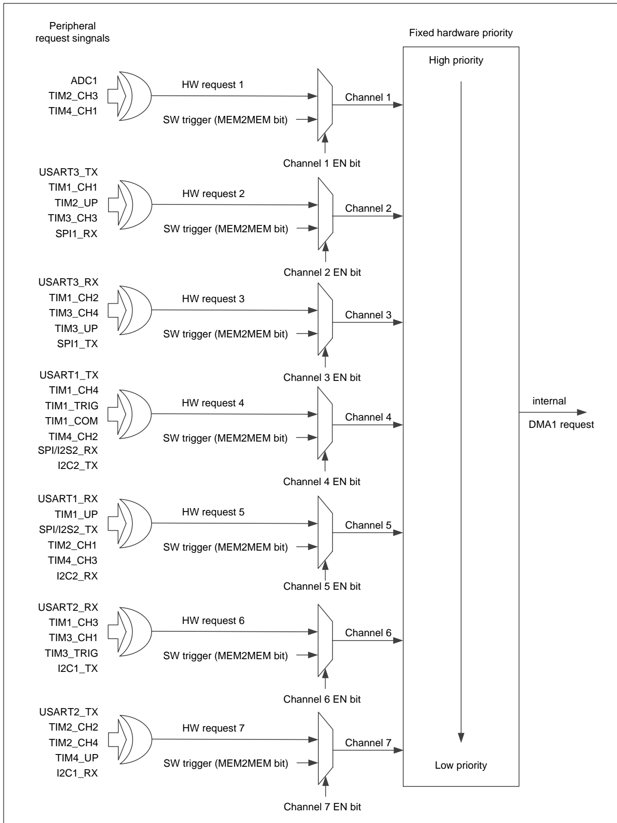
Figure 11-2 DMA1 request mapping
