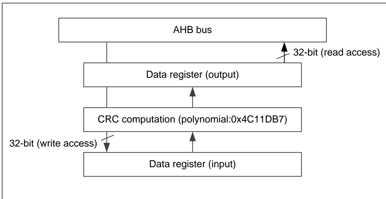
Figure 3-1 CRC calculation unit block diagram
