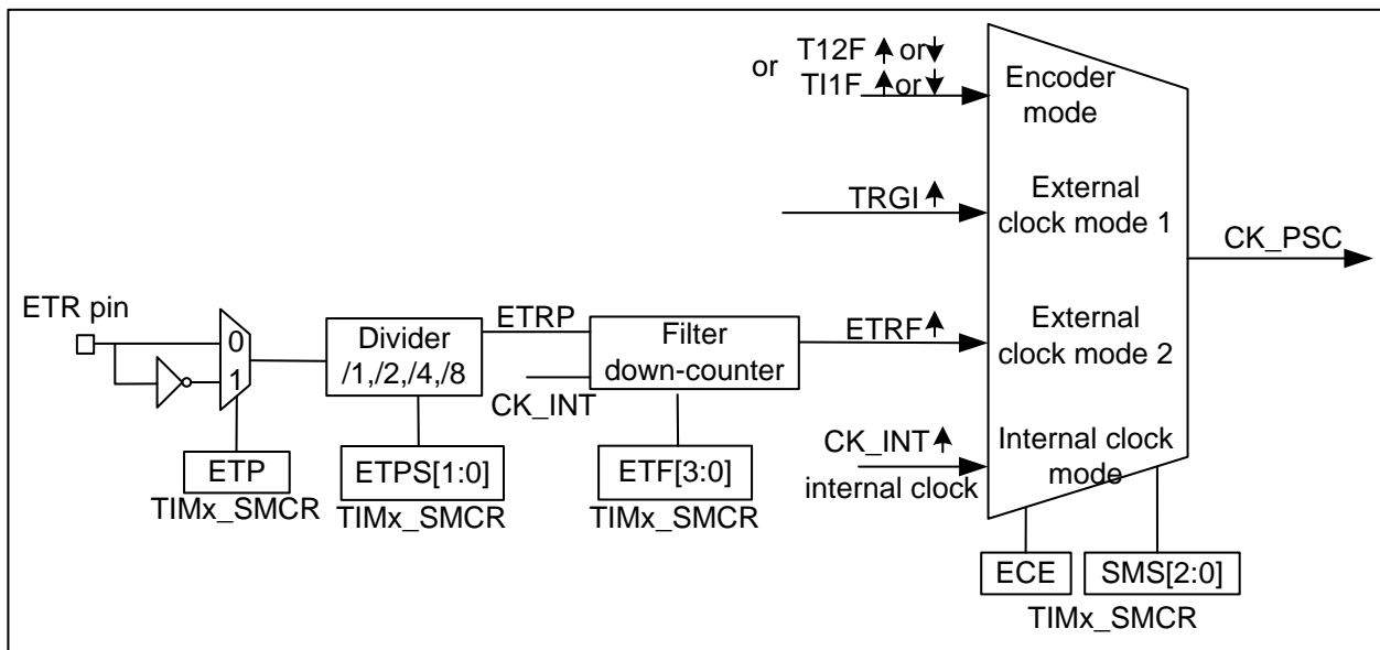
Figure 13-24 External trigger input block
