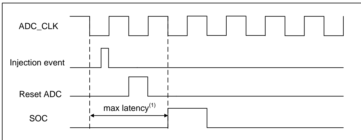
Figure 9-4 Injected conversion latency
