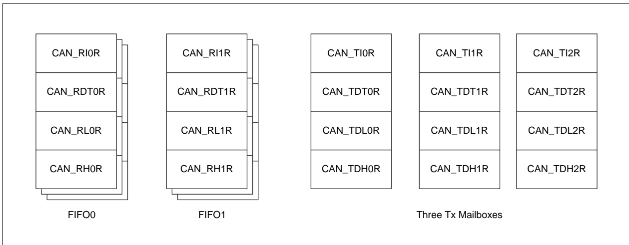
Figure 21-15 RX and TX mailboxes
