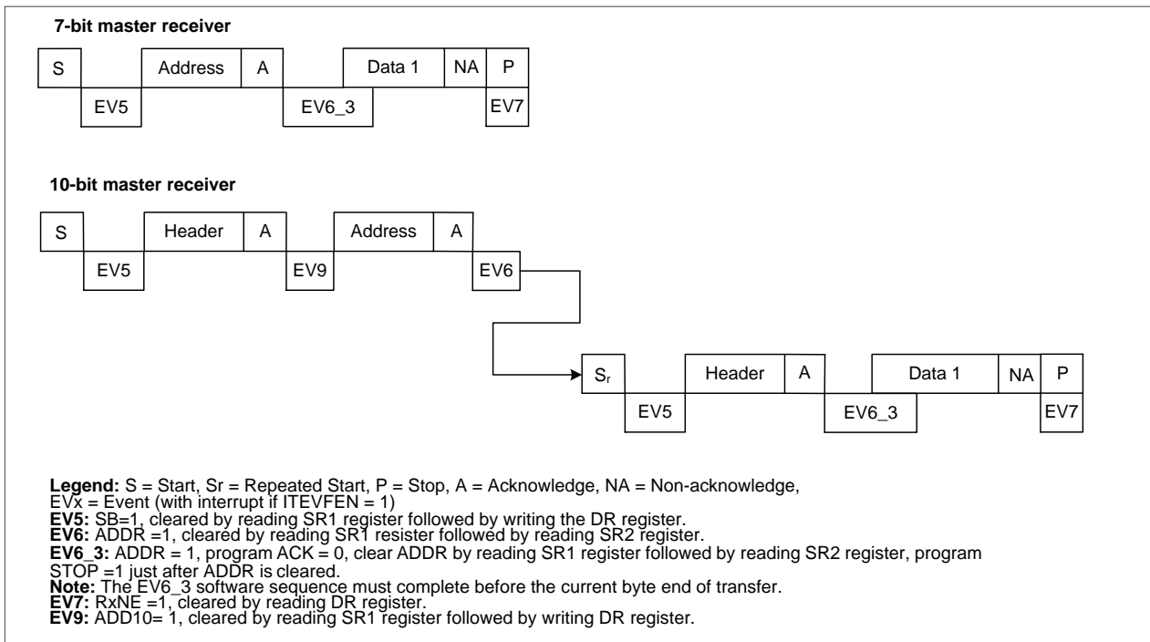
Figure 23-9 Method 2: transfer sequence diagram for master receiver when N=1
