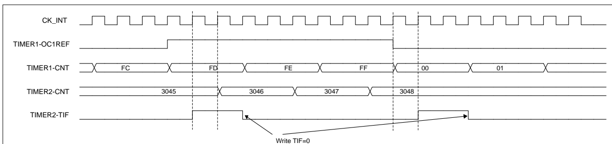
Figure 13-42 Gating timer 2 with OC1REF of timer 1
