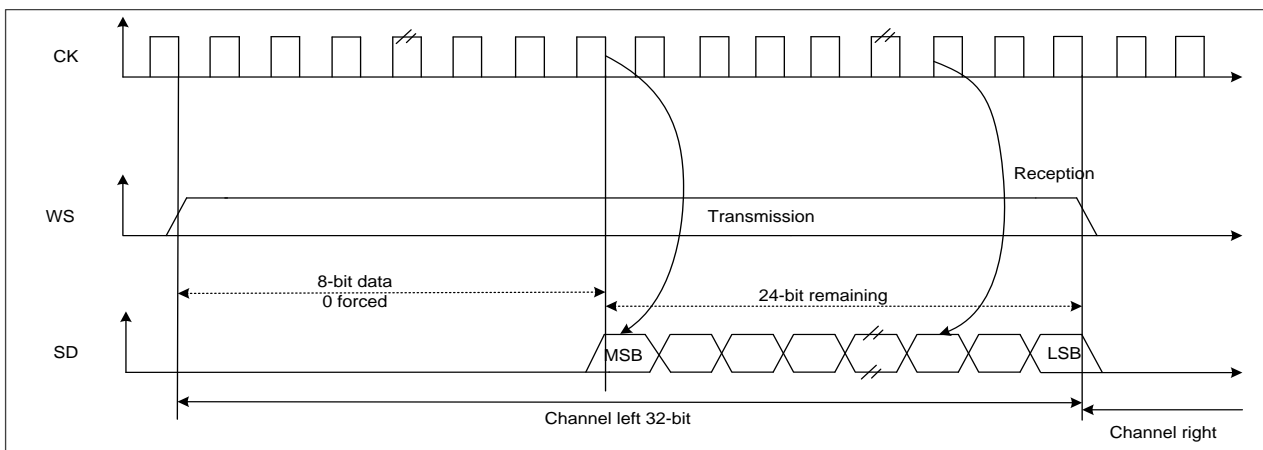
Figure 22-23 LSB justified 24-bit frame length with CPOL = 0
