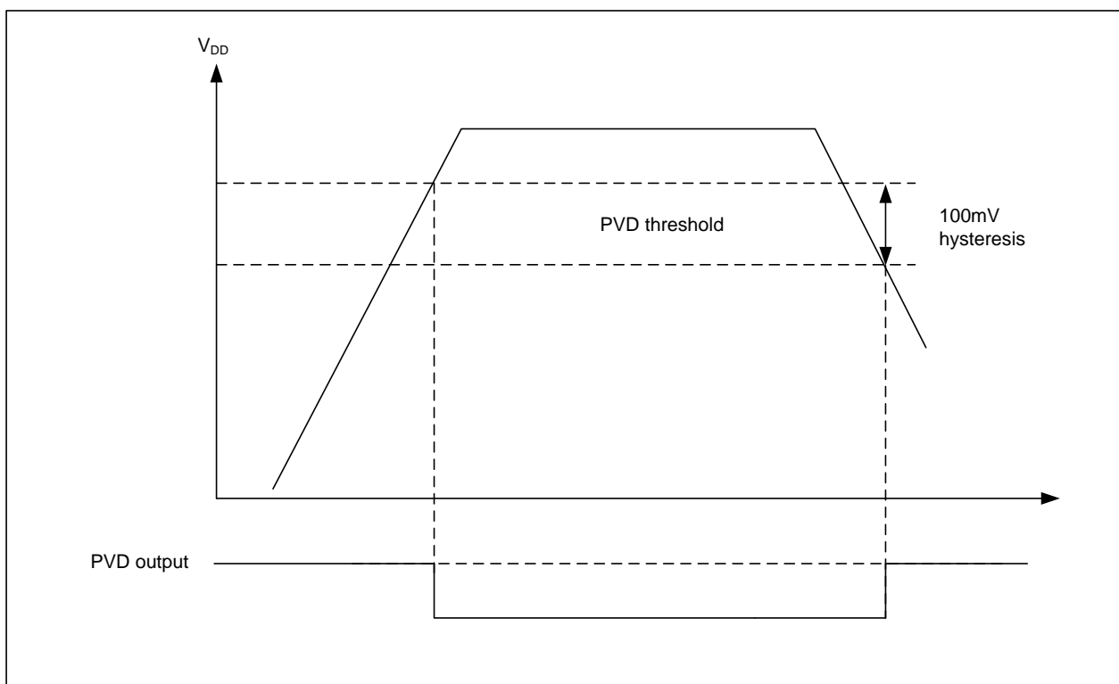
Figure 4-3 PVD thresholds
