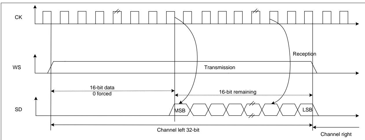
Figure 22-26 LSB justified 16-bit extended to 32-bit packet frame with CPOL = 0
