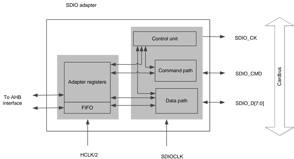
Figure 19-7 SDIO adapter
