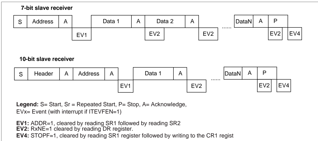
Figure 23-4 Transfer sequence diagram for slave receiver
