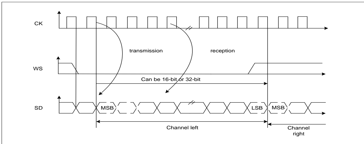
Figure 22-13 I2S Philips protocol waveforms (16/32-bit full accuracy, CPOL = 0)
