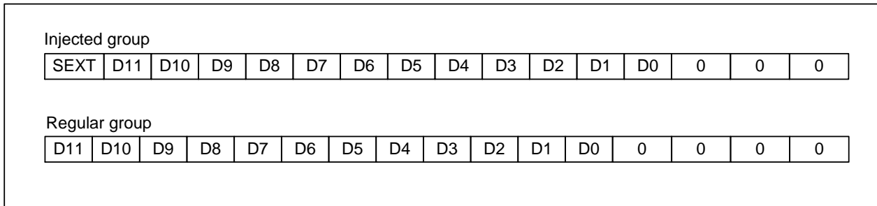
Figure 9-7 Left alignment of data
