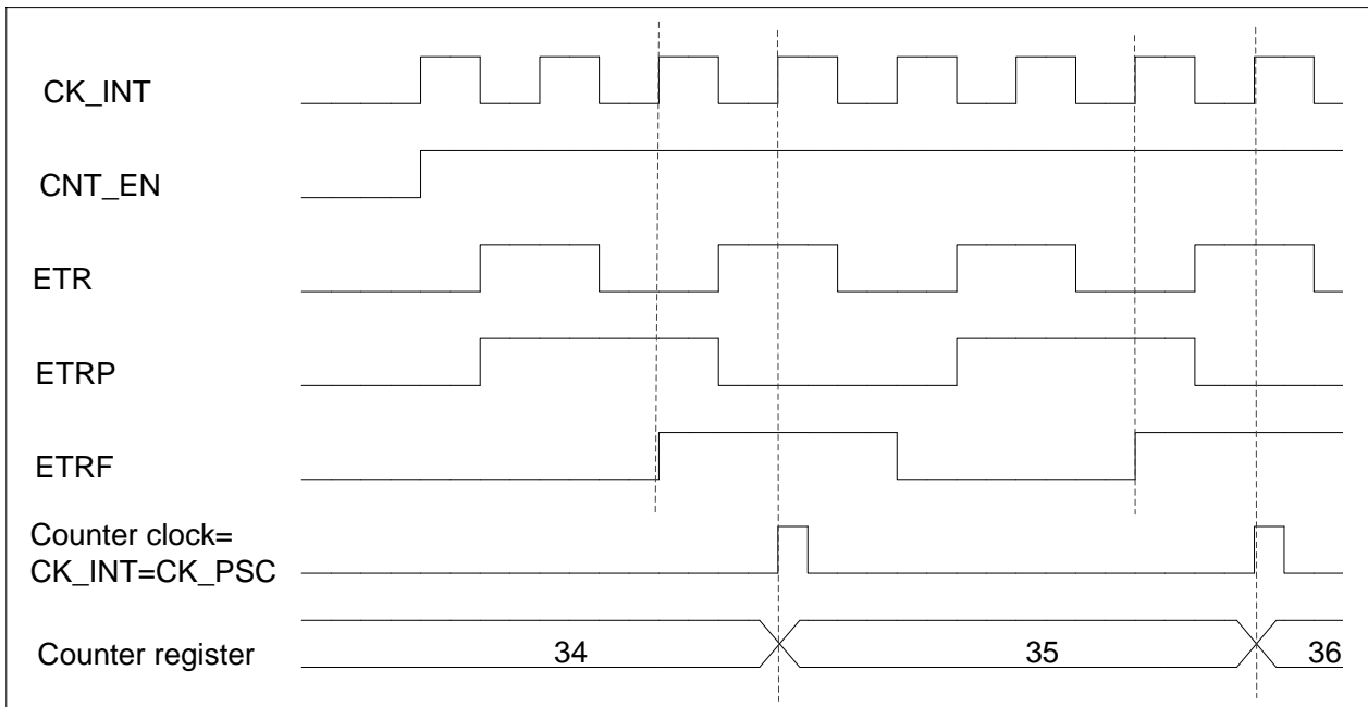
Figure 13-25 Control circuit in external clock mode 2
