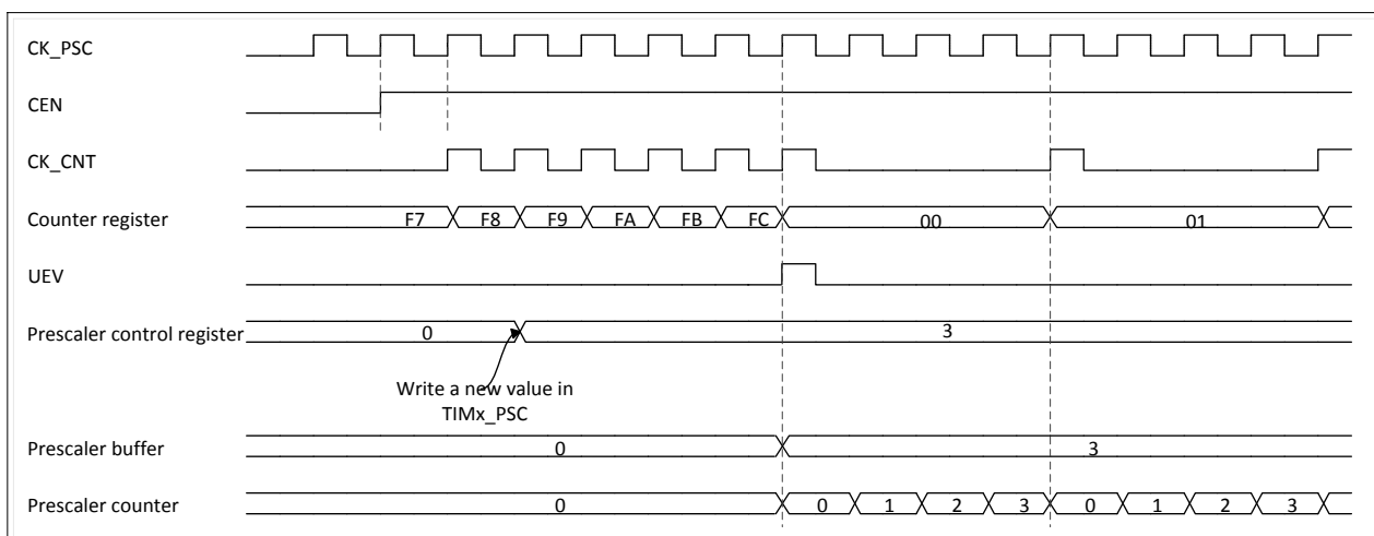
Figure 14-3 Counter timing diagram with prescaler division change from 1 to 4
