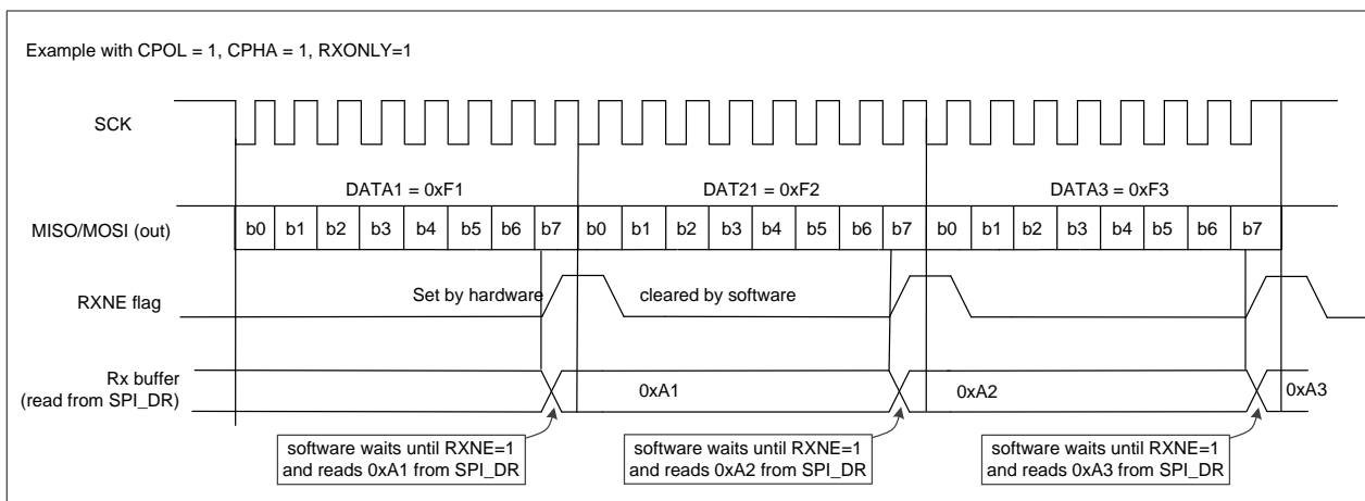
Figure 22-8 RXNE behavior in receive-only mode (BIDIRMODE=0 and RXONLY=1) in case of continuous transfers
