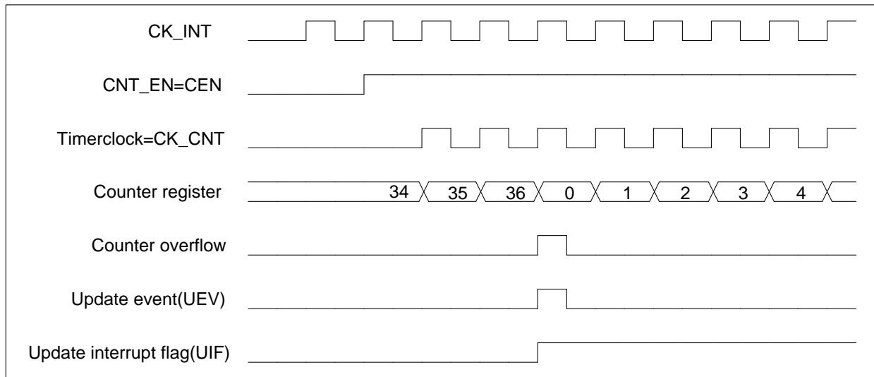
Figure 13-4 Counter timing diagram, internal clock divided by 1
