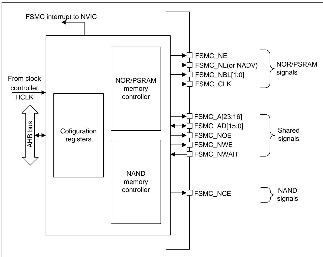
Figure 18-1 FSMC block diagram
