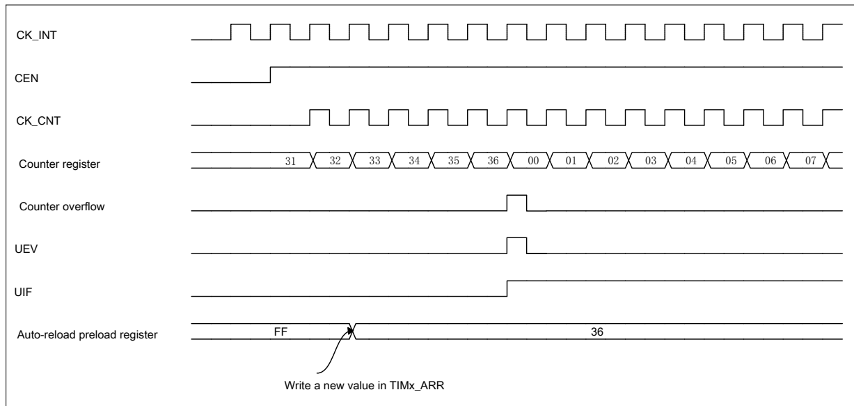
Figure 13-8 Counter timing diagram, update event when ARPE=0(TIMx_ARR not preloaded)
