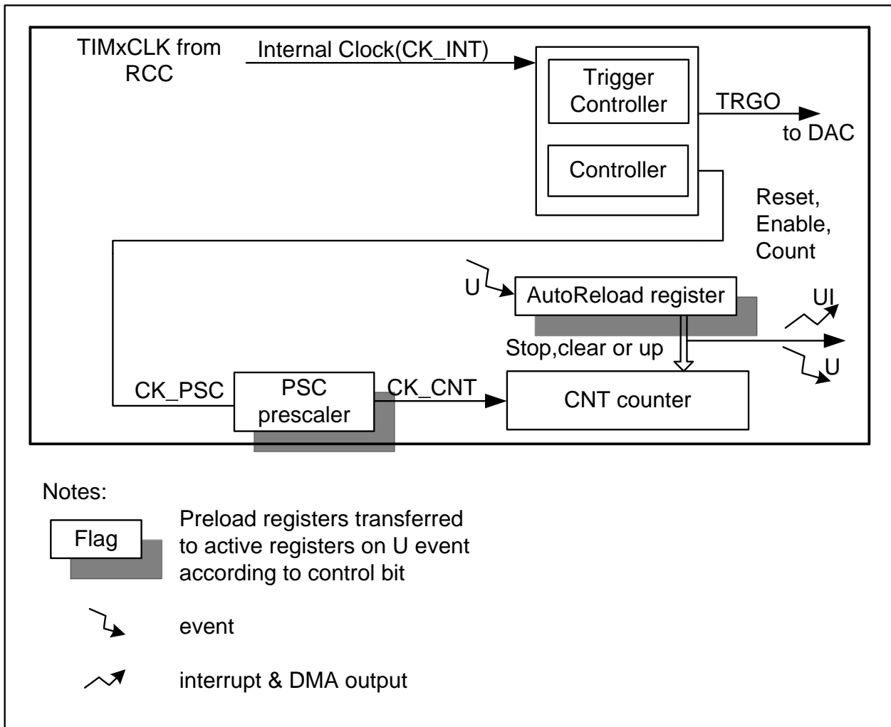
Figure 14-1 Basic timer block diagram
