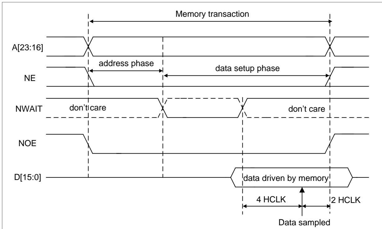
Figure 18-16 Asynchronous wait during a read access
