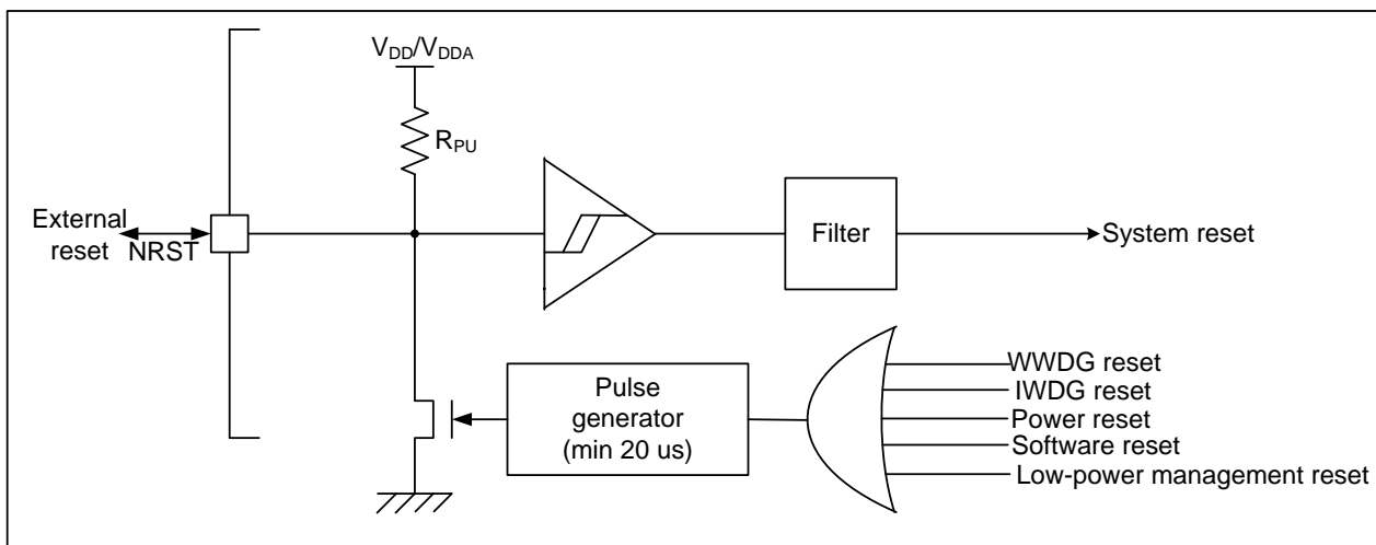
Figure 6-1 Simplified diagram of the reset circuit
