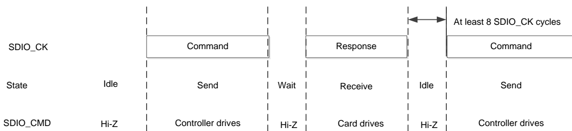
Figure 19-11 SDIO command transfer
