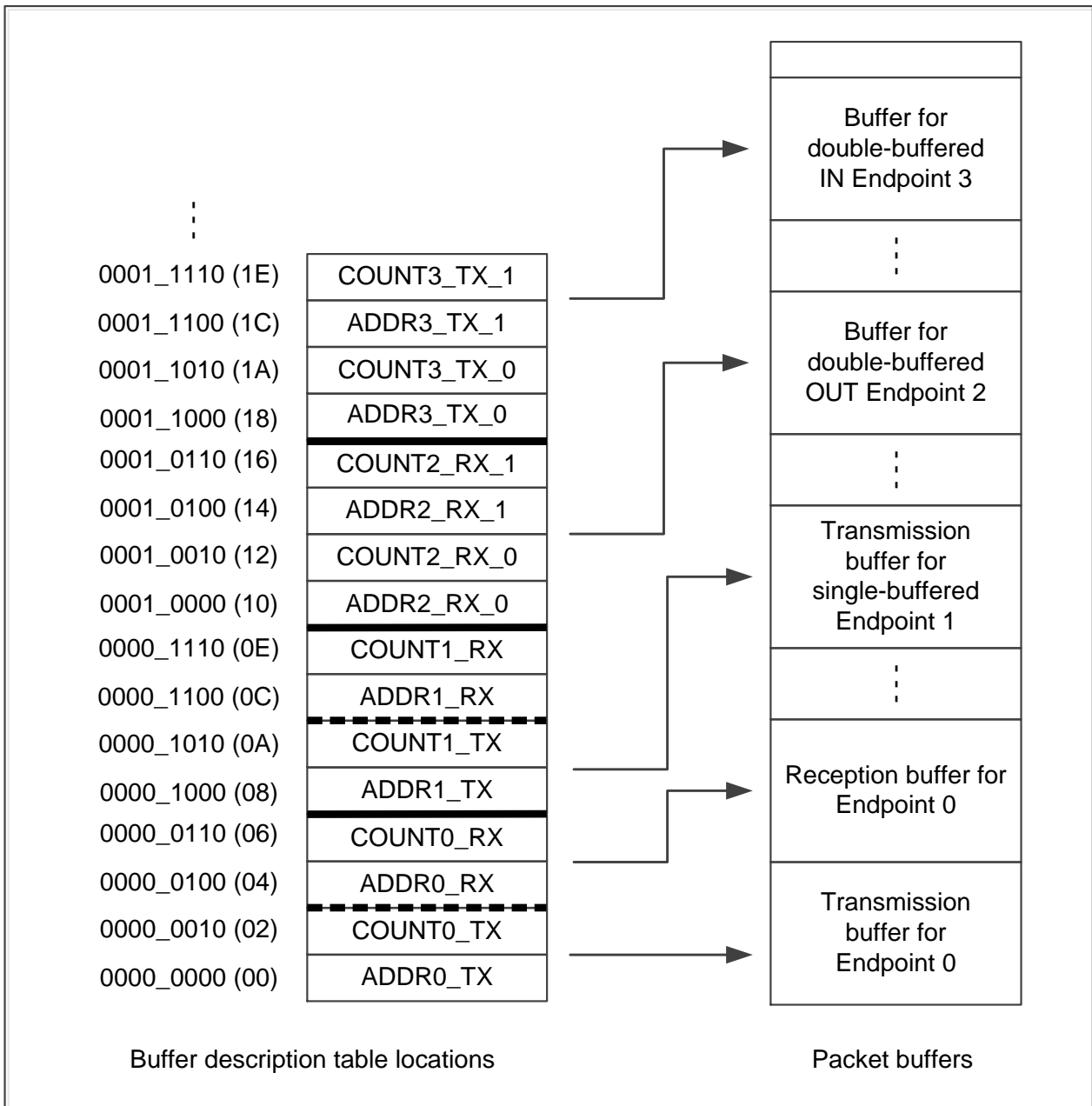
Figure 20-2 Packet buffer areas with examples of buffer description table locations
