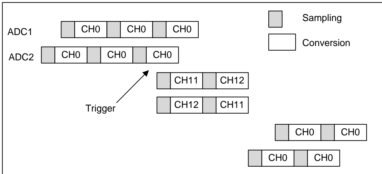
Figure 9-17 Interleaved single channel with injected sequence CH11, CH12
