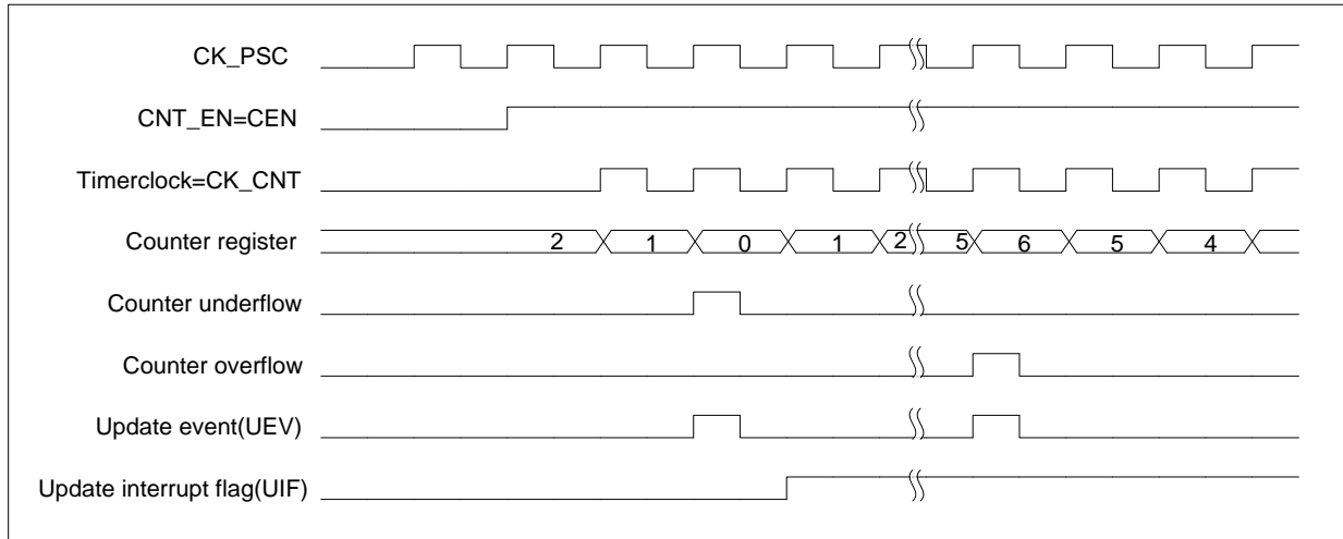
Figure 12-15 Counter timing diagram, internal clock divided by 1, TIMx_ARR = 0x6
