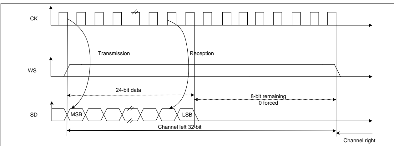
Figure 22-20 MSB justified 24-bit frame length with CPOL = 0
