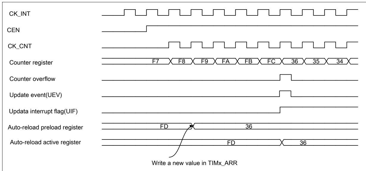
Figure 13-20 Counter timing diagram, Update event with ARPE=1 (counter overflow)
