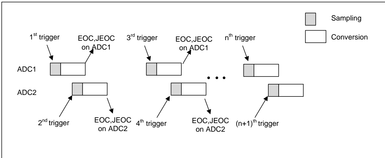
Figure 9-13 Alternate trigger: injected channel group of each ADC
