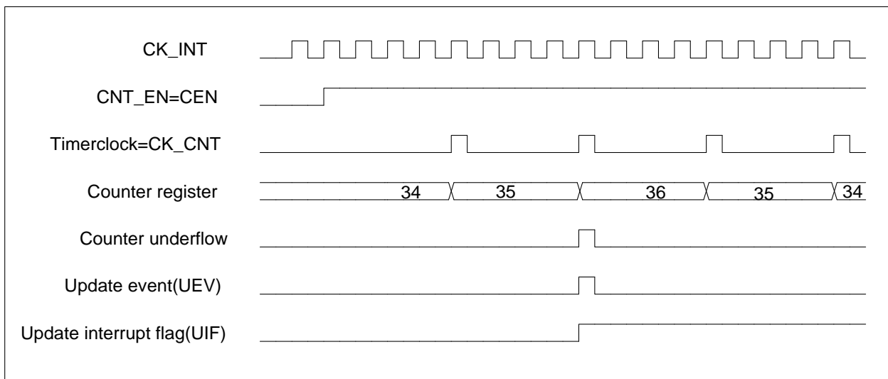
Figure 13-17 Counter timing diagram, internal clock divided by 4, TIMx_ARR=0x36
