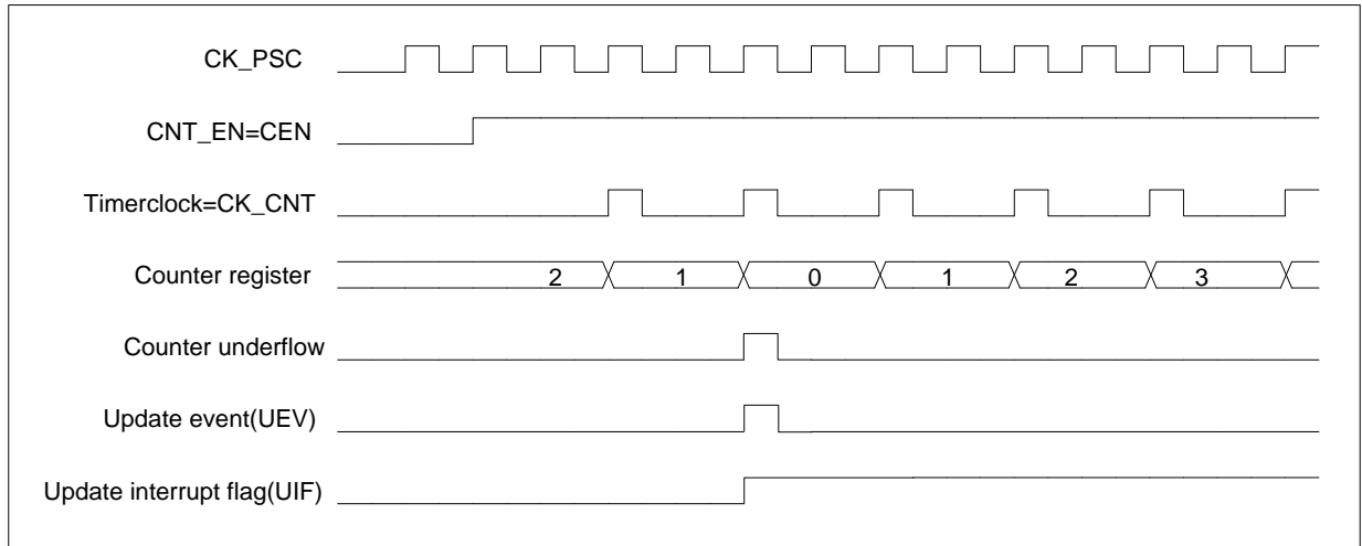
Figure 12-16 Counter timing diagram, internal clock divided by 2
