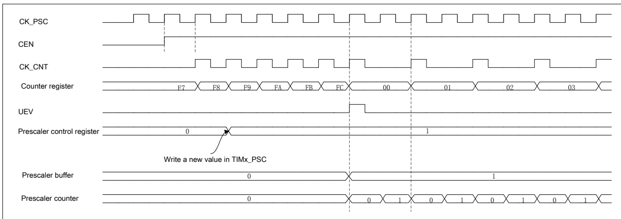
Figure 14-2 Counter timing diagram with prescaler division change from 1 to 2
