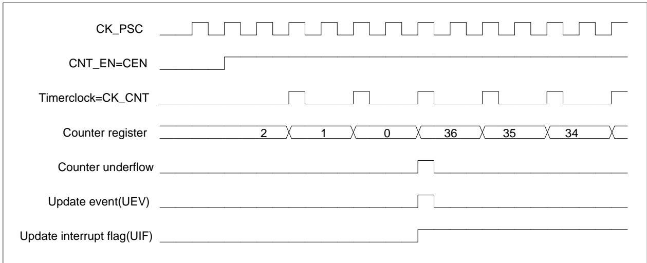
Figure 12-11 Counter timing diagram, internal clock divided by 2
