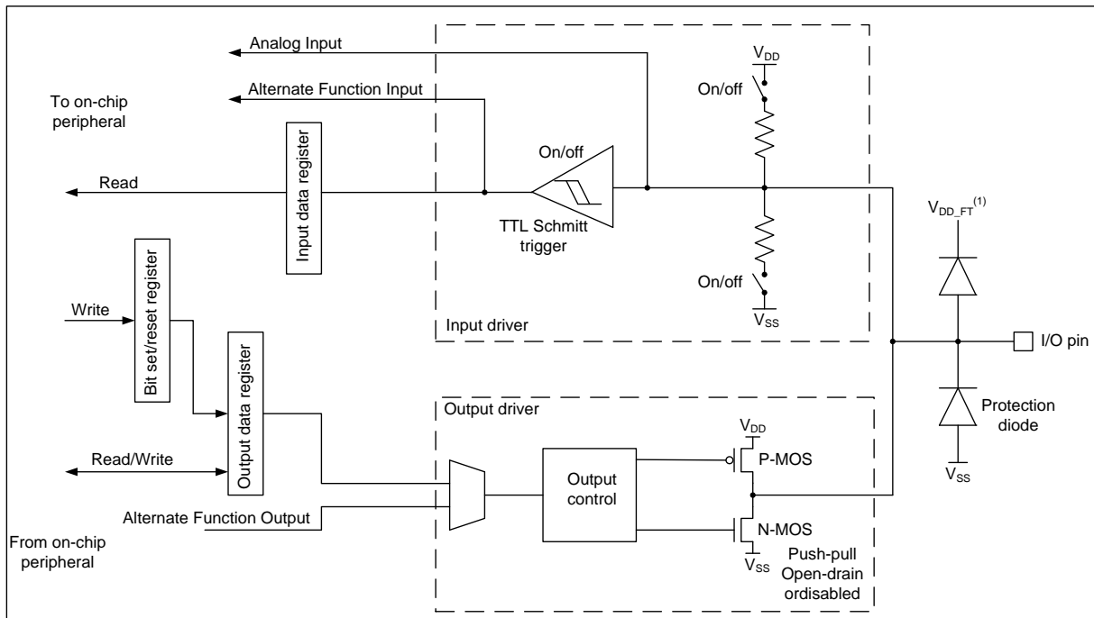
Figure 7-2 Basic structure of a 5-Volt tolerant I/O port bit
