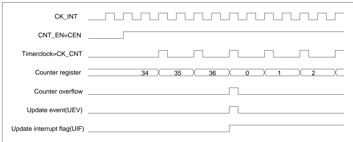
Figure 13-5 Counter timing diagram, internal clock divided by 2
