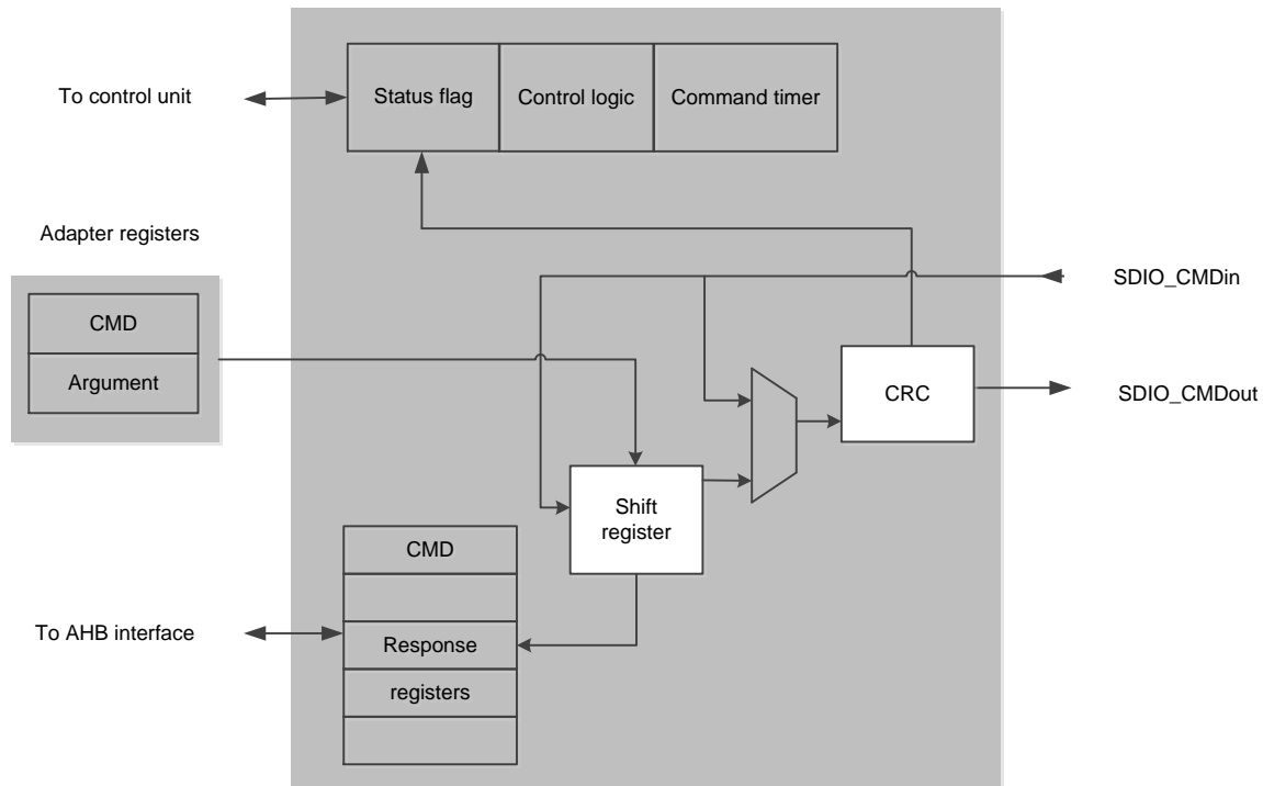
Figure 19-9 SDIO adapter command path
