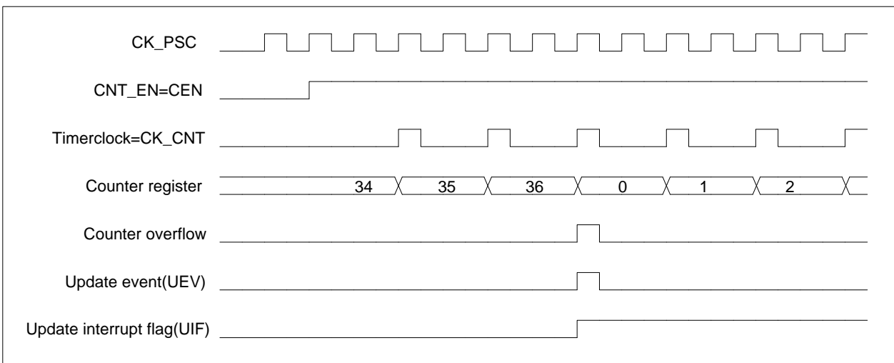
Figure 12-5 Counter timing diagram, internal clock divided by 2
