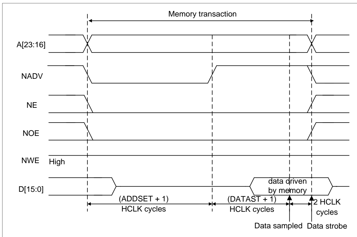
Figure 18-7 Mode2 and mode B read accesses
