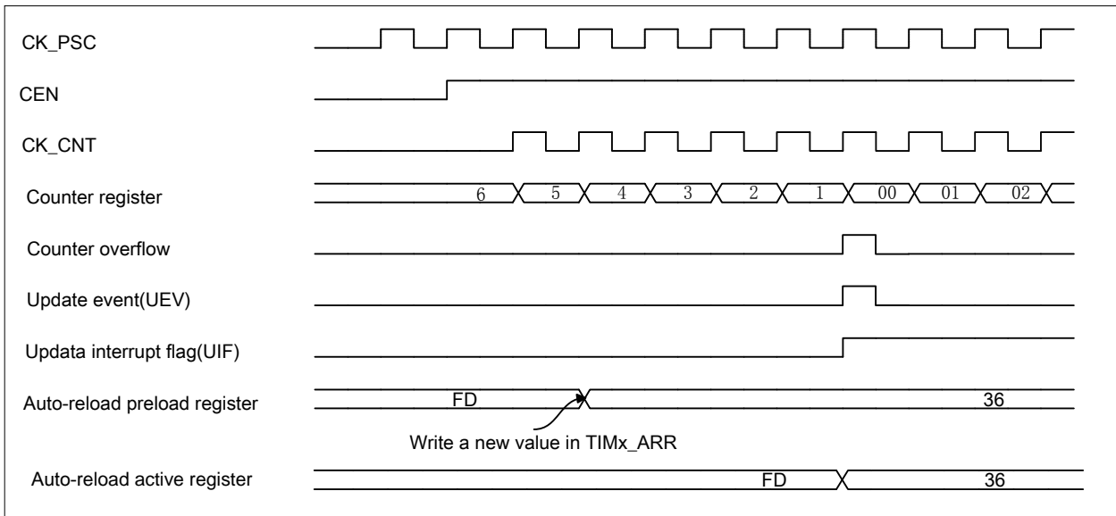
Figure 12-19 Counter timing diagram, update event with ARPE=1 (counter underflow)
