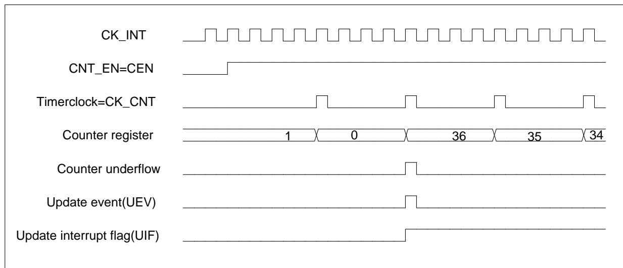
Figure 13-12 Counter timing diagram, internal clock divided by 4
