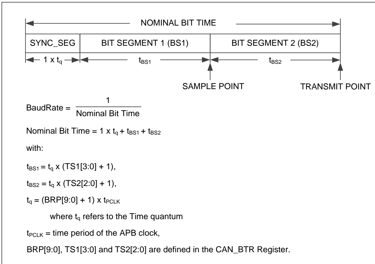
Figure 21-12 Bit timing
