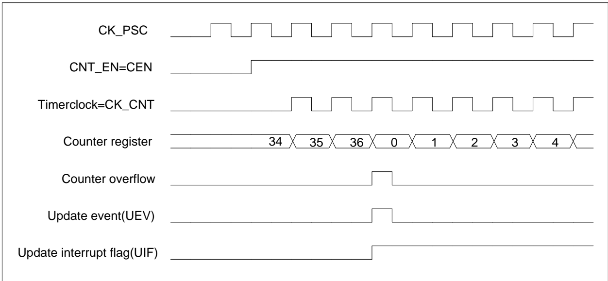
Figure 12-5 Counter timing diagram, internal clock divided by 2
