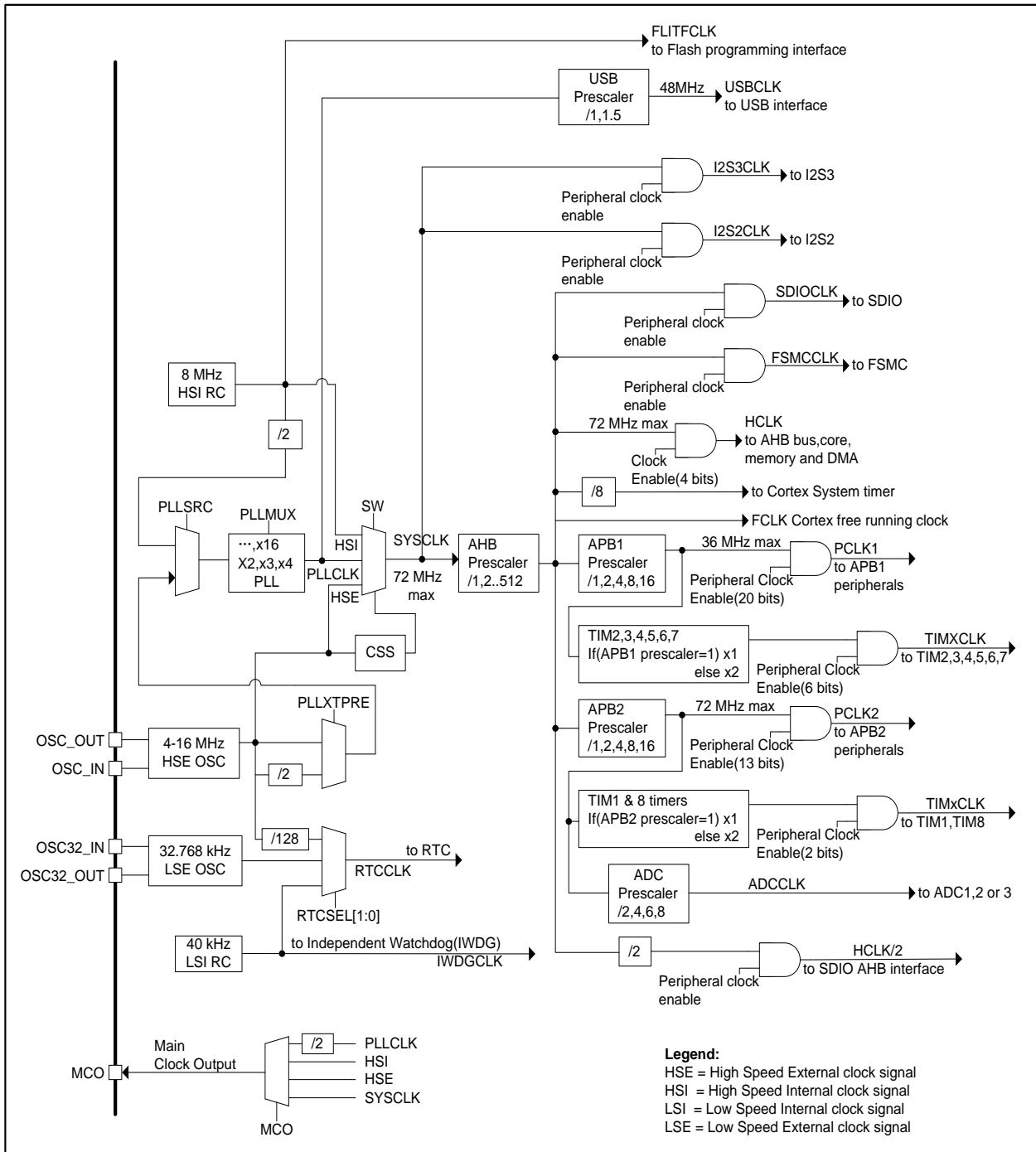
Figure 6-2 Clock tree
