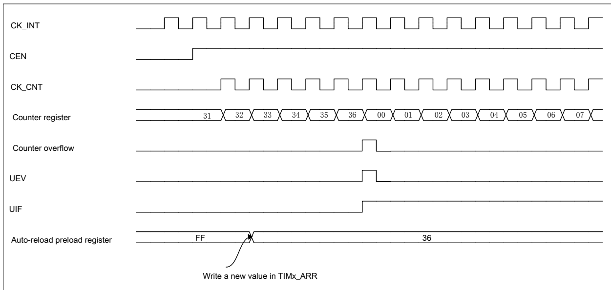
Figure 14-8 Counter timing diagram, update event when ARPE=0(TIMx_ARR not preloaded)
