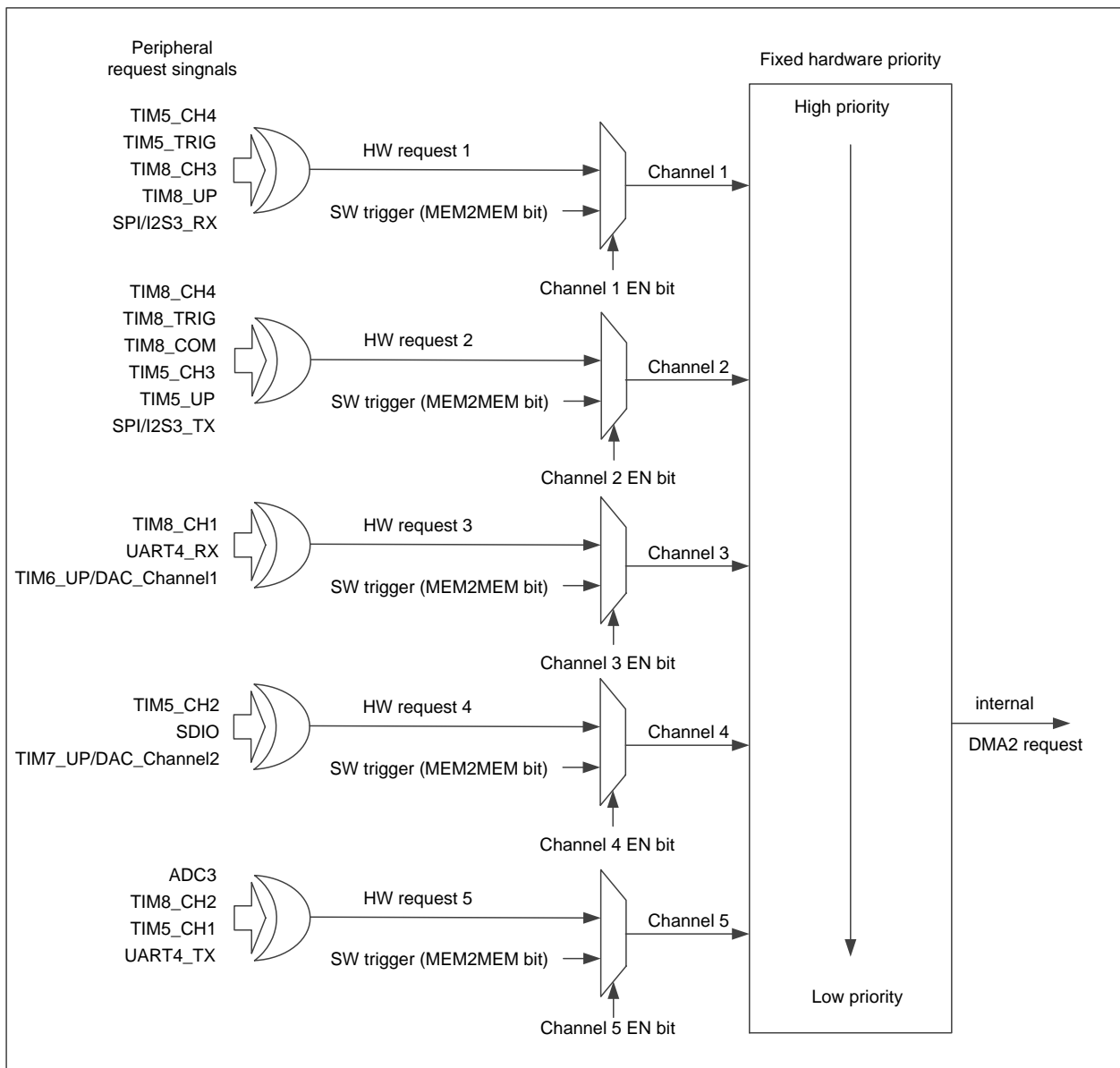
Figure 11-3 DMA2 request mapping
