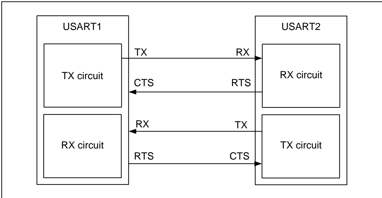
Figure 24-21 Hardware flow control between two USARTs
