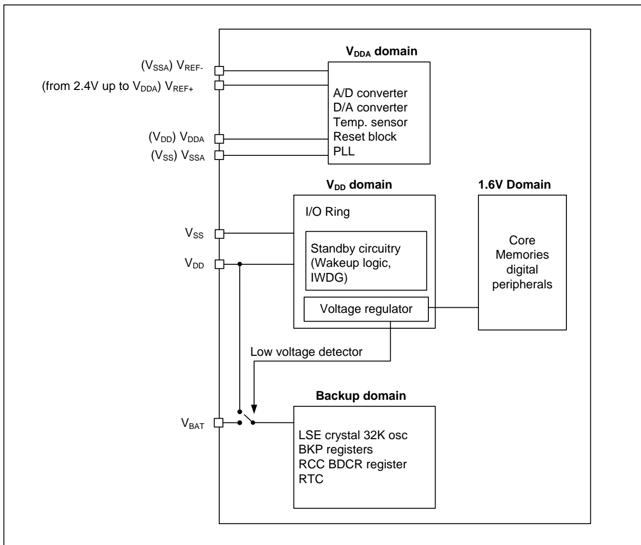
Figure 4-1 Power supply overview
