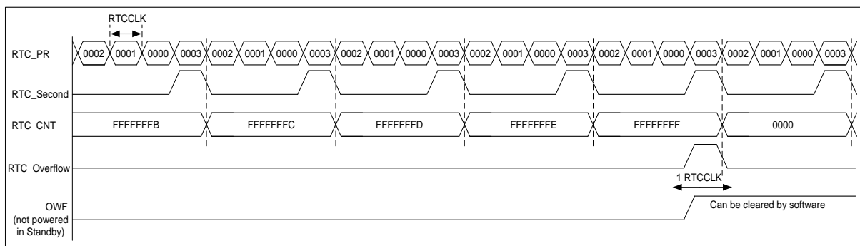
Figure 15-3 RTC Overflow waveform example with PR=0003
