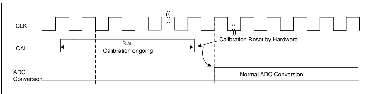
Figure 9-5 Calibration timing diagram
