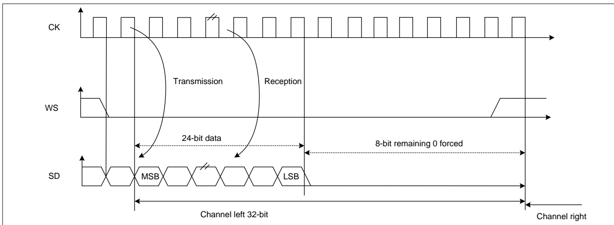
Figure 22-14 I2S Philips standard waveforms (24-bit frame with CPOL = 0)
