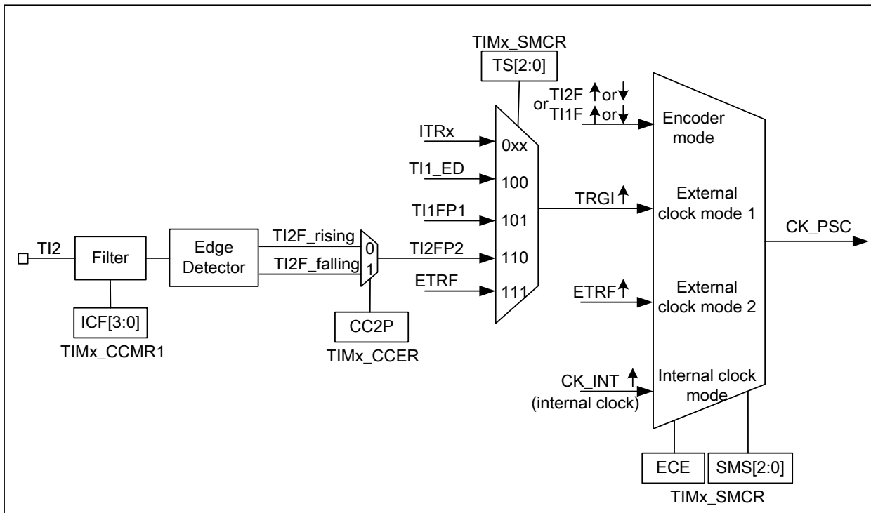
Figure 12-23 TI2 external clock connection example
