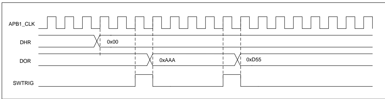
Figure 10-6 DAC conversion (SW trigger enabled) with LFSR wave generation
