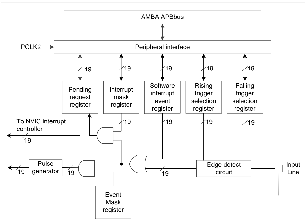
Figure 8-1 External interrupt/event controller block diagram
