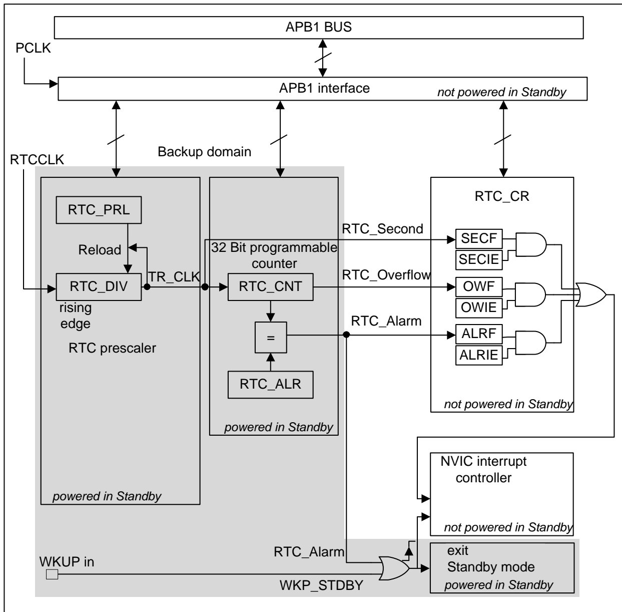
Figure 15-1 RTC simplified block diagram
