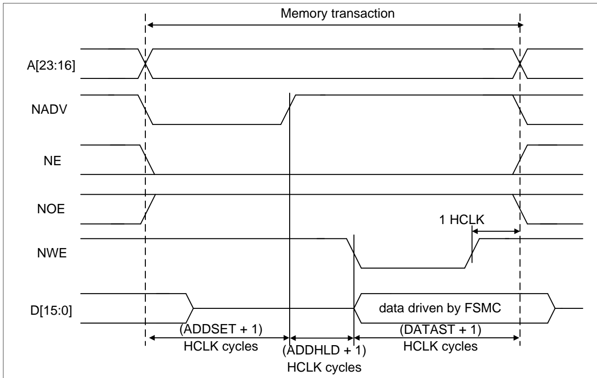
Figure 18-13 Mode D write accesses
