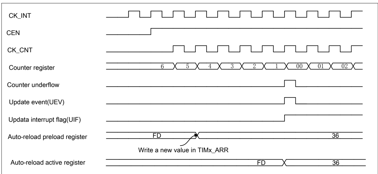
Figure 13-19 Counter timing diagram, update event with ARPE=1 (counter underflow)
