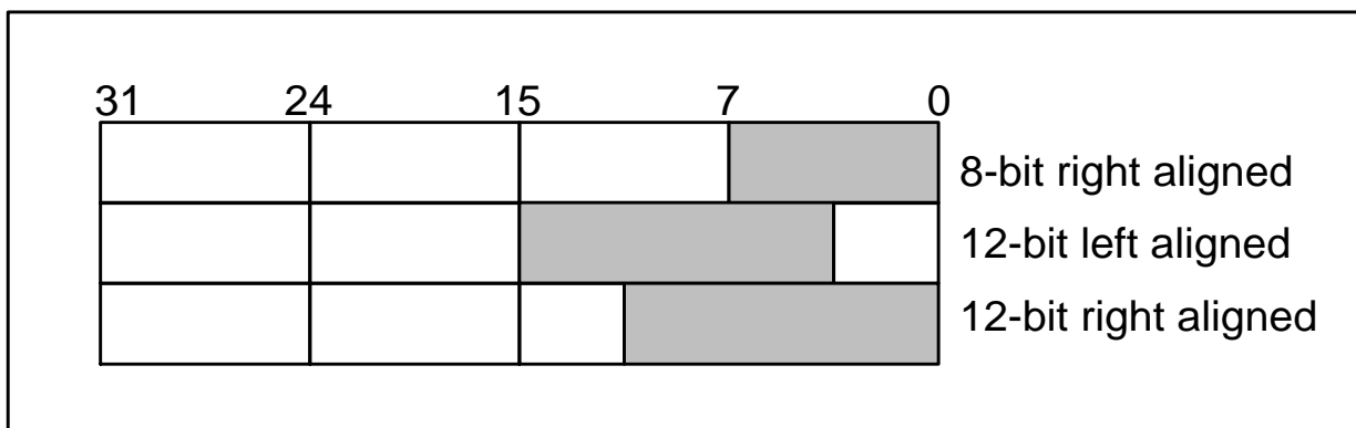
Figure 10-2 Data registers in single DAC channel mode
