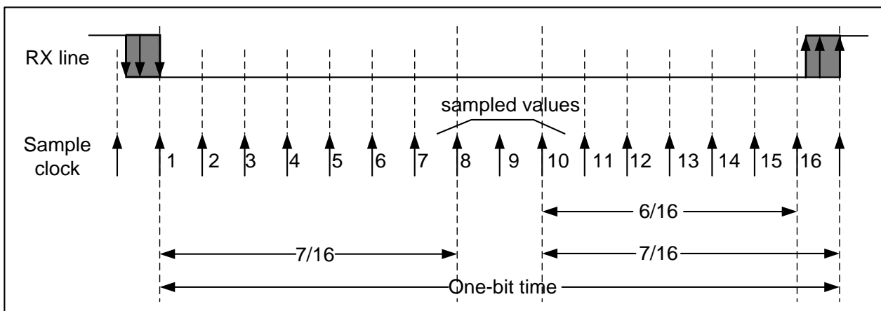
Figure 24-6 Data sampling for noise detection
