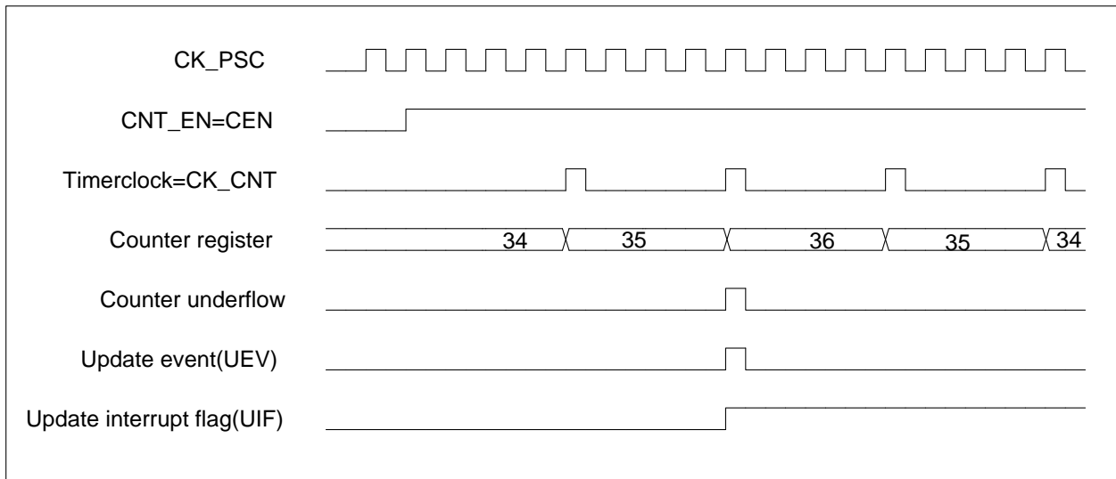
Figure 12-17 Counter timing diagram, internal clock divided by 4, TIMx_ARR=0x36
