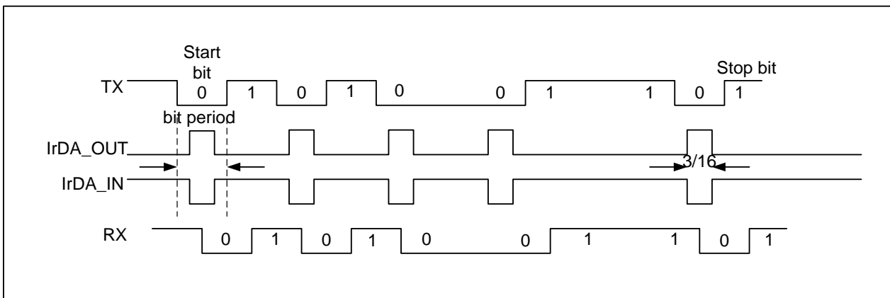
Figure 24-18 IrDA data modulation (3/16) -normal mode
