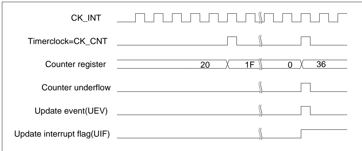
Figure 13-13 Counter timing diagram, internal clock divided by N
