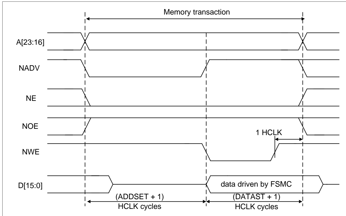
Figure 18-11 Mode C write accesses
