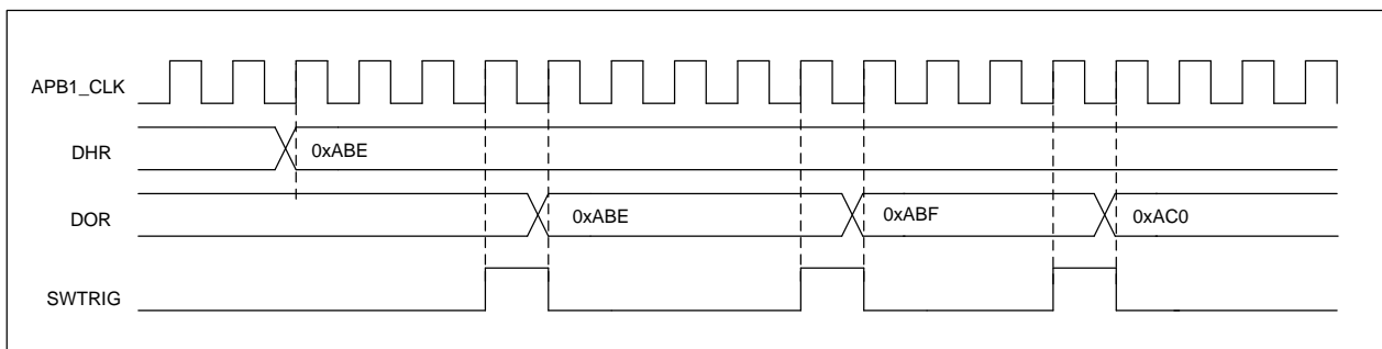
Figure 10-8 DAC conversion (SW trigger enabled) with triangle wave generation
