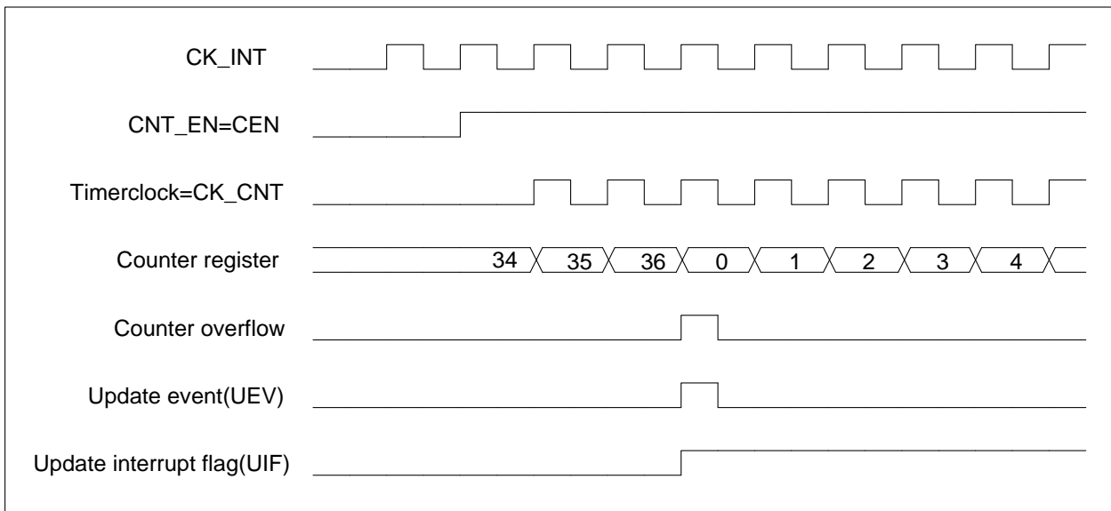
Figure 14-4 Counter timing diagram, internal clock divided by 1
