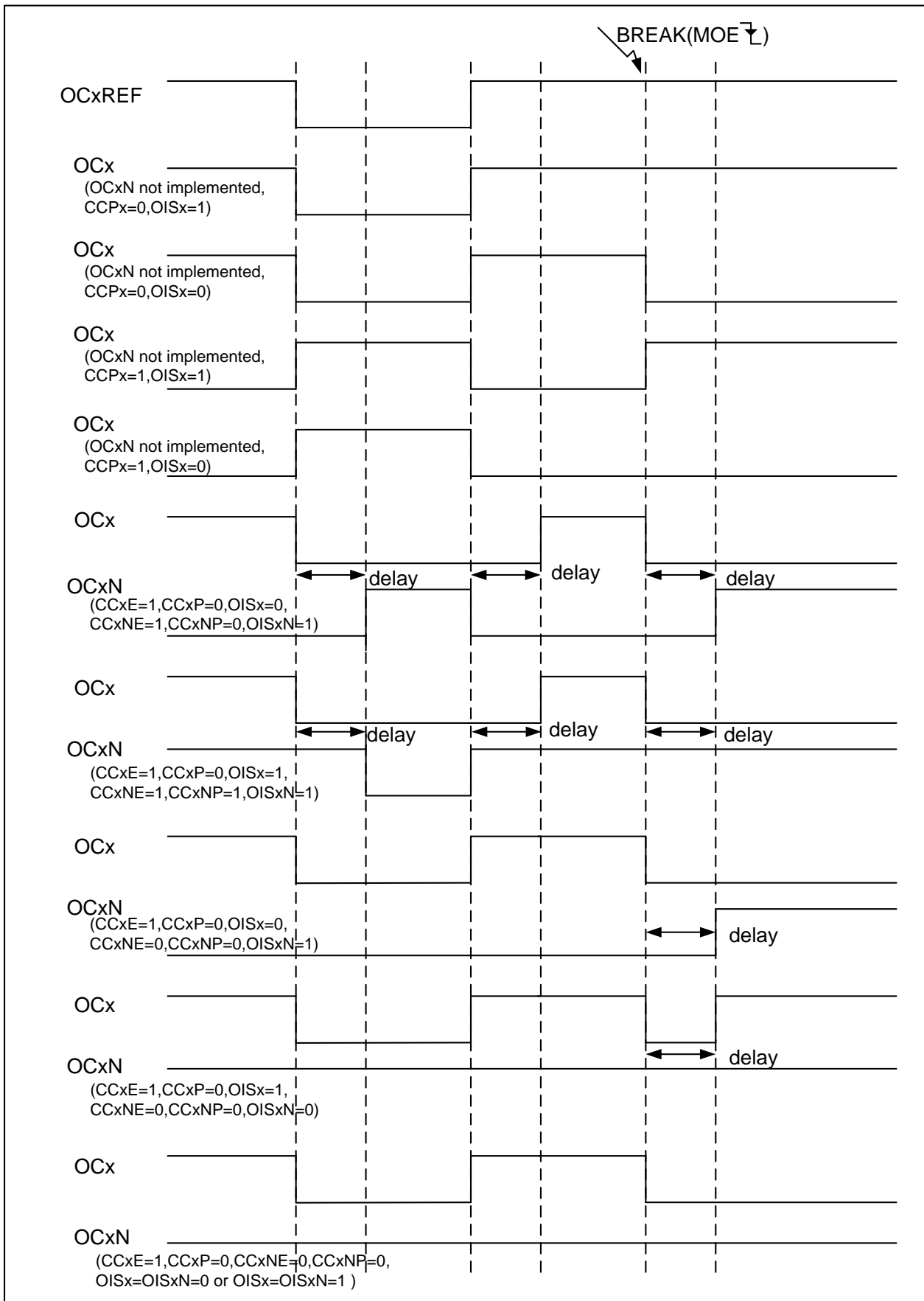
Figure 12-38 Output behavior in response to a break
