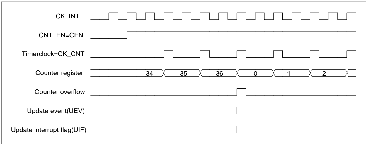
Figure 14-5 Counter timing diagram, internal clock divided by 2
