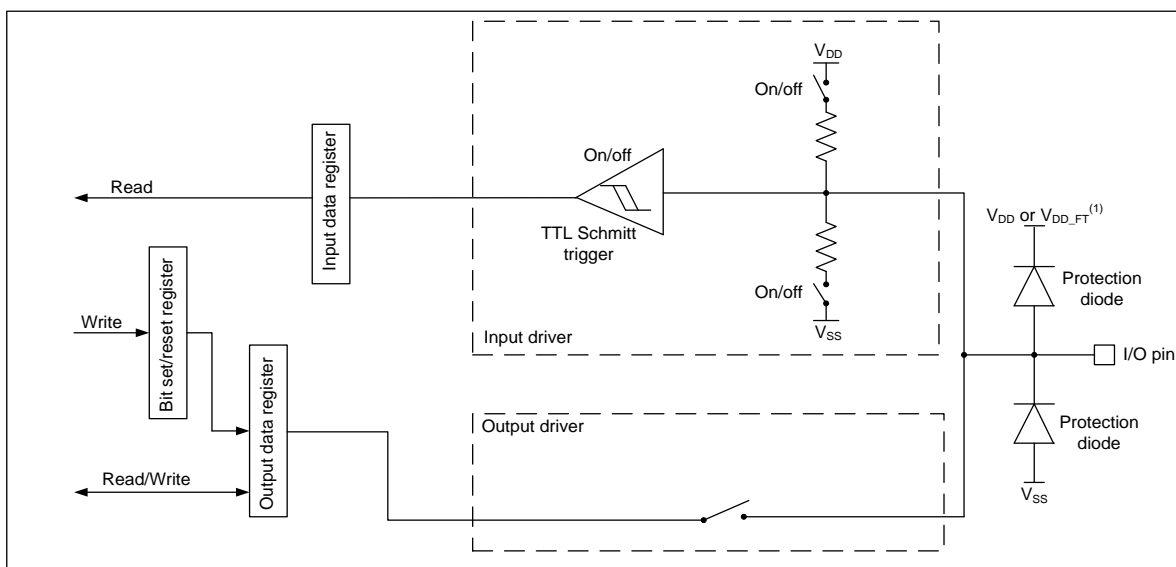
Figure 7-3 Input floating/pull up/pull down configurations
