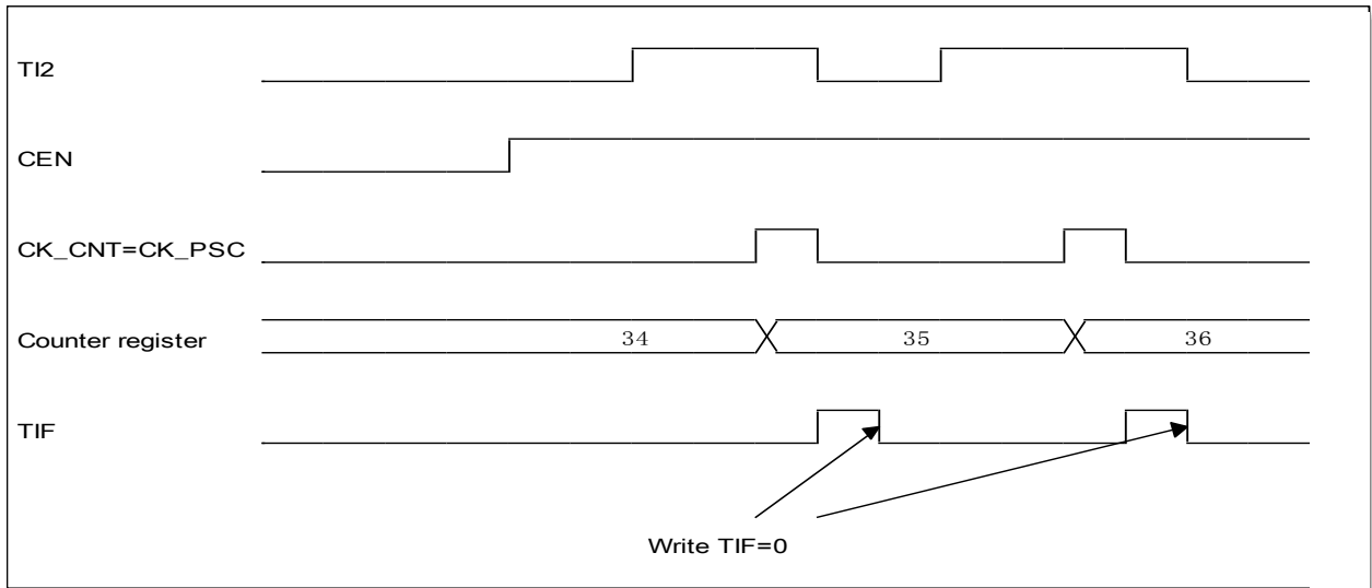
Figure 13-23 Control circuit in external clock mode 1
