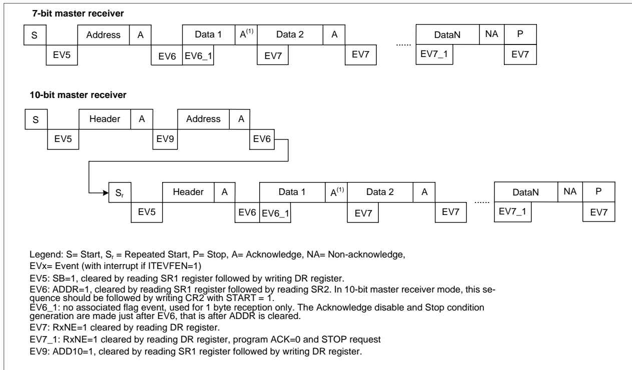
Figure 23-6 Method 1: transfer sequence diagram for master receiver
