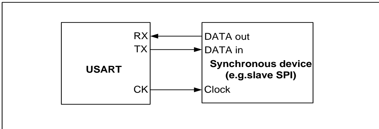
Figure 24-11 USART example of synchronous transmission
