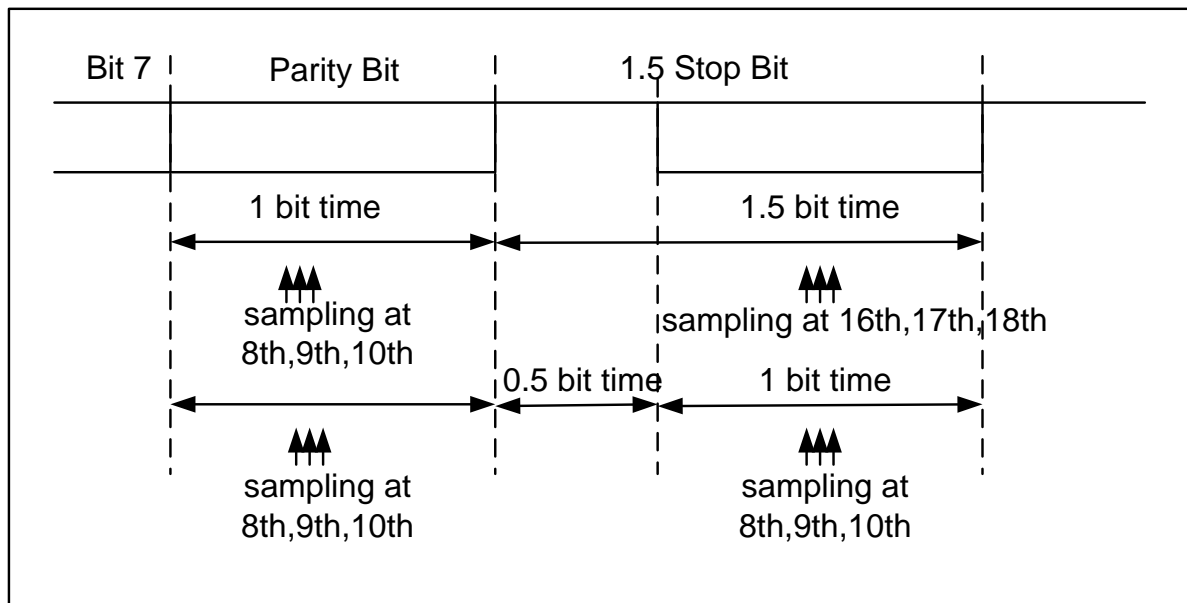
Figure 24-16 Parity error detection using the 1.5 stop bits
