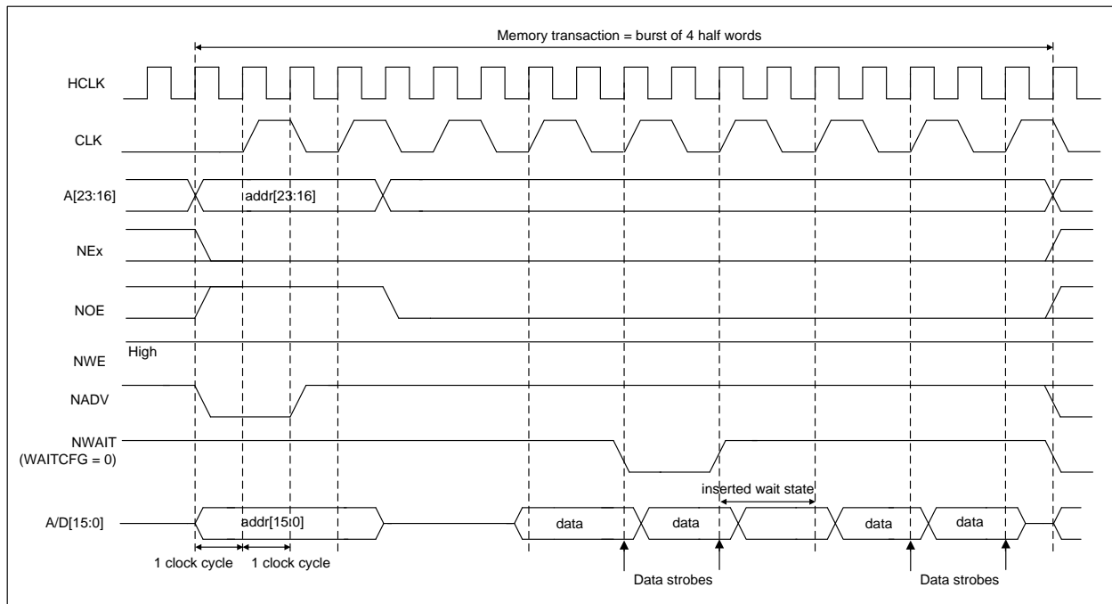
Figure 18-19 Synchronous multiplexed read mode - NOR, PSRAM (CRAM)
