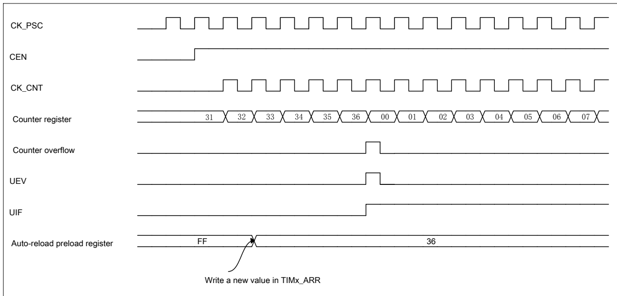
Figure 12-8 Counter timing diagram, update event when ARPE=0(TIMx_ARR not preloaded)
