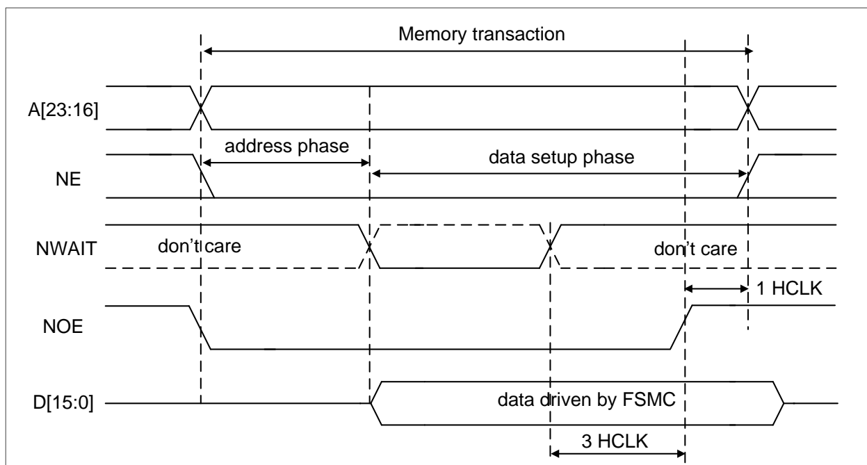
Figure 18-17 Asynchronous wait during a write access
