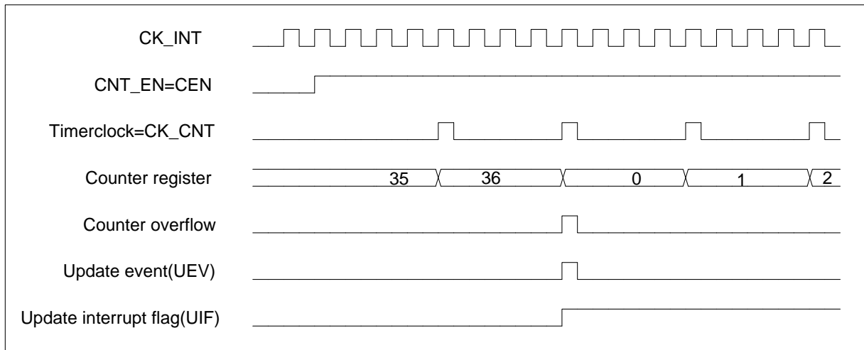
Figure 13-7 Counter timing diagram, internal clock divided by N
