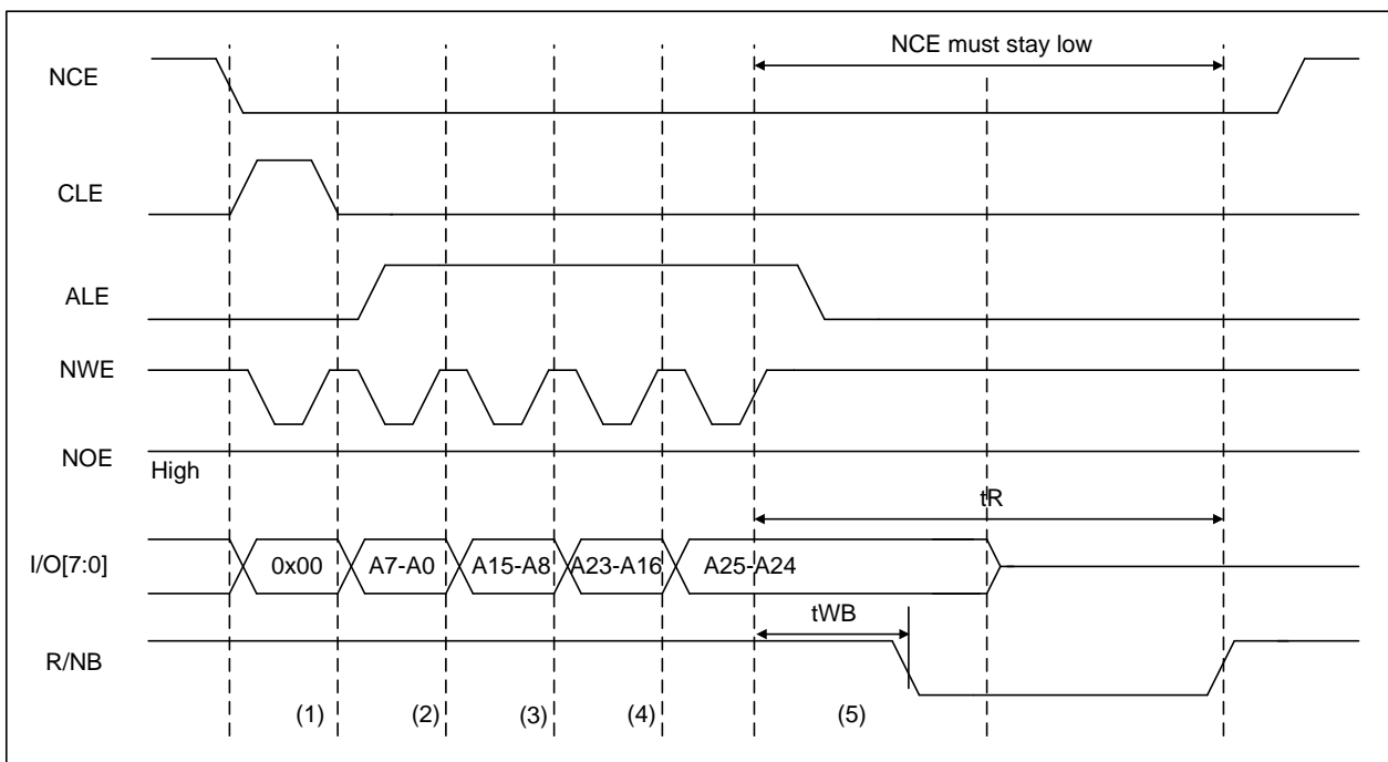
Figure 18-22 Access to non ‘CE don’t care’ NAND-Flash
