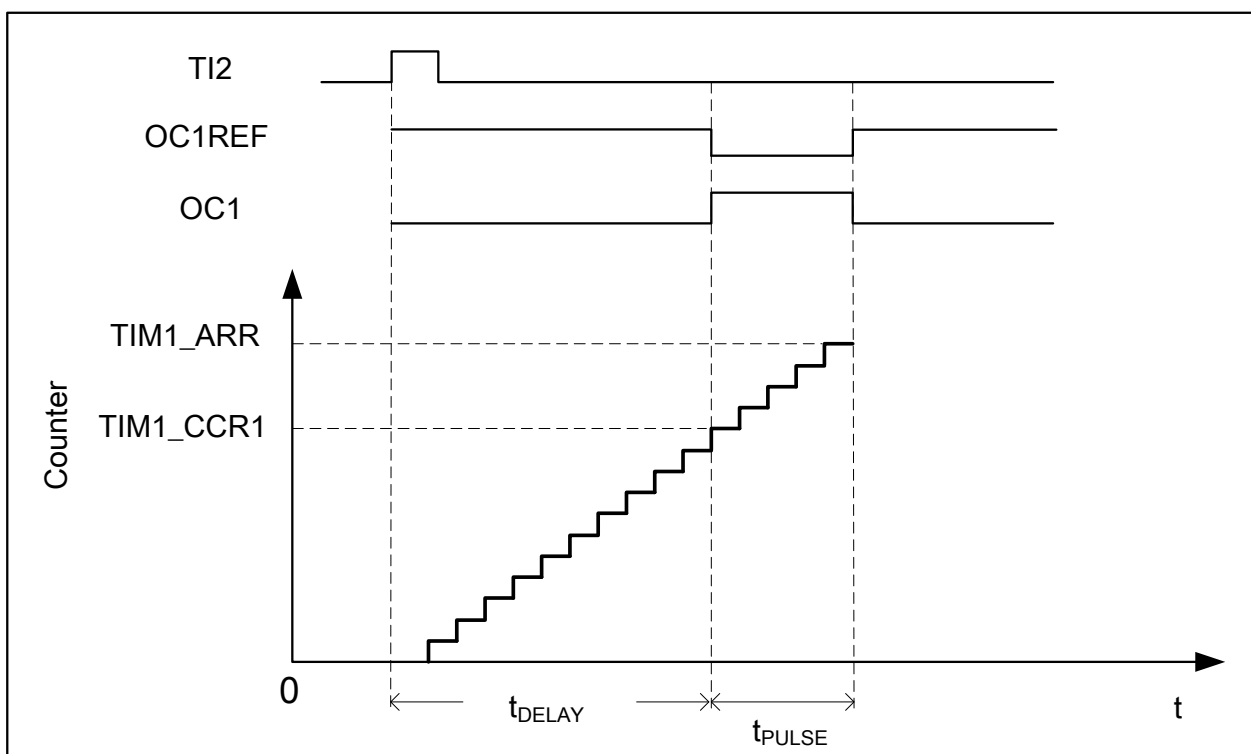
Figure 12-41 Example of one pulse mode
