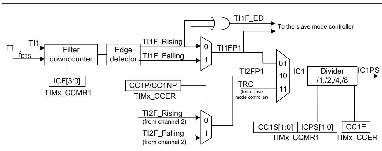
Figure 13-26 Capture/compare channel (example: channel 1 input stage)
