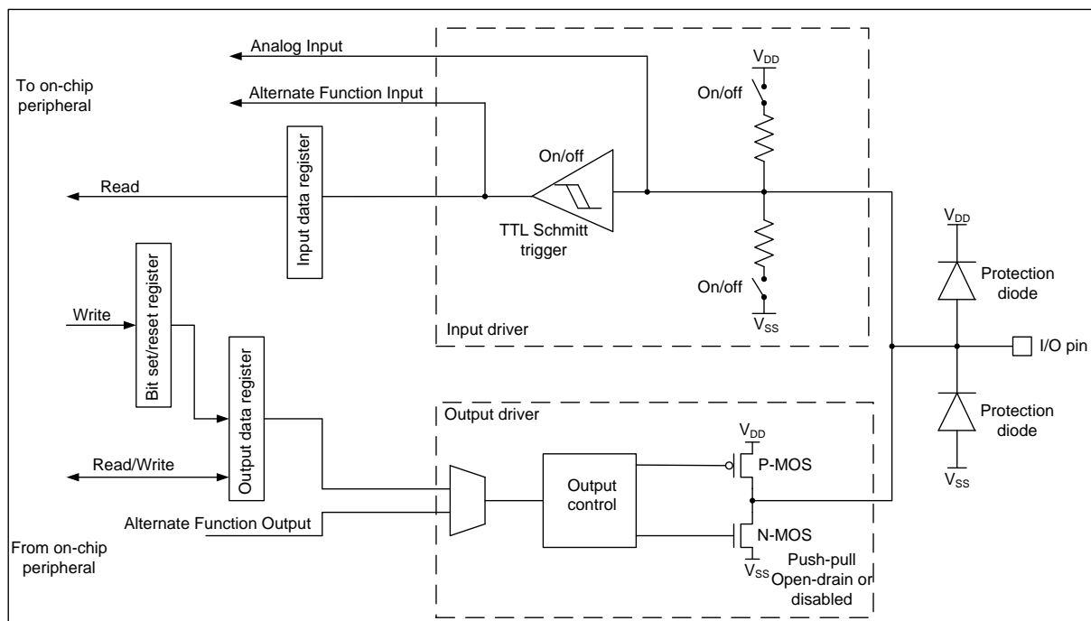
Figure 7-1 Basic structure of a standard I/O port bit
