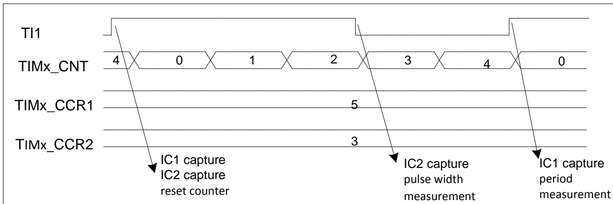
Figure 12-31 PWM input mode timing
