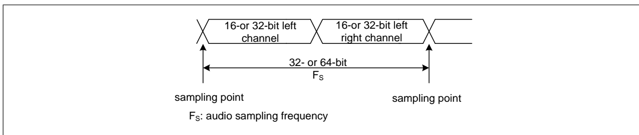
Figure 22-30 Audio sampling frequency definition
