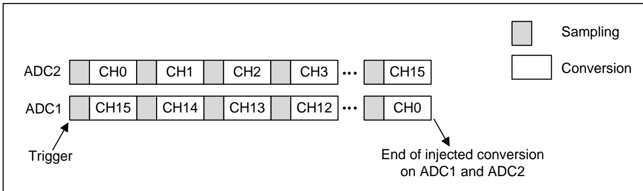
Figure 9-10 Regular simultaneous mode on 16 channels
