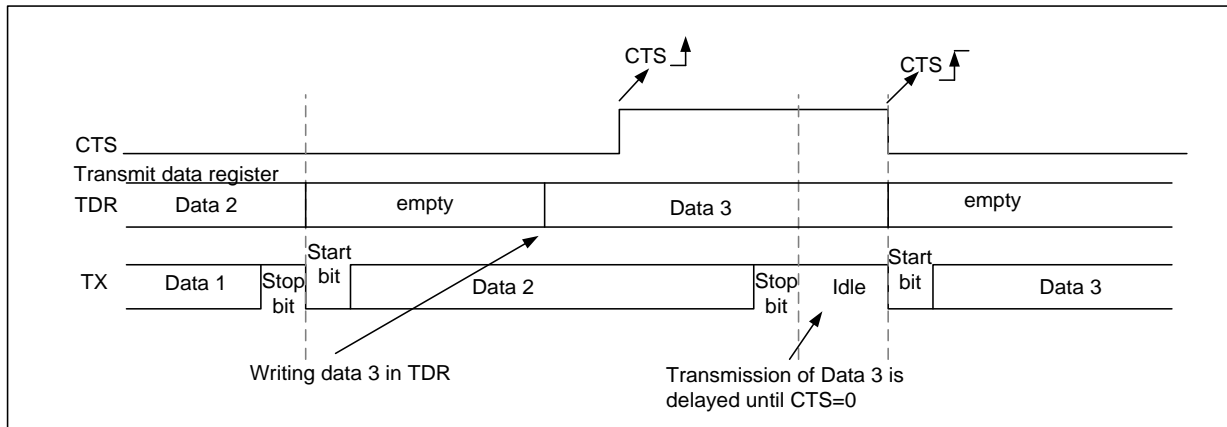
Figure 24-23 CTS flow control
