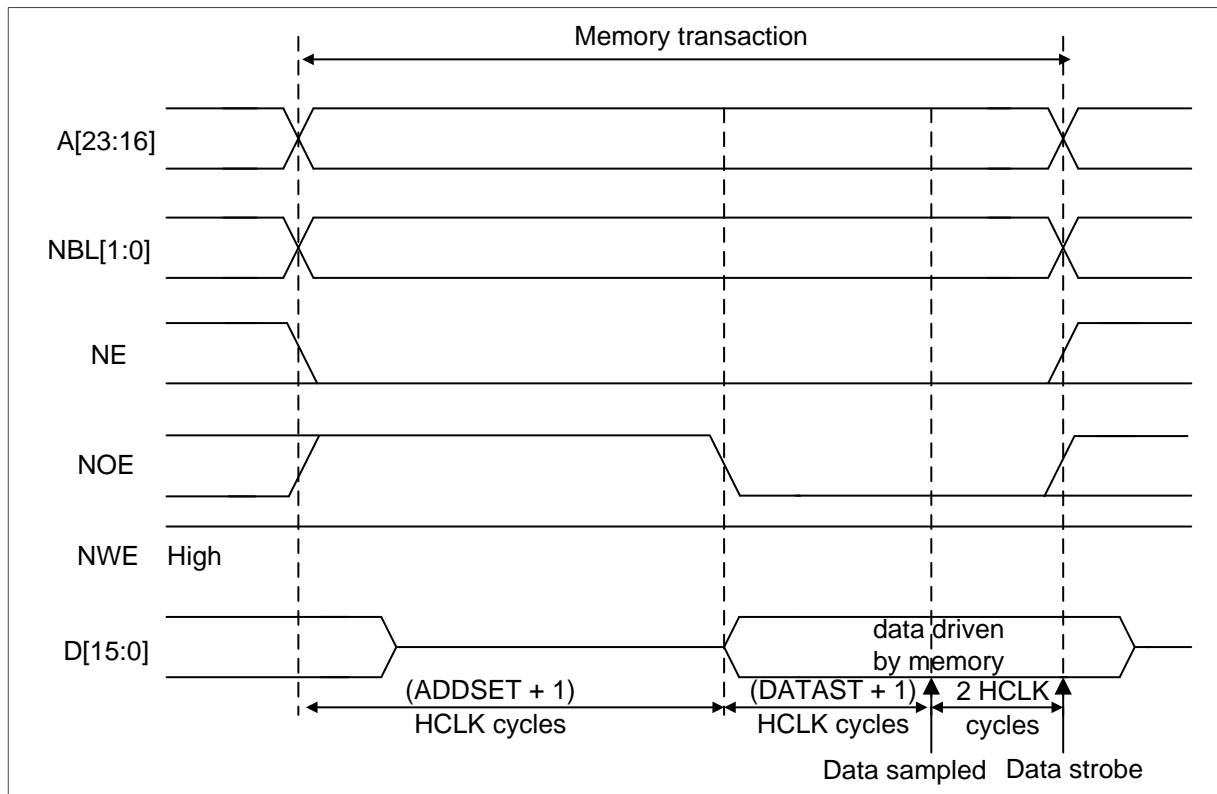
Figure 18-5 ModeA read accesses
