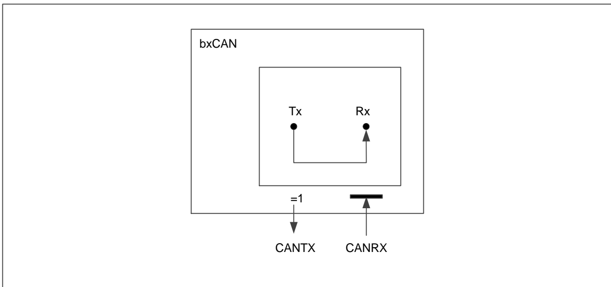
Figure 21-5 bxCAN in combined mode
