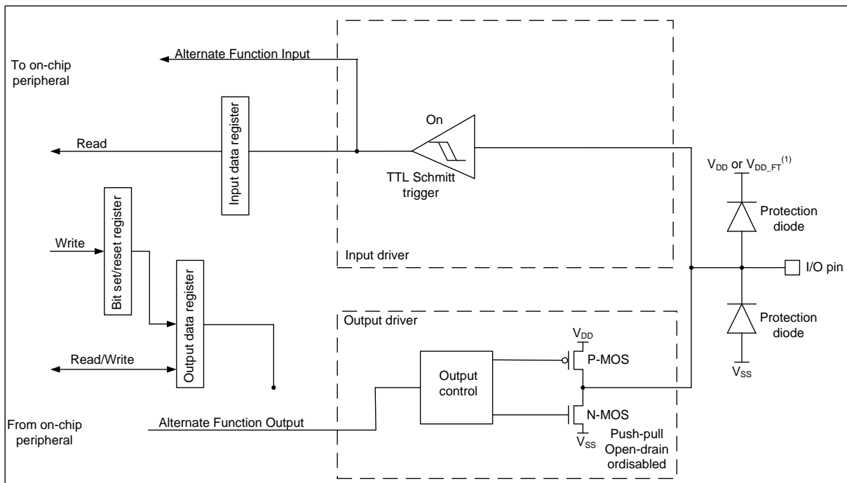
Figure 7-5 Alternate function configuration
