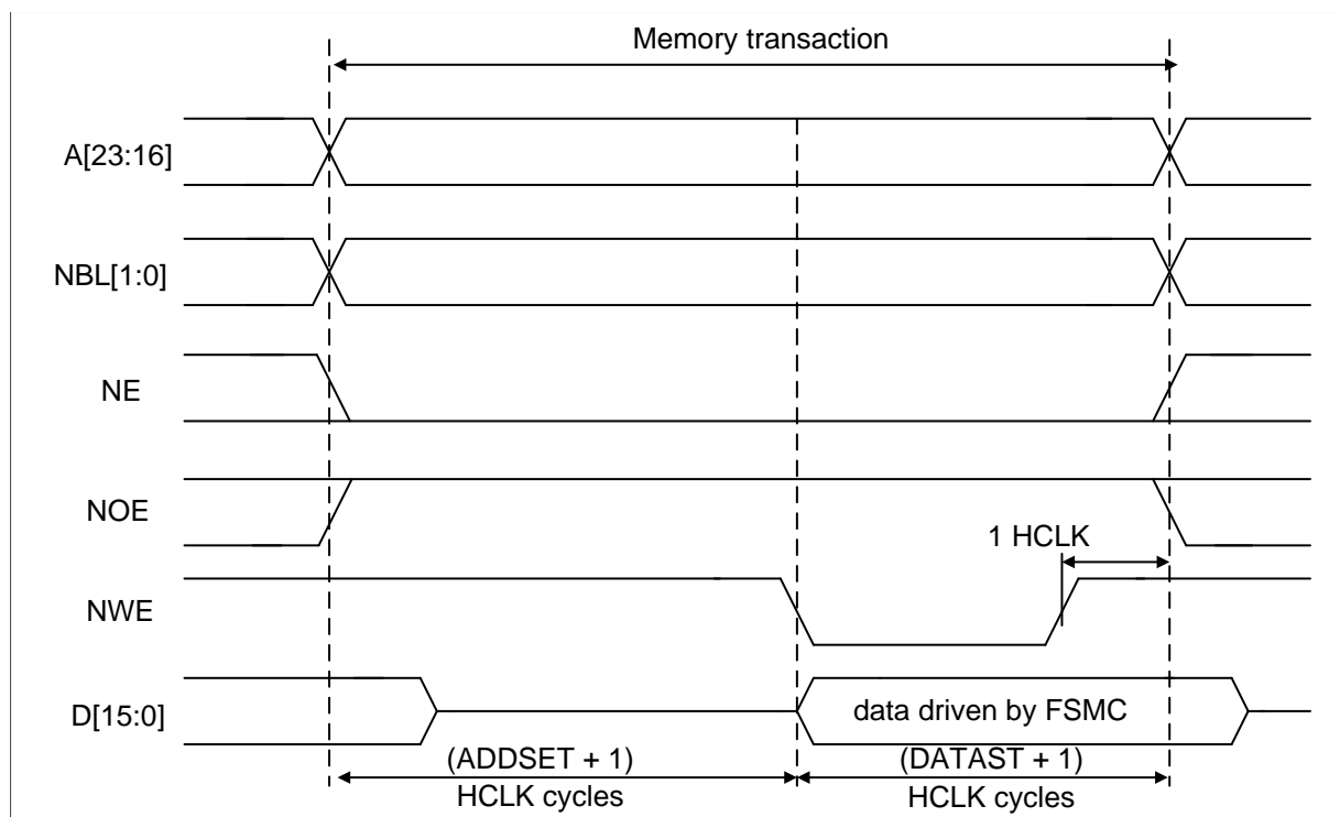
Figure 18-6 ModeA write accesses
