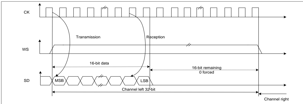
Figure 22-21 MSB justified 16-bit extended to 32-bit packet frame with CPOL = 0
