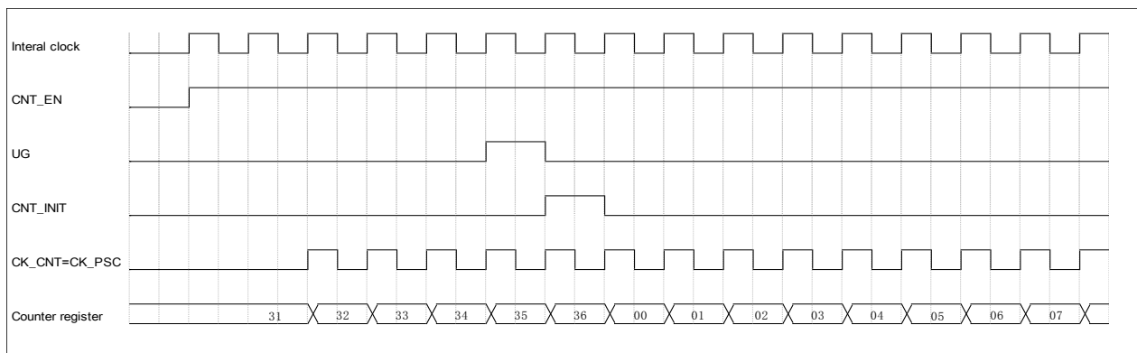
Figure 12-22 Control circuit in normal mode, internal clock divided by 1
