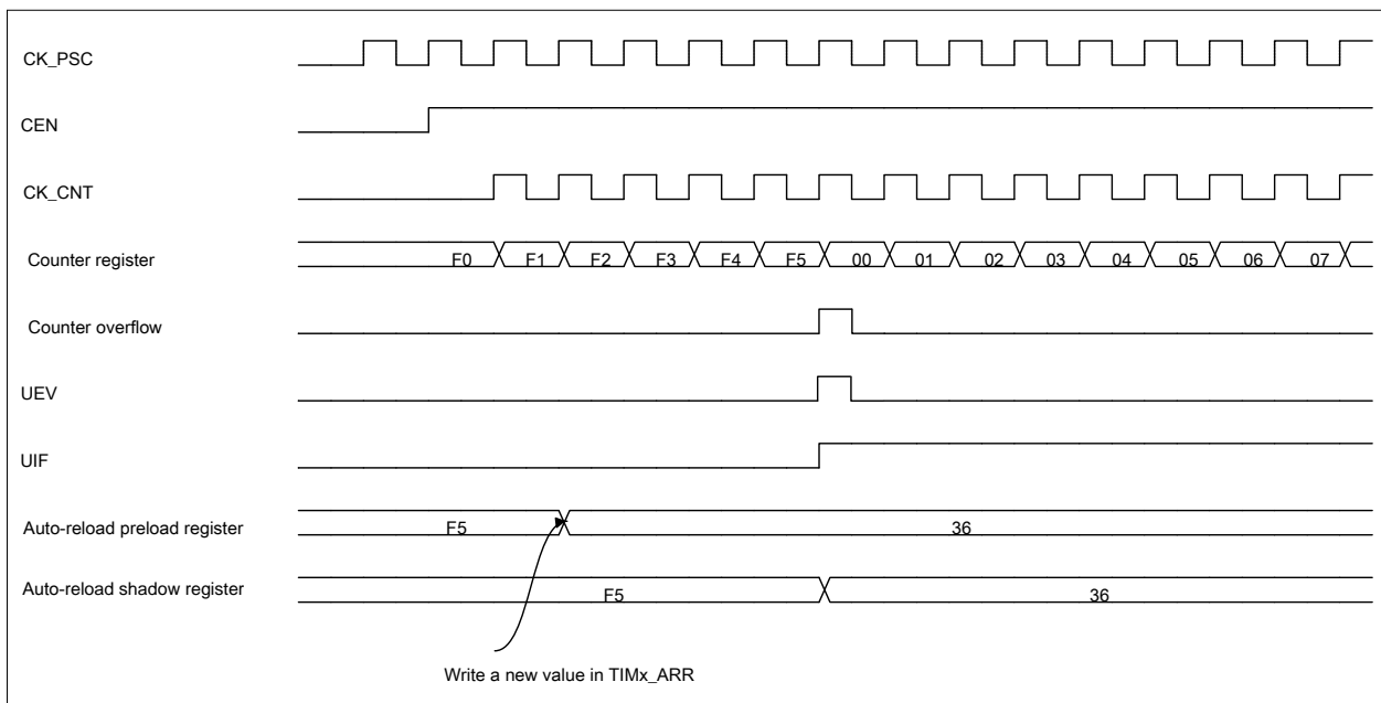
Figure 14-9 Counter timing diagram, update event when ARPE=1(TIMx_ARR preloaded)
