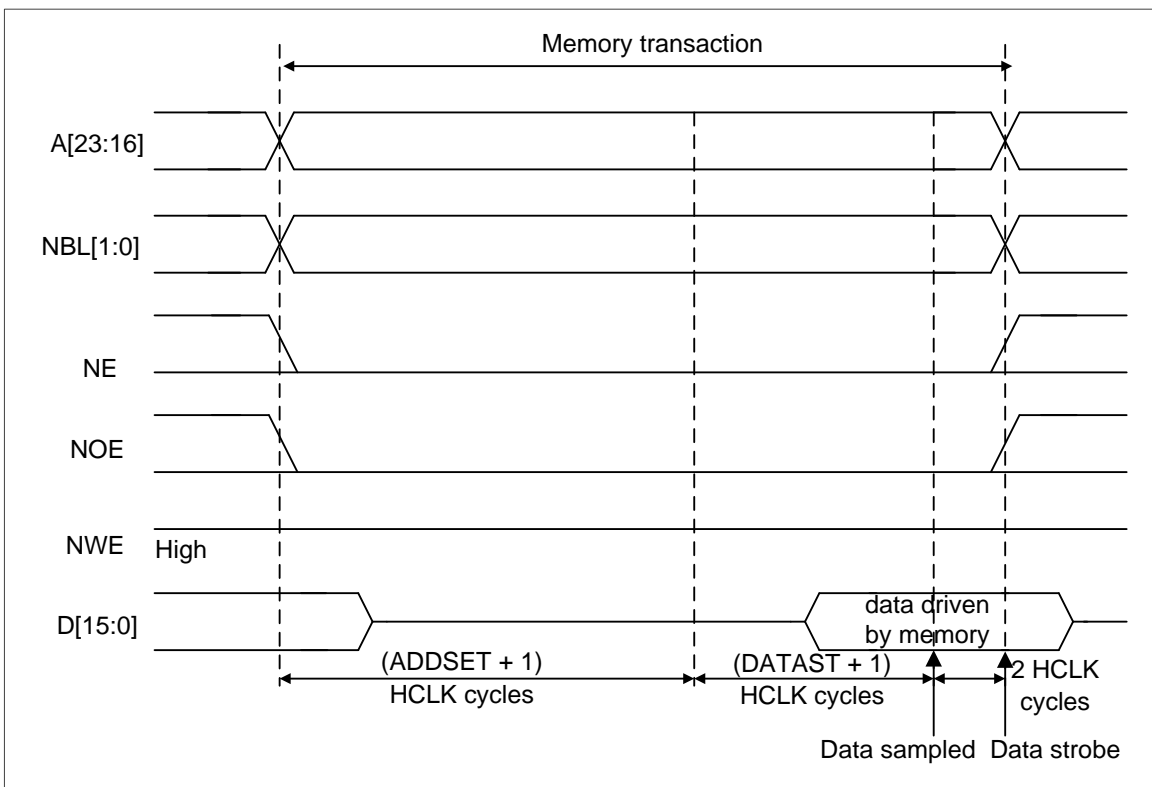
Figure 18-3 Mode1 read accesses
