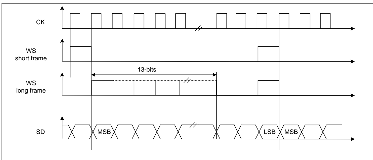
Figure 22-28 PCM standard waveforms (16-bit)
