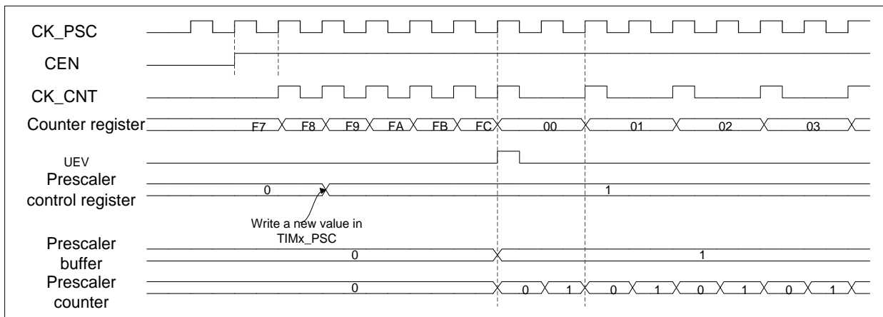
Figure 12-2 Counter timing diagram with prescaler division change from 1 to 2
