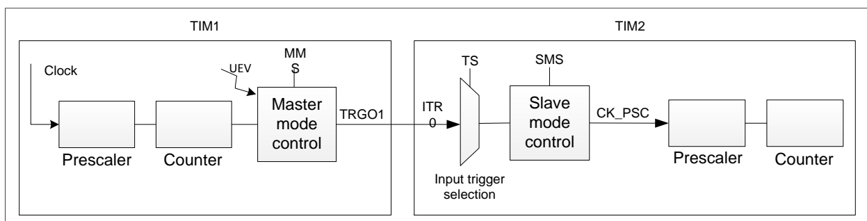
Figure 13-41 Master/Slave timer example
