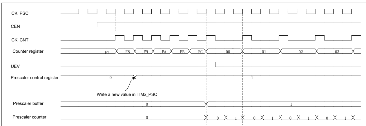
Figure 13-2 Counter timing diagram with prescaler division change from 1 to 2
