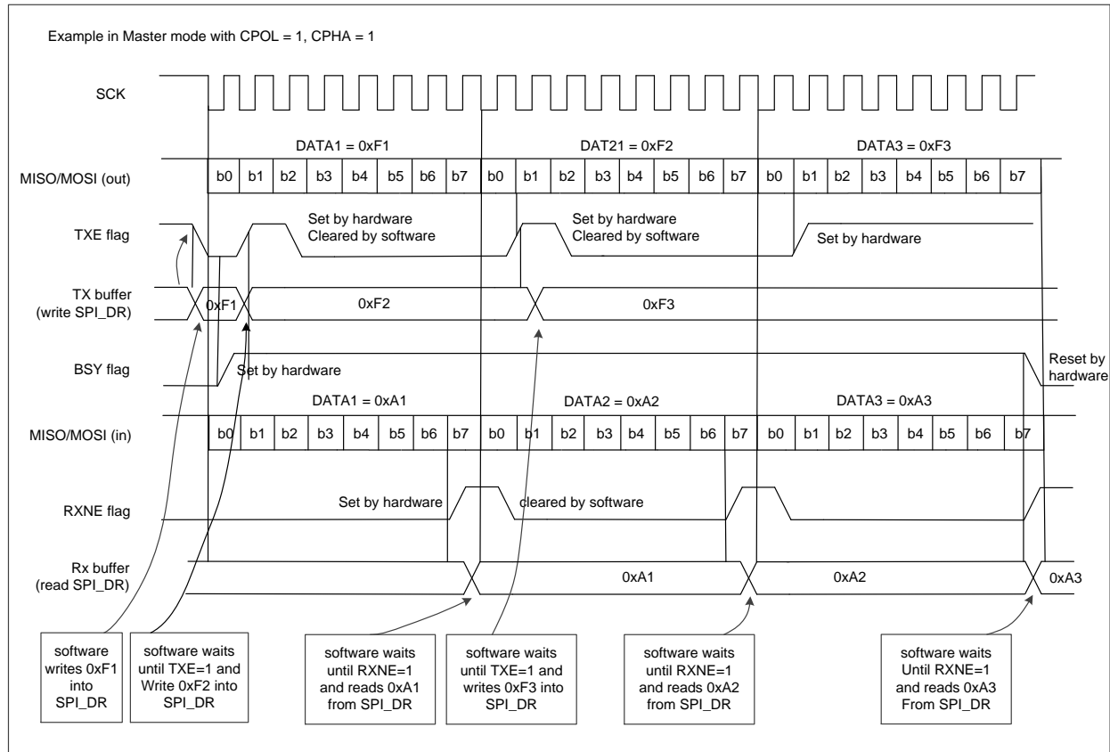
Figure 22-4 TXE/RXNE/BSY behavior in Master / full-duplex mode (BIDIMODE=0 and RXONLY=0) in case of continuous transfers
