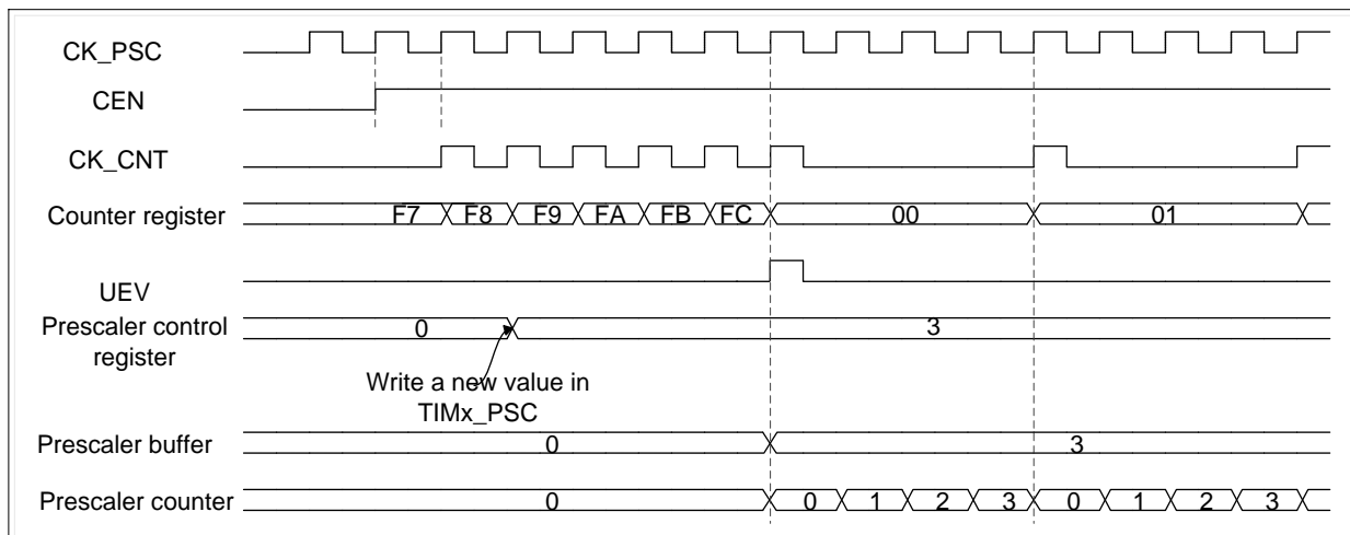
Figure 12-3 Counter timing diagram with prescaler division change from 1 to 4
