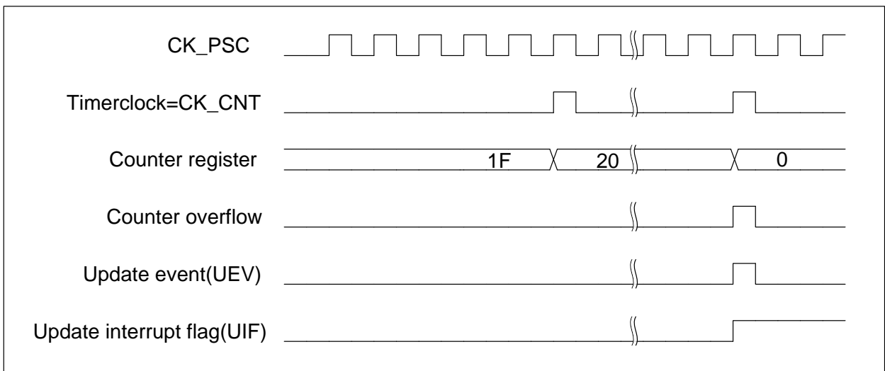
Figure 12-7 Counter timing diagram, internal clock divided by N
