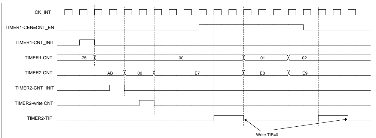
Figure 13-43 Gating timer 2 with Enable of timer 1
