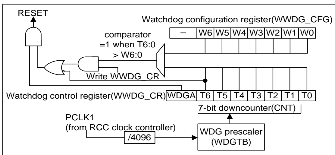
Figure 17-1 Watchdog block diagram
