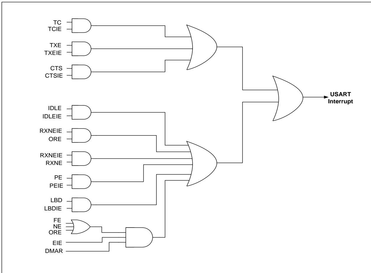
Figure 24-24 USART interrupt mapping diagram
