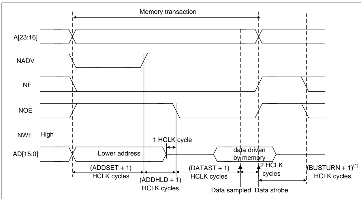
Figure 18-14 Multiplexed read accesses
