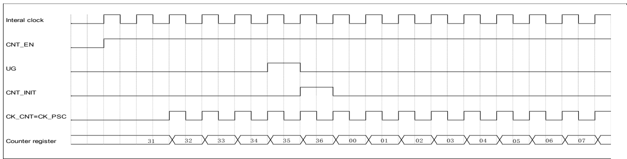
Figure 13-21 Control circuit in normal mode, internal clock divided by 1
