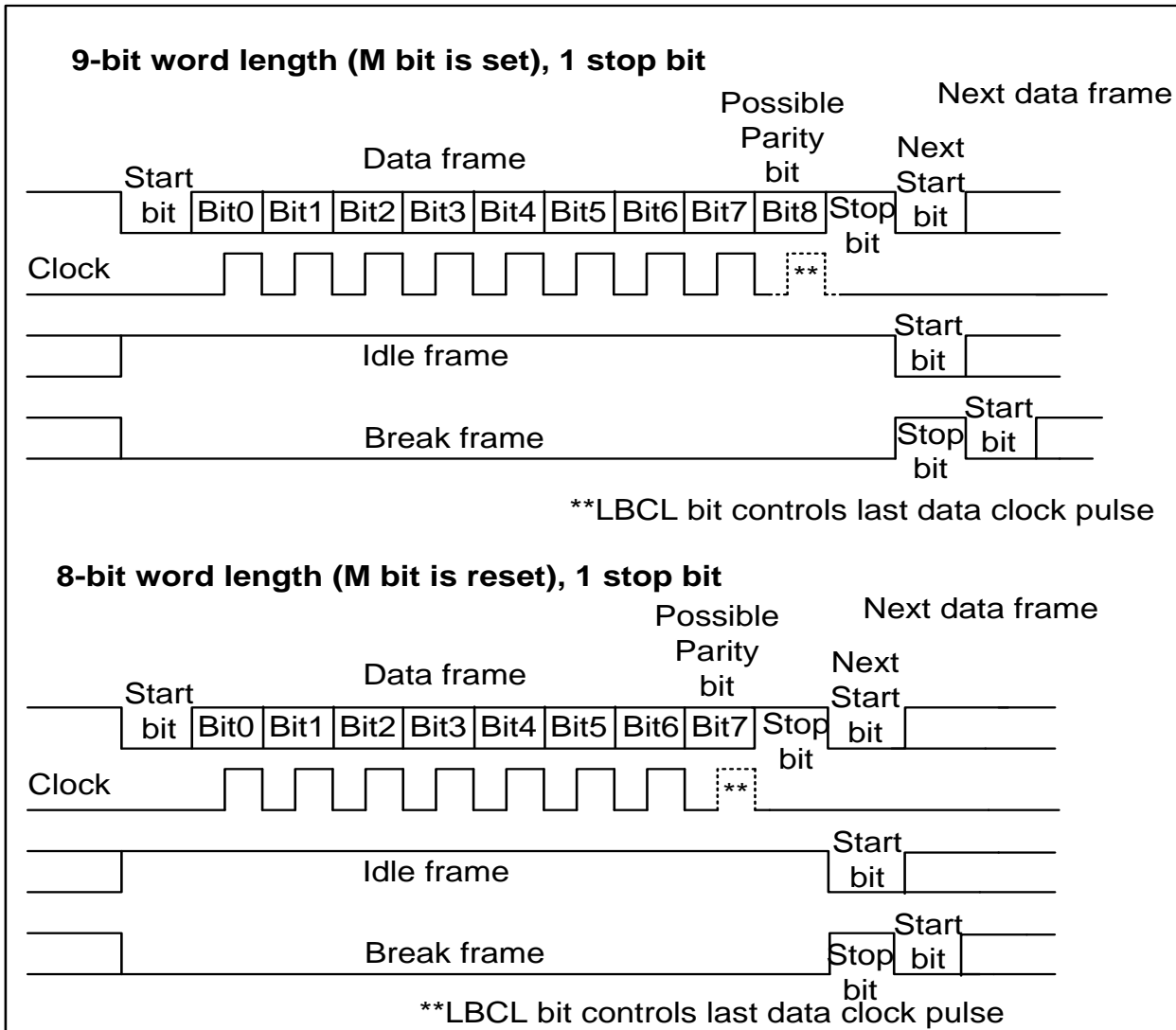
Figure 24-2 Word length programming
