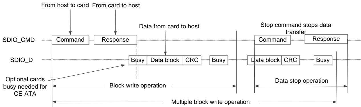
Figure 19-3 SDIO (multiple) block write operation
