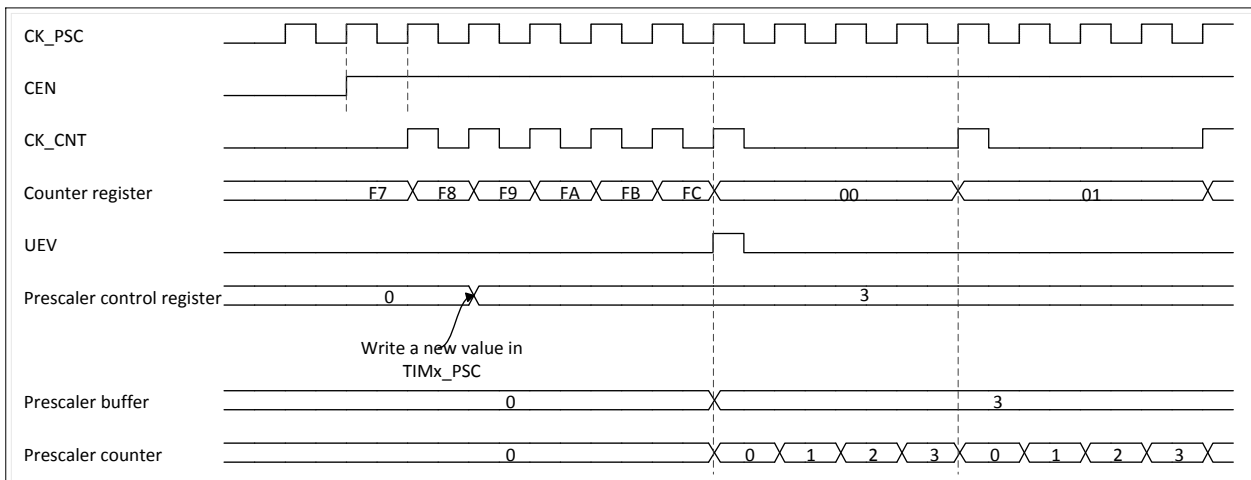
Figure 13-3 Counter timing diagram with prescaler division change from 1 to 4
