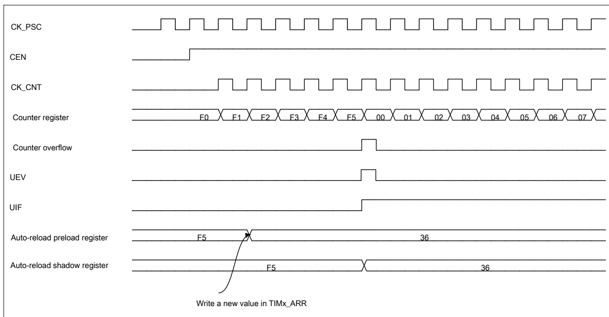
Figure 12-9 Counter timing diagram, update event when ARPE=1(TIMx_ARR preloaded)
