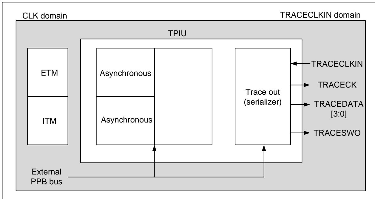
Figure 26-4 TPIU block diagram
