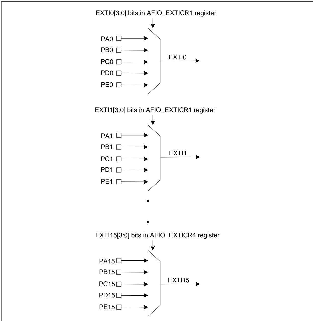
Figure 8-2 External interrupt/event GPIO mapping
