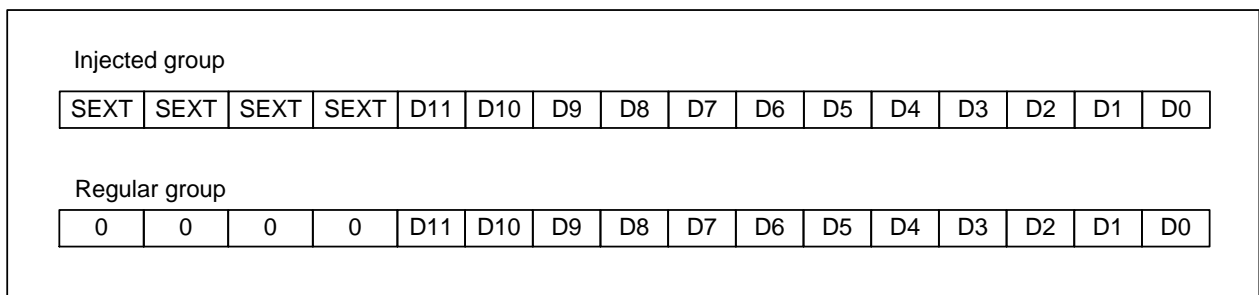
Figure 9-6 Right alignment of data
