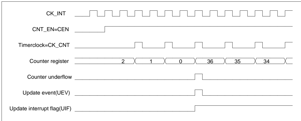
Figure 13-11 Counter timing diagram, internal clock divided by 2
