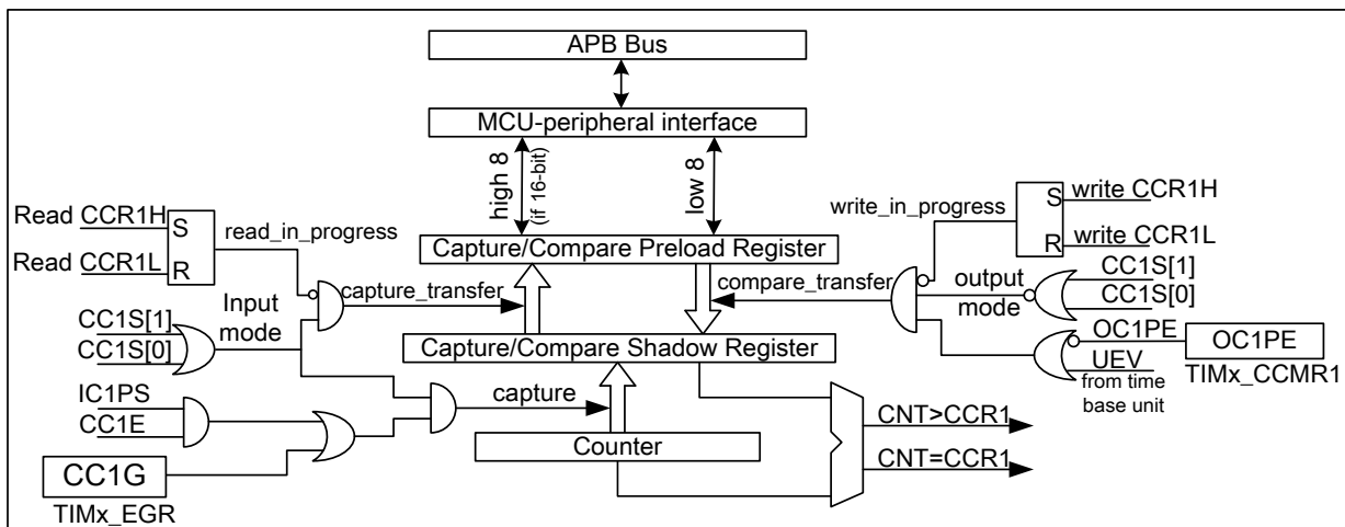
Figure 12-28 Capture/compare channel 1 main circuit
