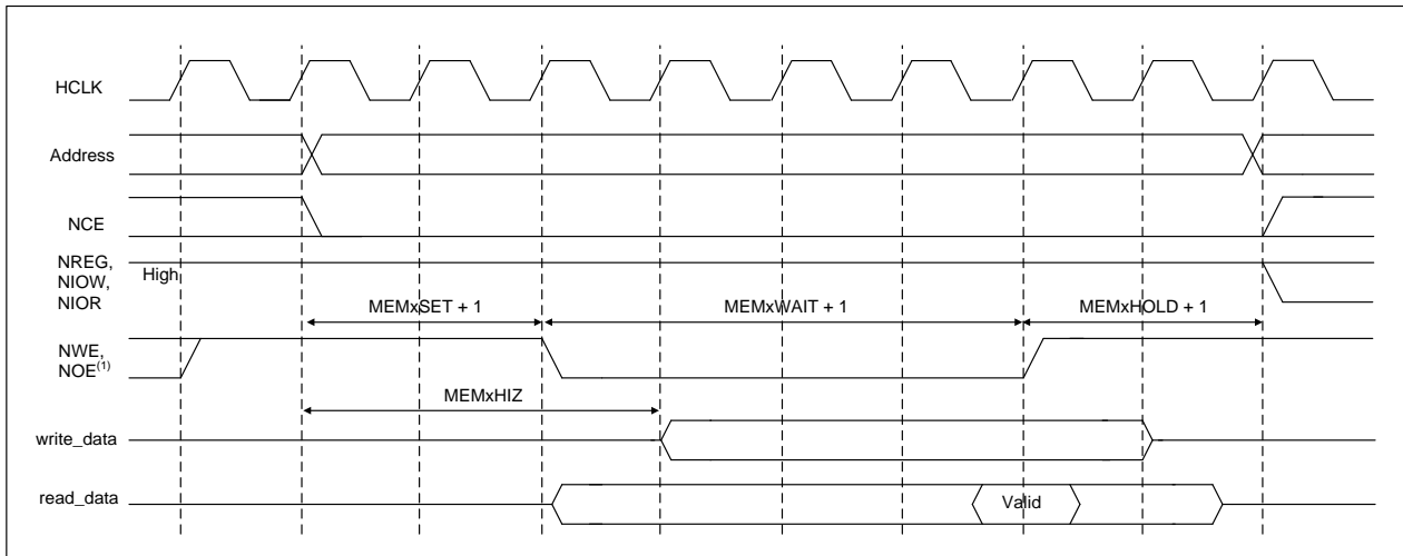
Figure 18-21 NAND controller timing for common memory access
