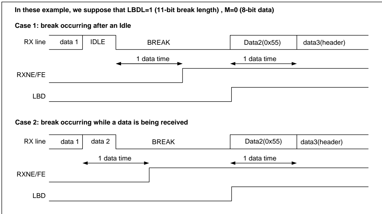
Figure 24-10 Break detection in LIN mode vs. Framing error detection
