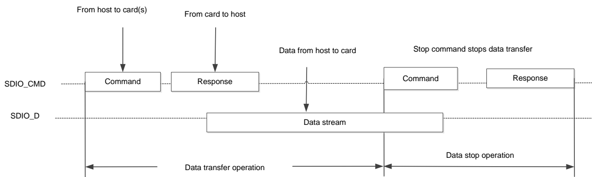
Figure 19-5 SDIO sequential write operation
