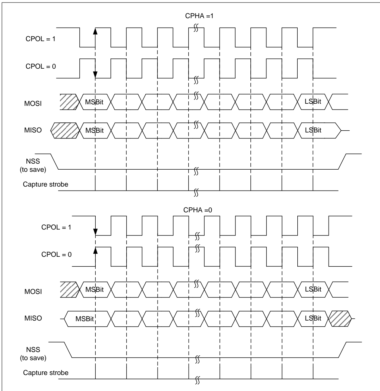
Figure 22-3 Data clock timing diagram
