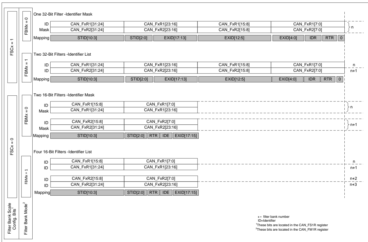
Figure 21-8 Filter bank scale configuration - register organization
