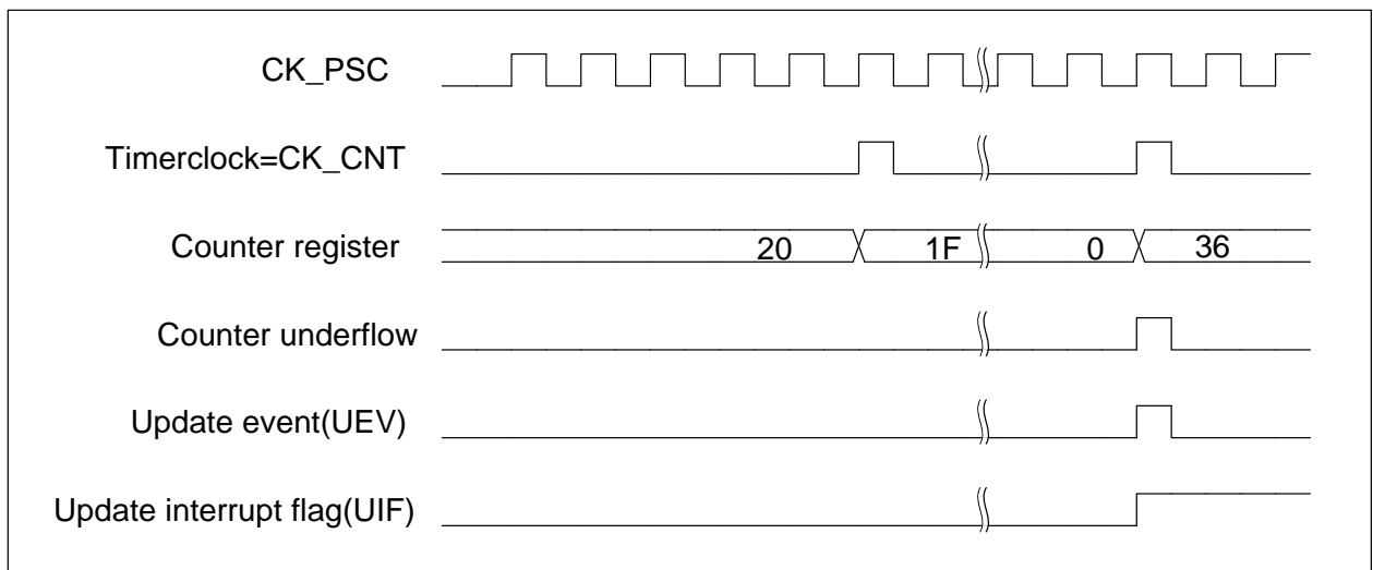
Figure 12-13 Counter timing diagram, internal clock divided by N
