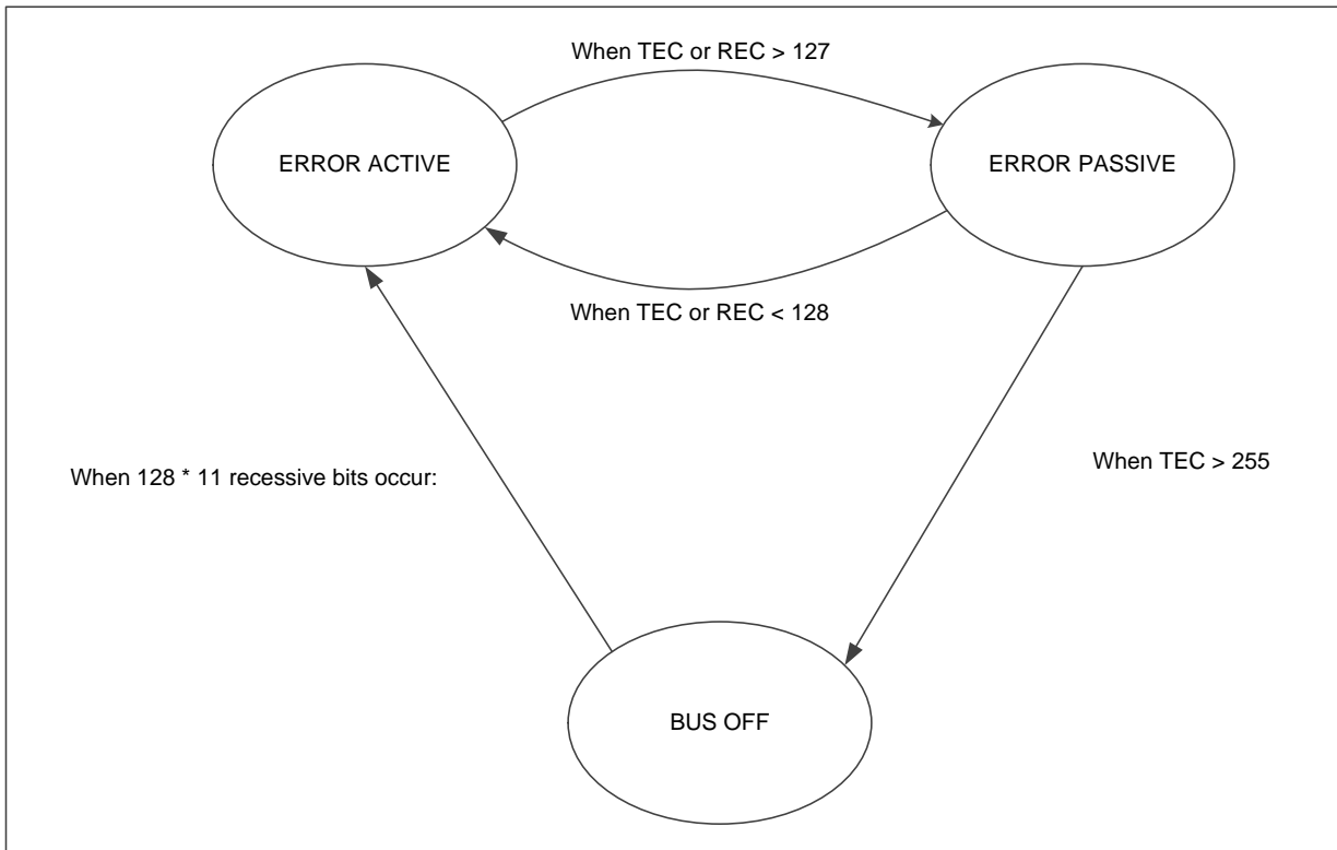
Figure 21-11 CAN error state diagram
