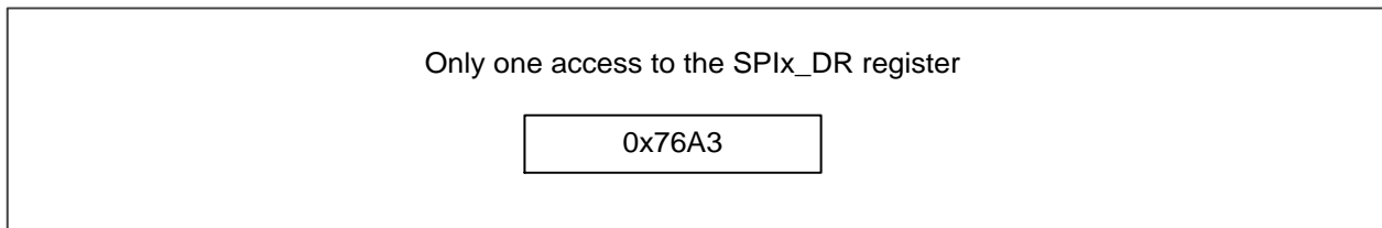
Figure 22-27 Example of LSB justified 16-bit extended to 32-bit packet frame
