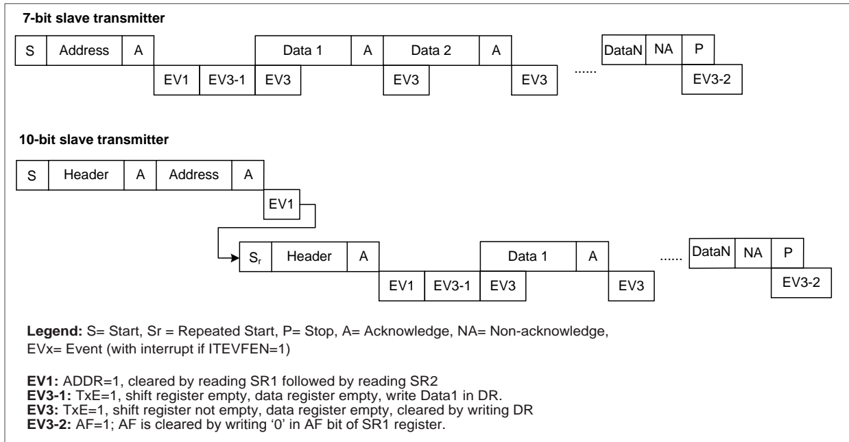
Figure 23-3 Transfer sequence diagram for slave transmitter
