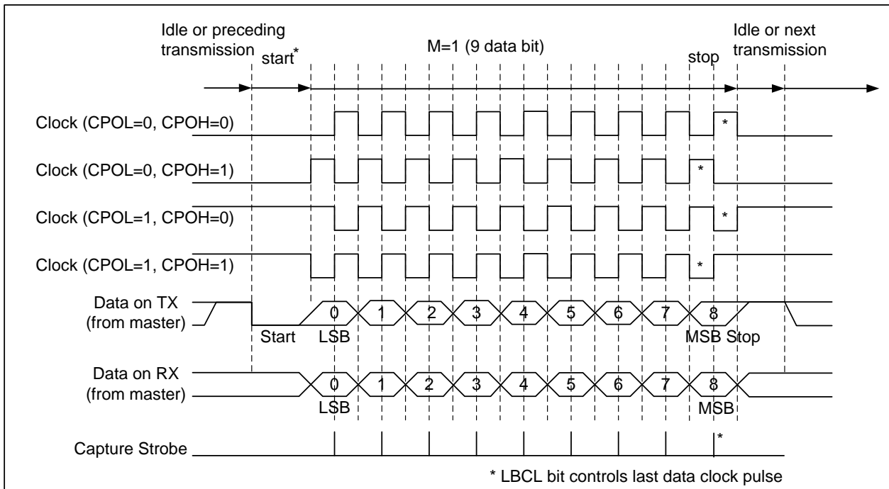
Figure 24-13 USART data clock timing diagram (M=1)
