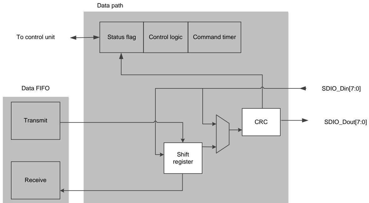
Figure 19-12 Data path
