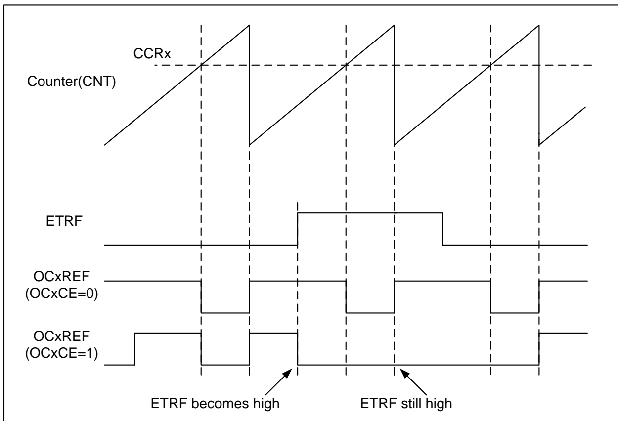
Figure 12-39 Clearing TIMx OCxREF
