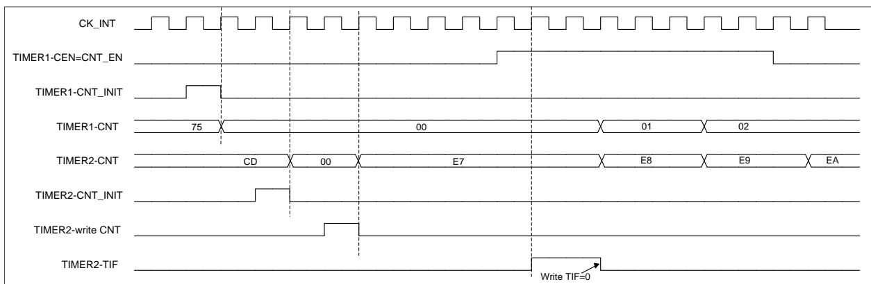
Figure 13-45 Triggering timer 2 with Enable of timer 1
