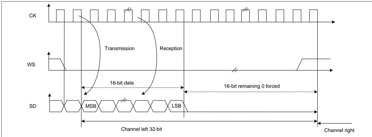
Figure 22-17 I2S Philips standard (16-bit extended to 32-bit packet frame with CPOL = 0)
