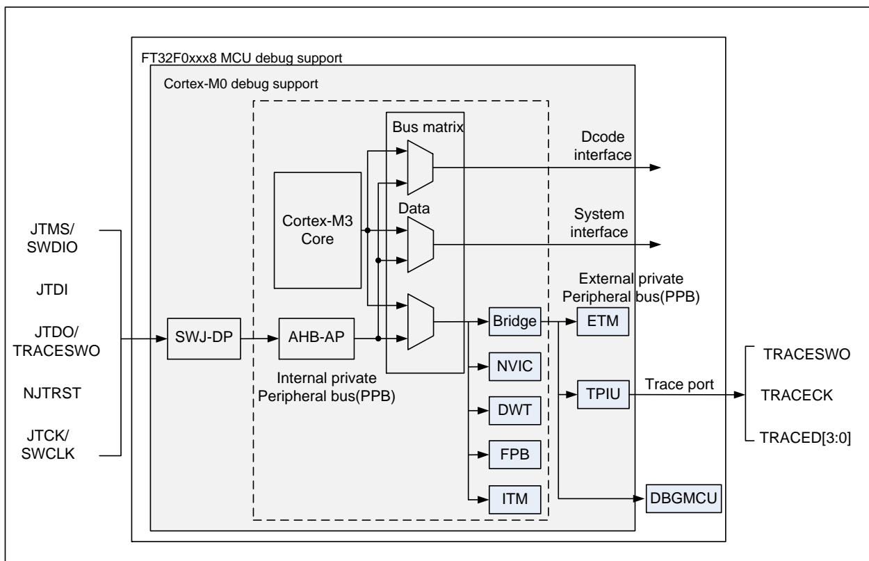
Figure 26-1 Block diagram of FT32 MCU and Cortex ® -M3-level debug support
