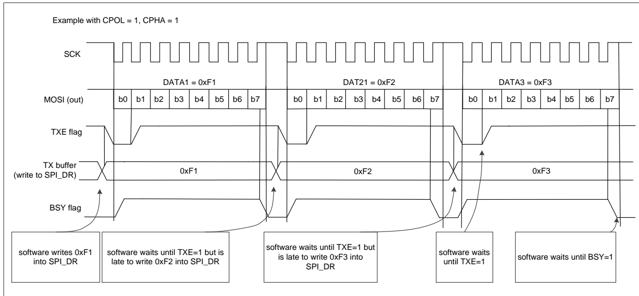
Figure 22-9 TXE/BSY behavior when transmitting (BIDIRMODE=0 and RXONLY=0) in case of discontinuous transfers
