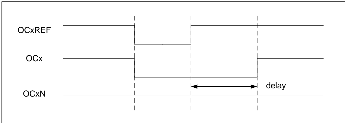
Figure 12-37 Dead-time waveforms with delay greater than the positive pulse
