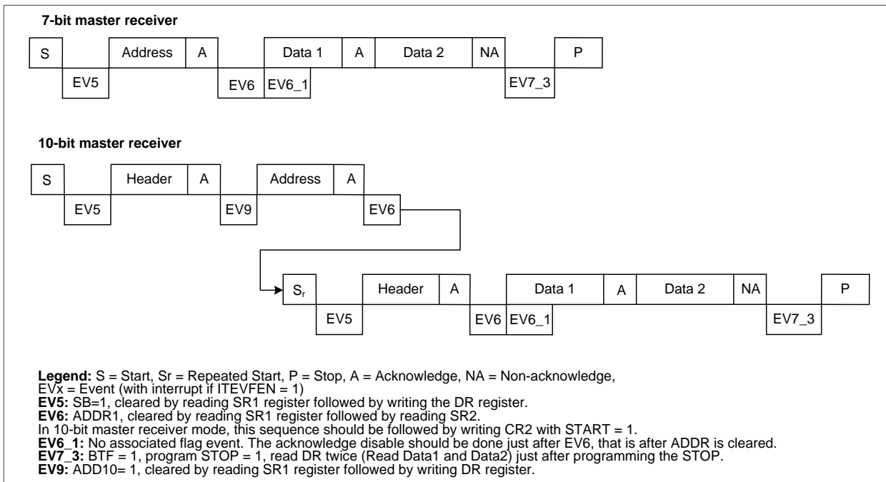
Figure 23-8 Method 2: transfer sequence diagram for master receiver when N=2
