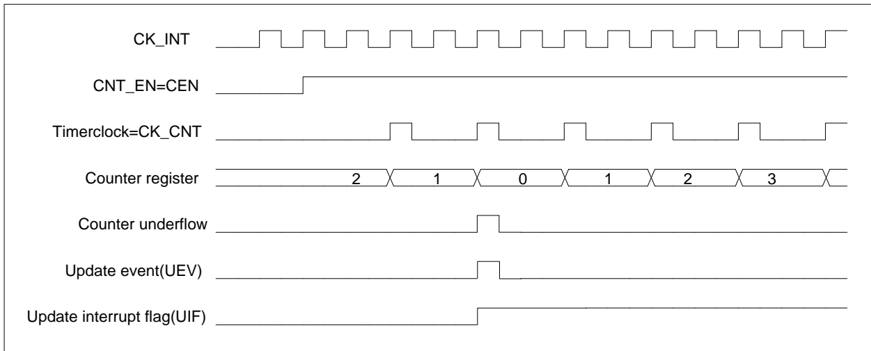
Figure 13-16 Counter timing diagram, internal clock divided by 2
