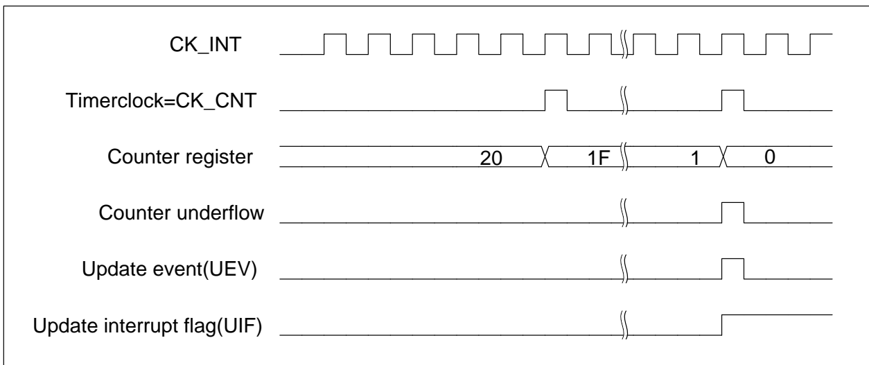
Figure 13-18 Counter timing diagram, internal clock divided by N
