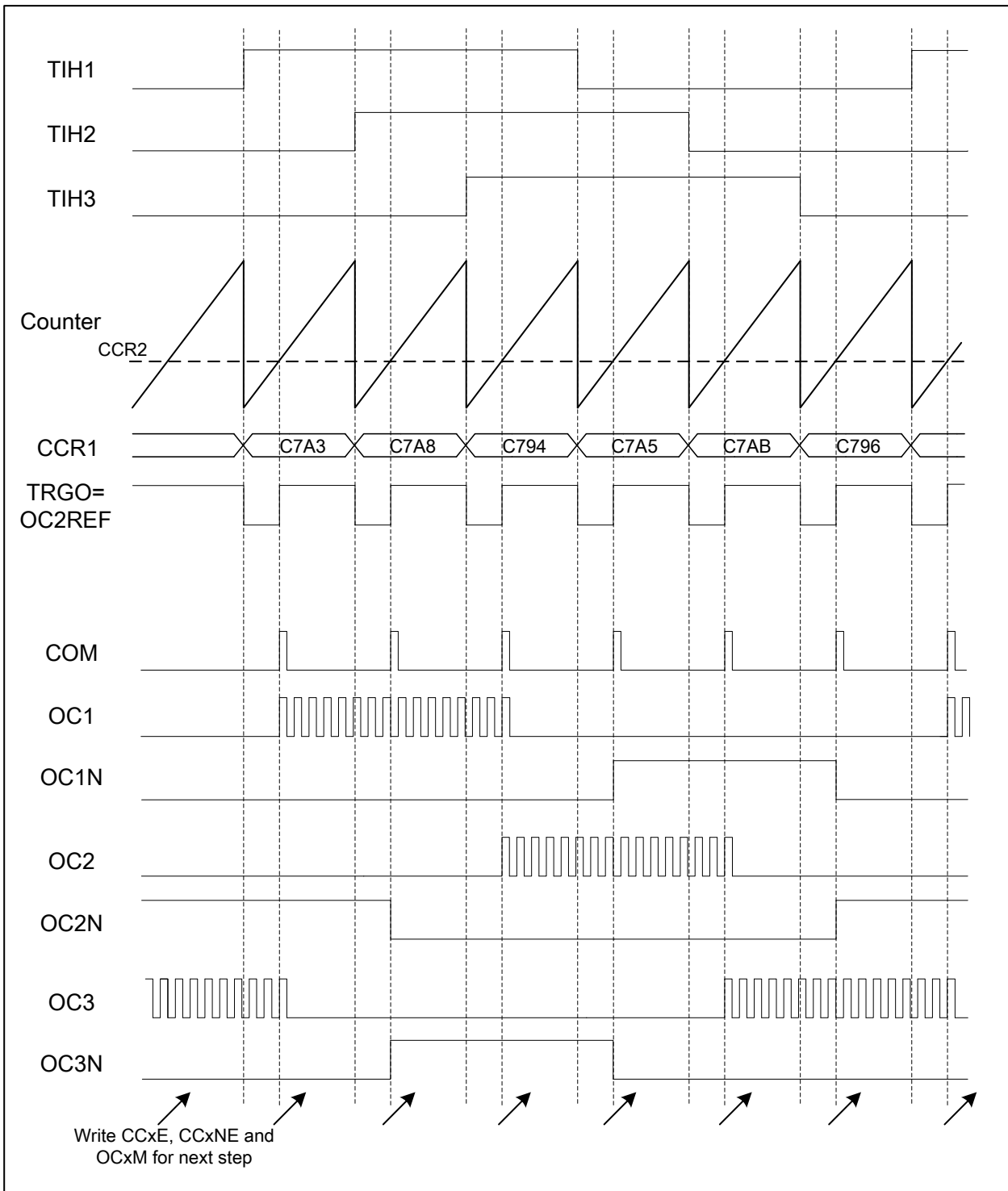
Figure 12-44 Example of Hall sensor interface
