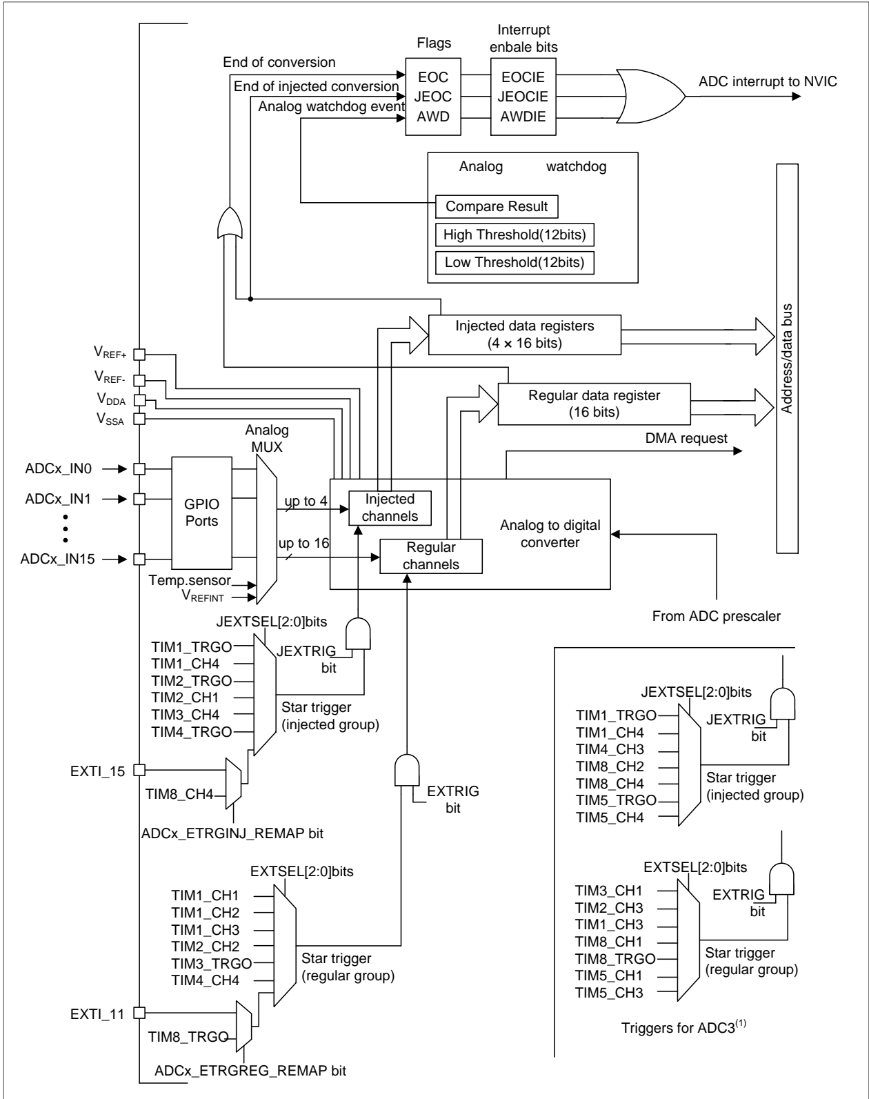
Figure 9-1 Single ADC block diagram
