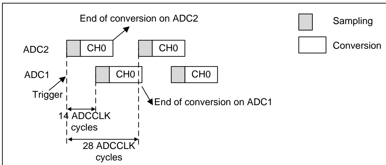
Figure 9-12 Slow interleaved mode on 1 channel
