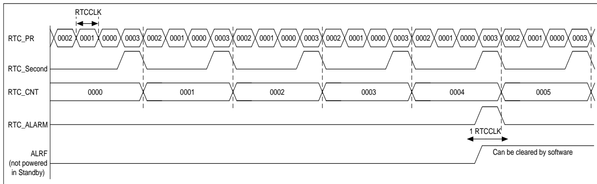
Figure 15-3 RTC Overflow waveform example with PR=0003
