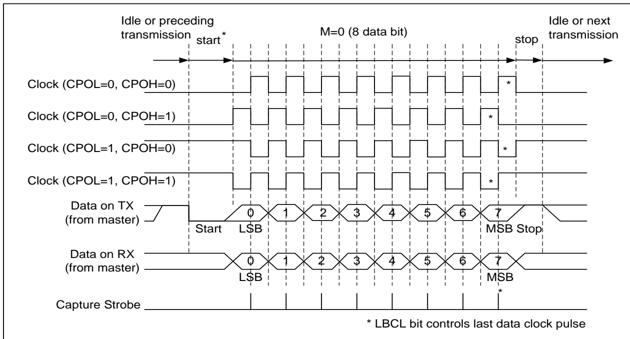
Figure 24-12 USART data clock timing diagram (M=0)
