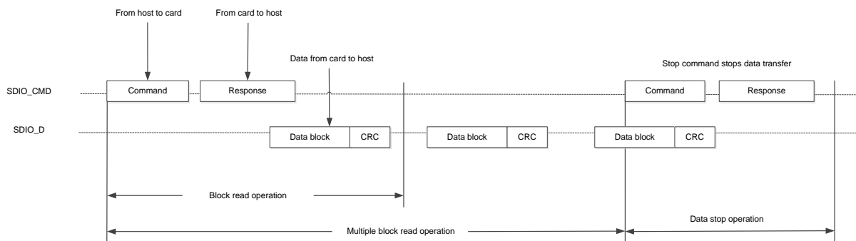
Figure 19-2 SDIO (multiple) block read operation
