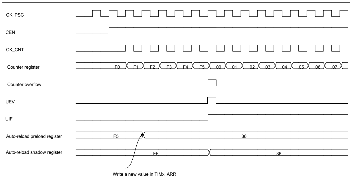
Figure 13-9 Counter timing diagram, update event when ARPE=1(TIMx_ARR preloaded)
