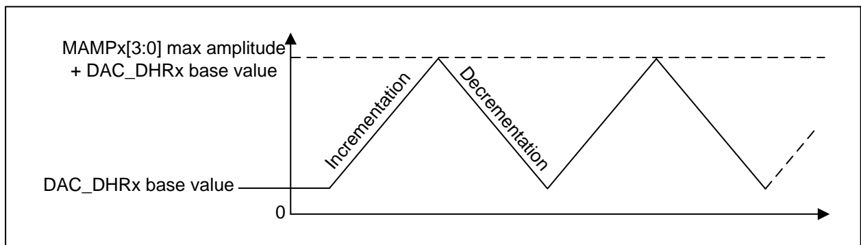
Figure 10-7 DAC triangle wave generation
