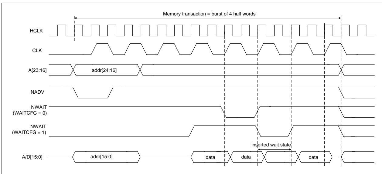
Figure 18-18 Wait configurations
