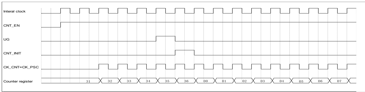
Figure 14-10 Control circuit in normal mode, internal clock divided by 1
