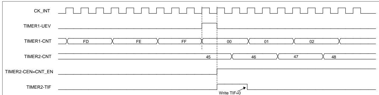
Figure 13-44 Triggering timer 2 with update of timer 1
