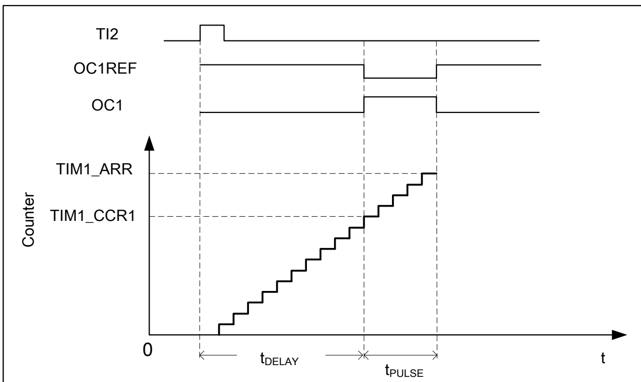
Figure 13-33 Example of one pulse mode
