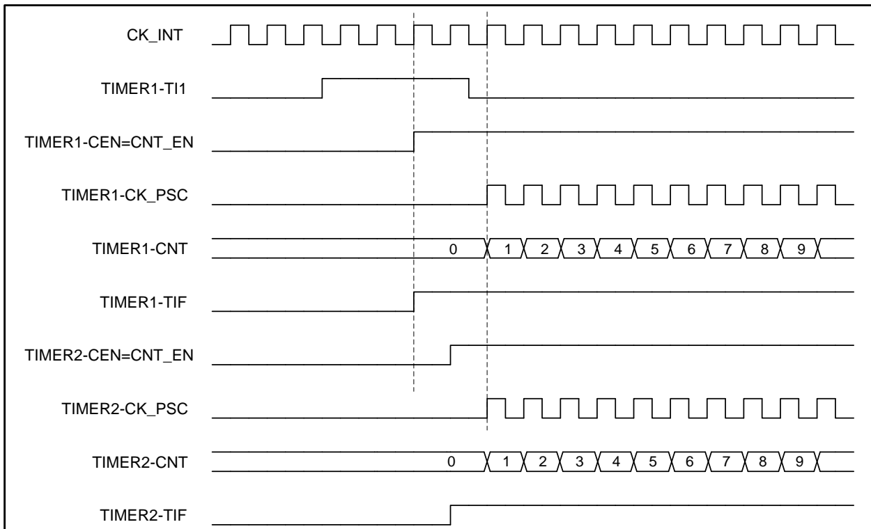
Figure 13-46 Triggering timer 1 and 2 with timer 1 T11 input
