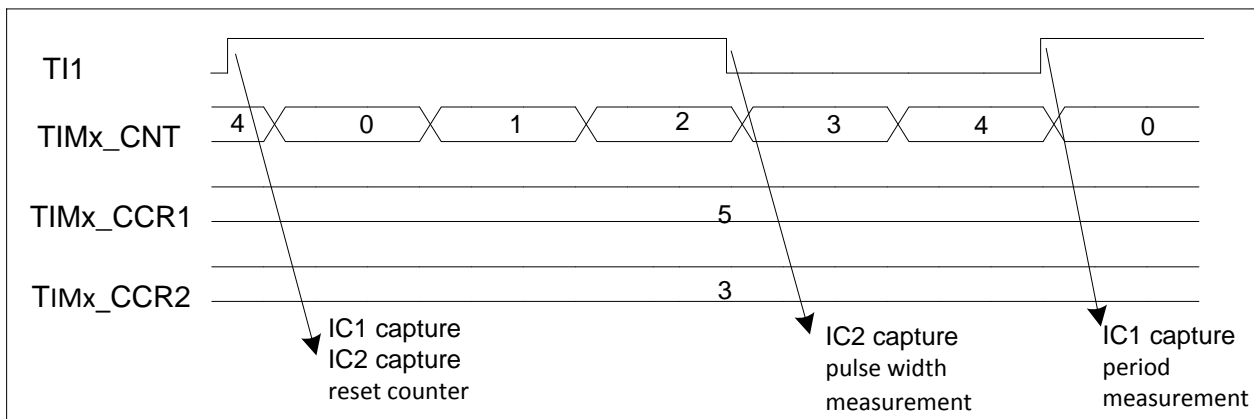
Figure 13-29 PWM input mode timing
