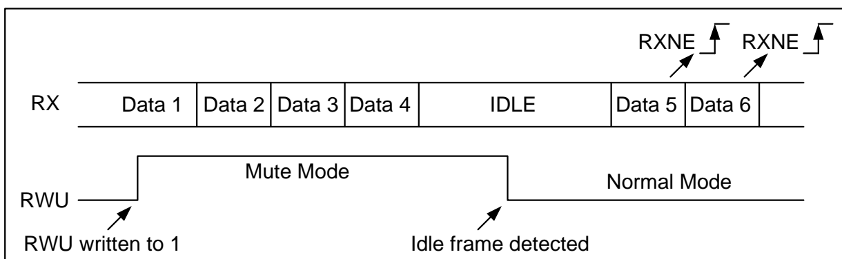
Figure 24-7 Mute mode using Idle line detection
