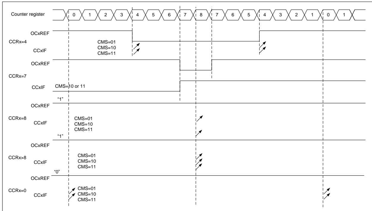
Figure 13-32 Center-aligned PWM waveforms (ARR=8)
