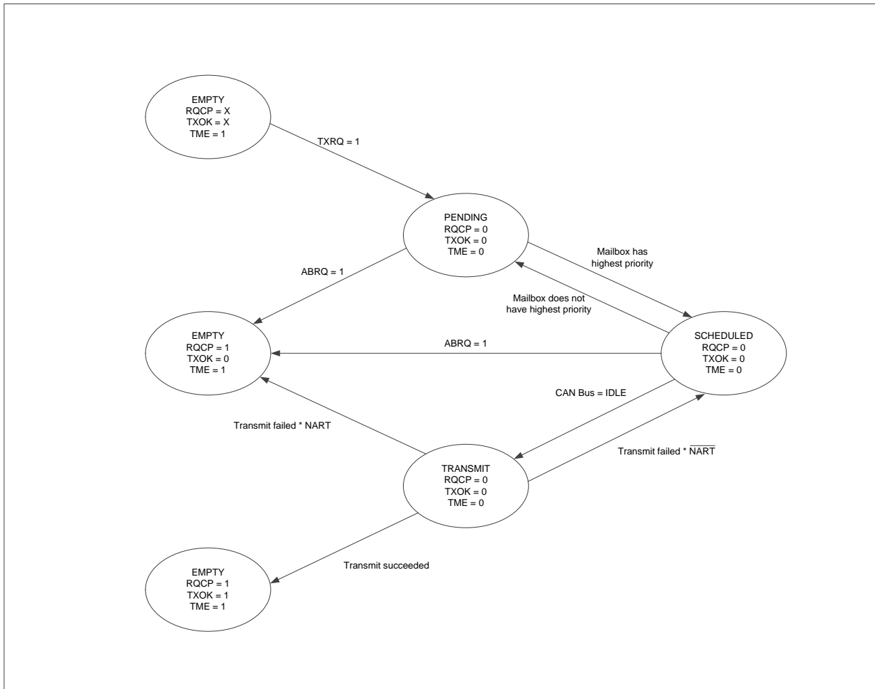
Figure 21-6 Transmit mailbox states
