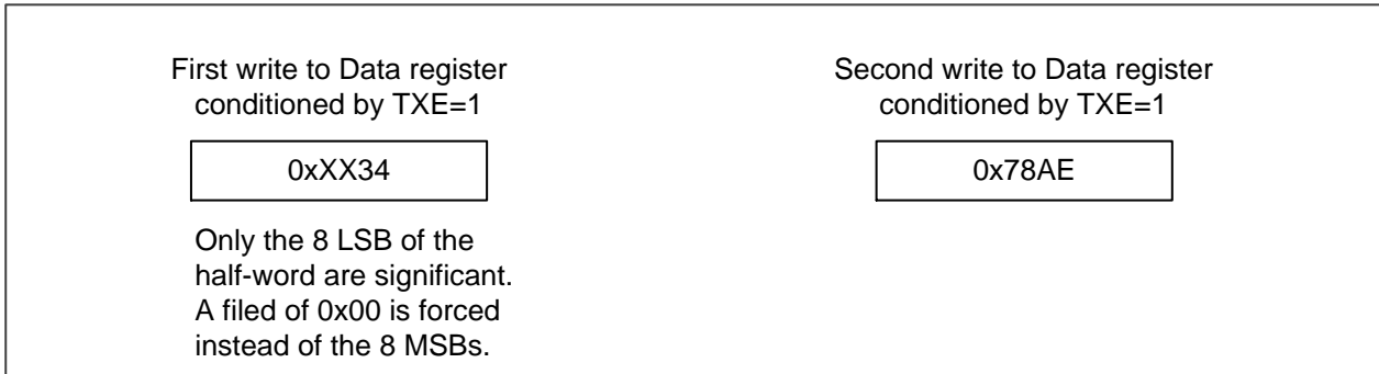
Figure 22-24 Operations required to transmit 0x3478AE
