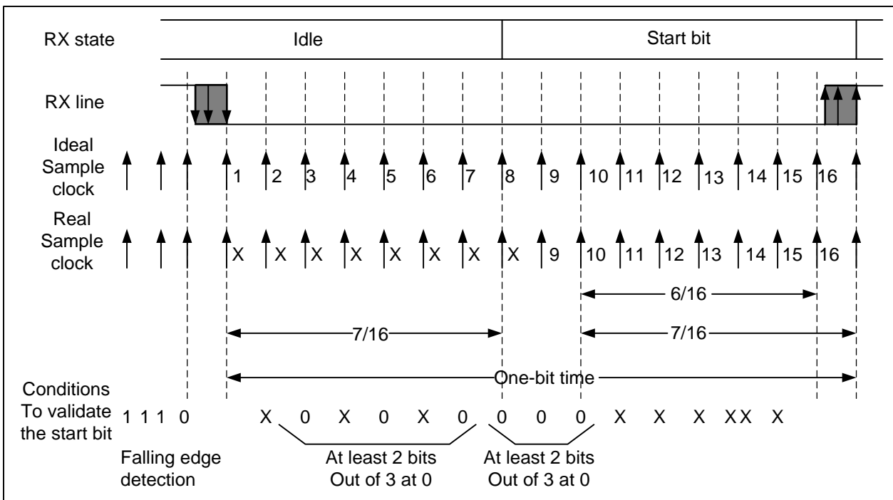
Figure 24-5 start bit detection
