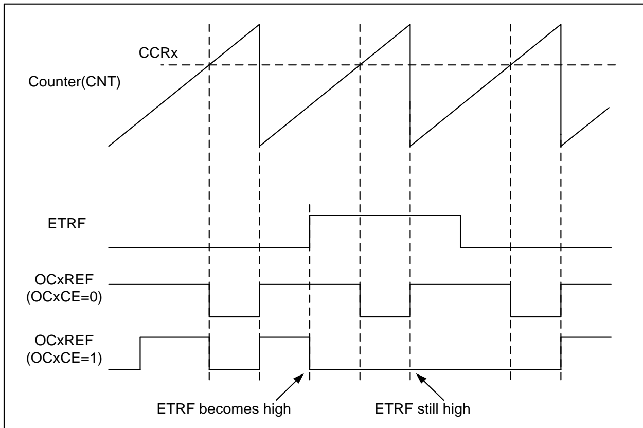
Figure 13-34 Clearing TIMx OCxREF
