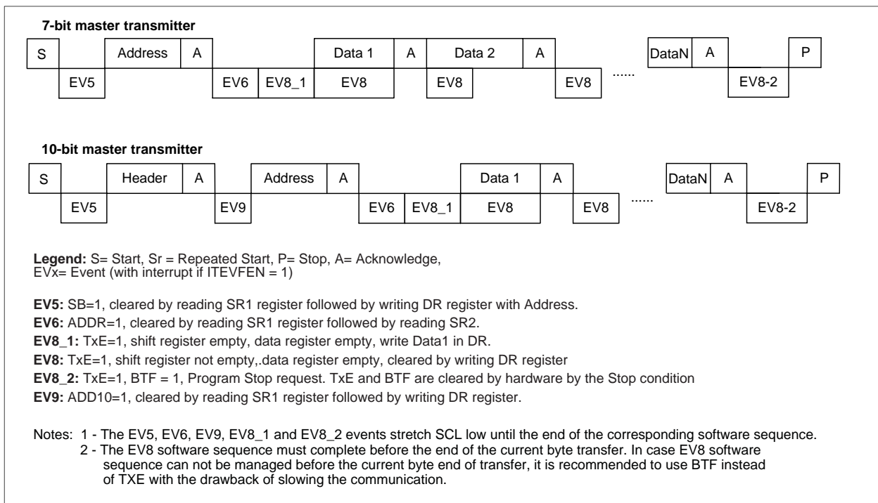
Figure 23-5 Transfer sequence diagram for master transmitter
