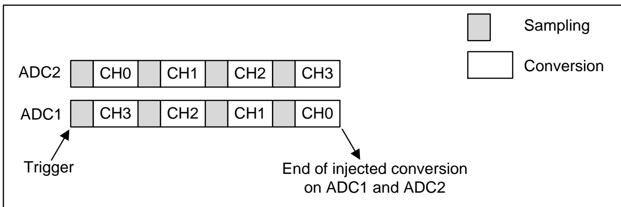
Figure 9-9 Injected simultaneous mode on 4 channels
