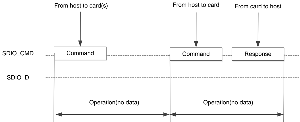
Figure 19-1 SDIO “no response” and “no data” operation
