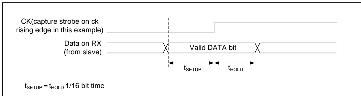
Figure 24-14 RX data setup/hold time
