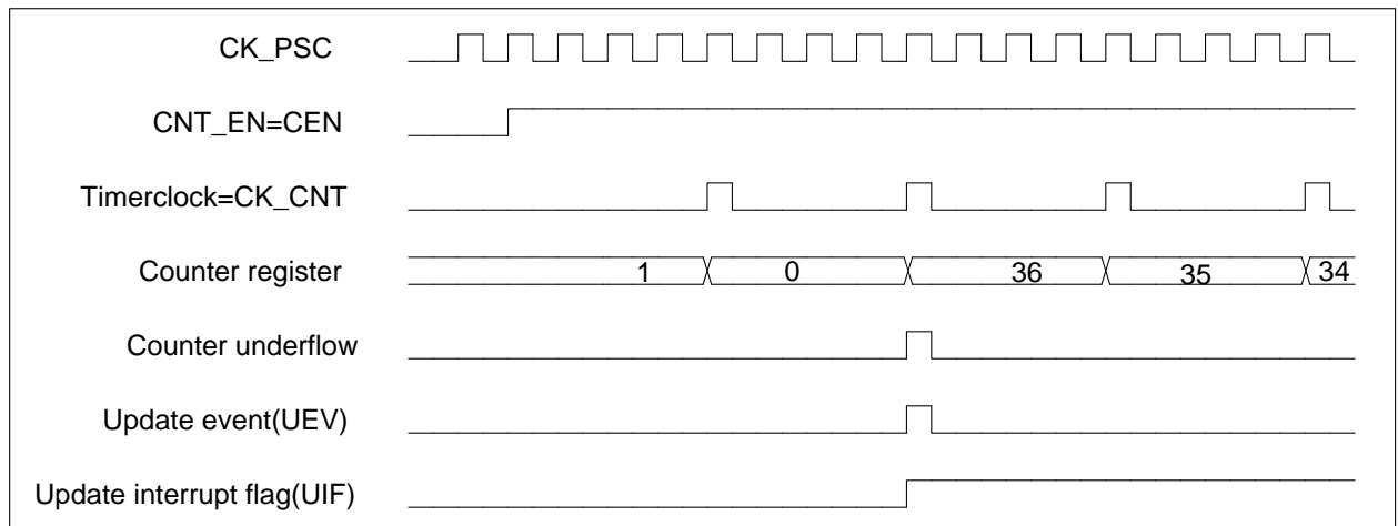
Figure 12-12 Counter timing diagram, internal clock divided by 4
