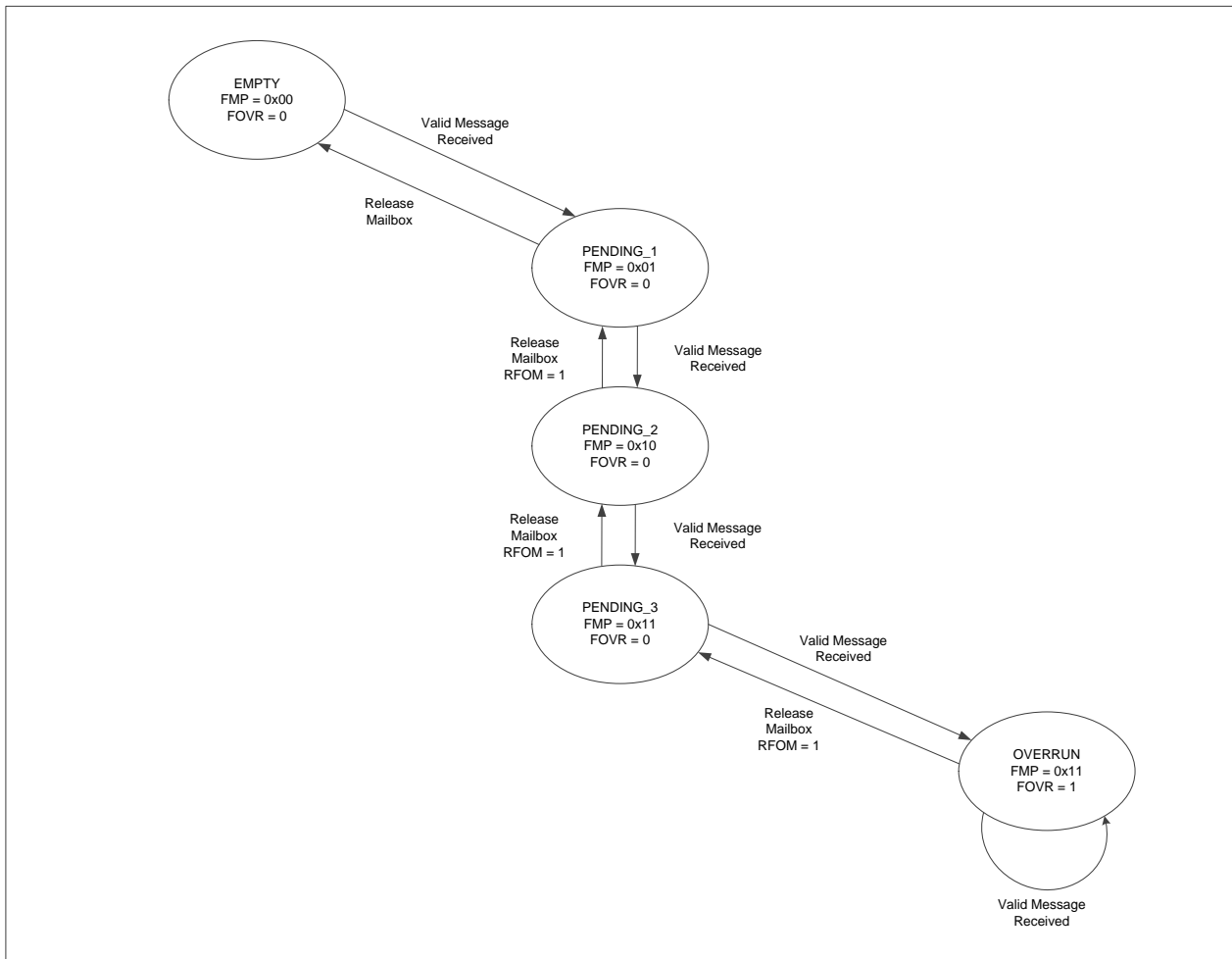
Figure 21-7 Receive FIFO states
