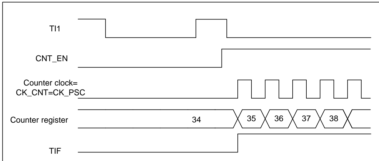
Figure 12-47 Control circuit in trigger mode
