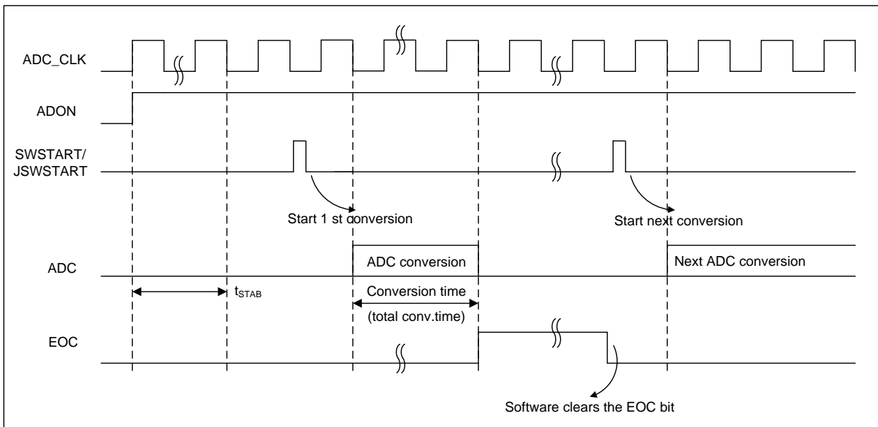
Figure 9-2 Timing diagram
