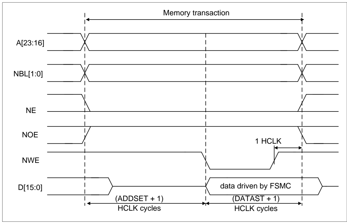
Figure 18-4 Mode1 write accesses
