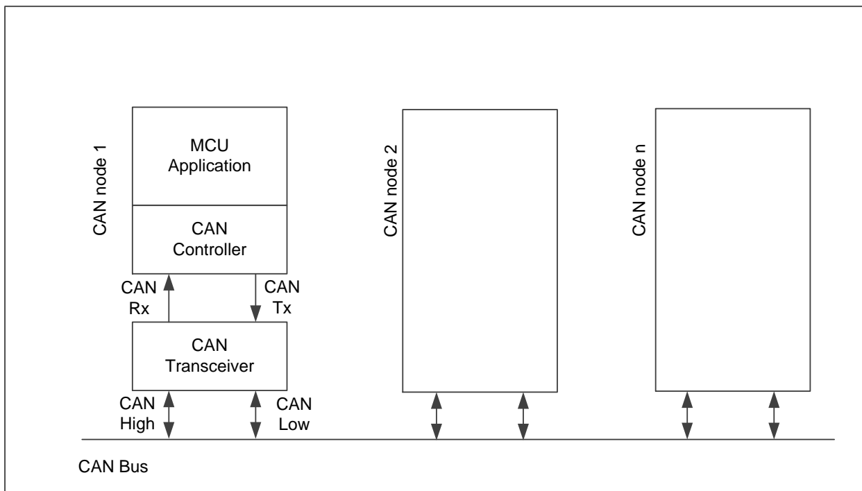
Figure 21-1 CAN network topology
