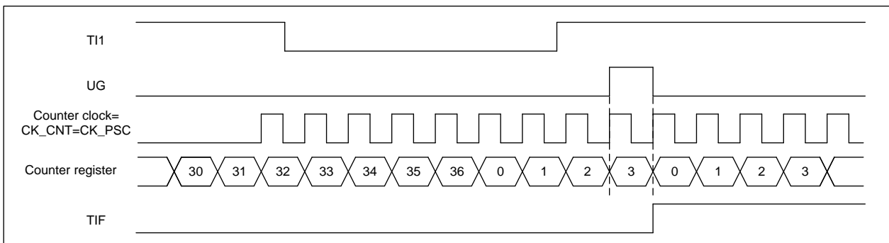
Figure 12-45 Control circuit in reset mode
