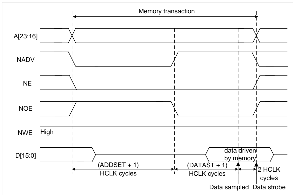
Figure 18-10 Mode C read accesses
