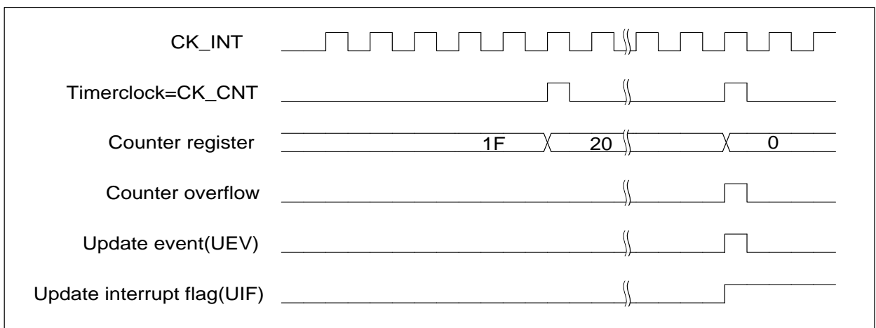
Figure 14-7 Counter timing diagram, internal clock divided by N
