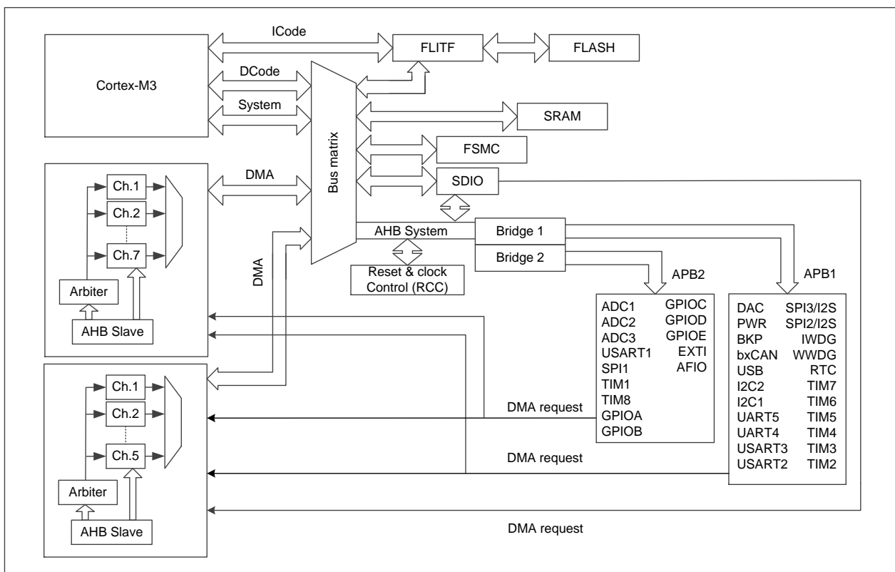
Figure 2-1 System architecture
