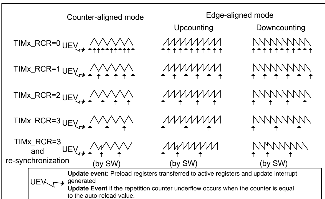
Figure 12-21 Update rate examples depending on mode and TIMx_RCR register settings
