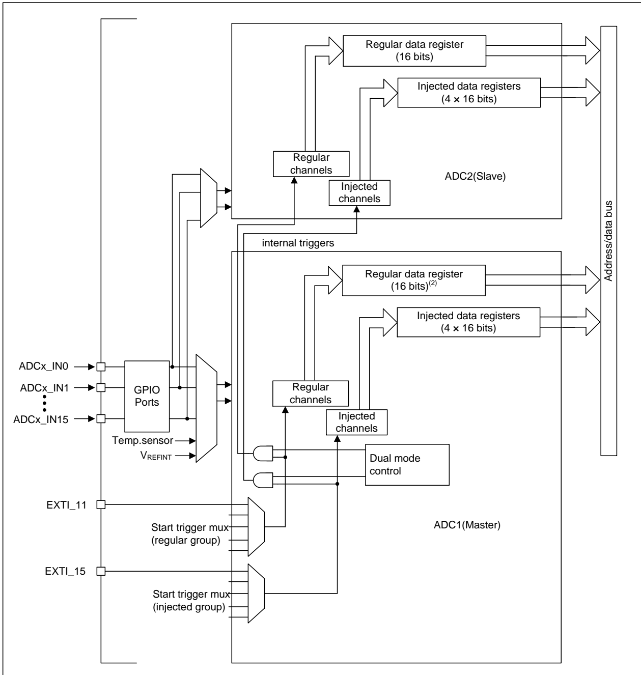
Figure 9-8 Dual ADC block diagram (1)
