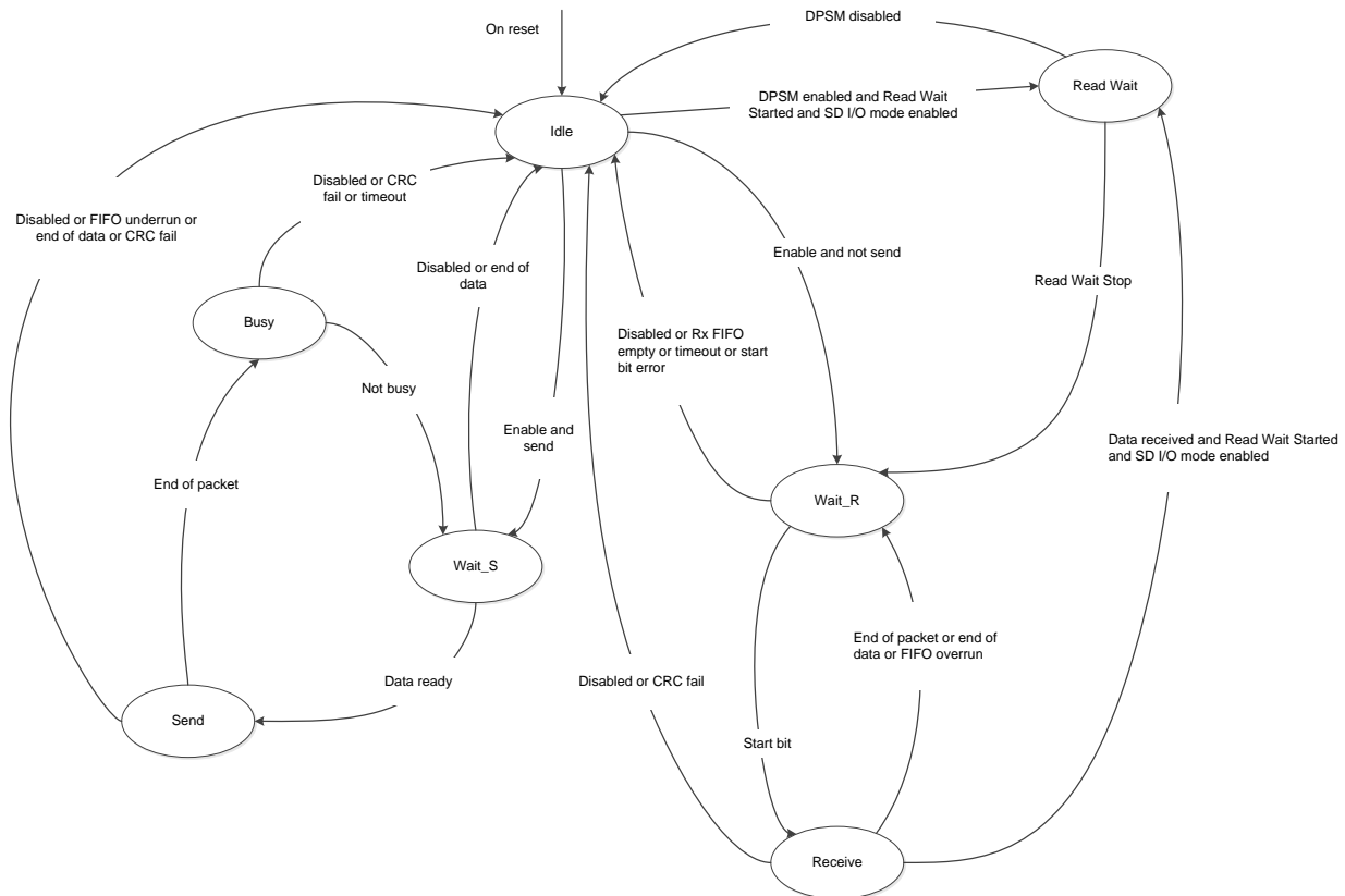
Figure 19-13 Data path state machine (DPSM)
