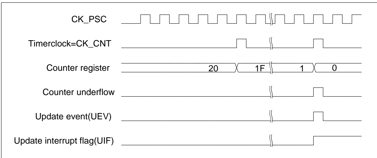
Figure 12-18 Counter timing diagram, internal clock divided by N
