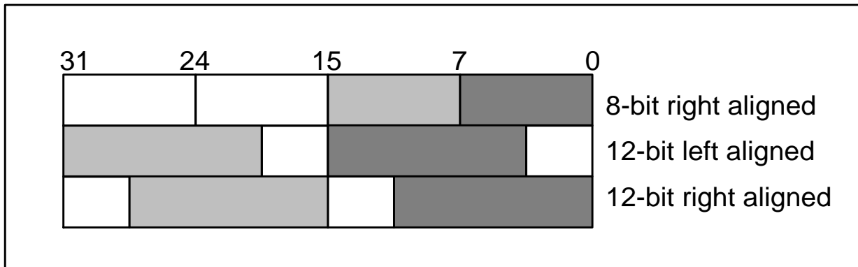
Figure 10-3 Data registers in dual DAC channel mode
