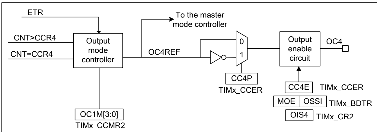
Figure 12-30 Output stage of capture/compare channel (channel 4)
