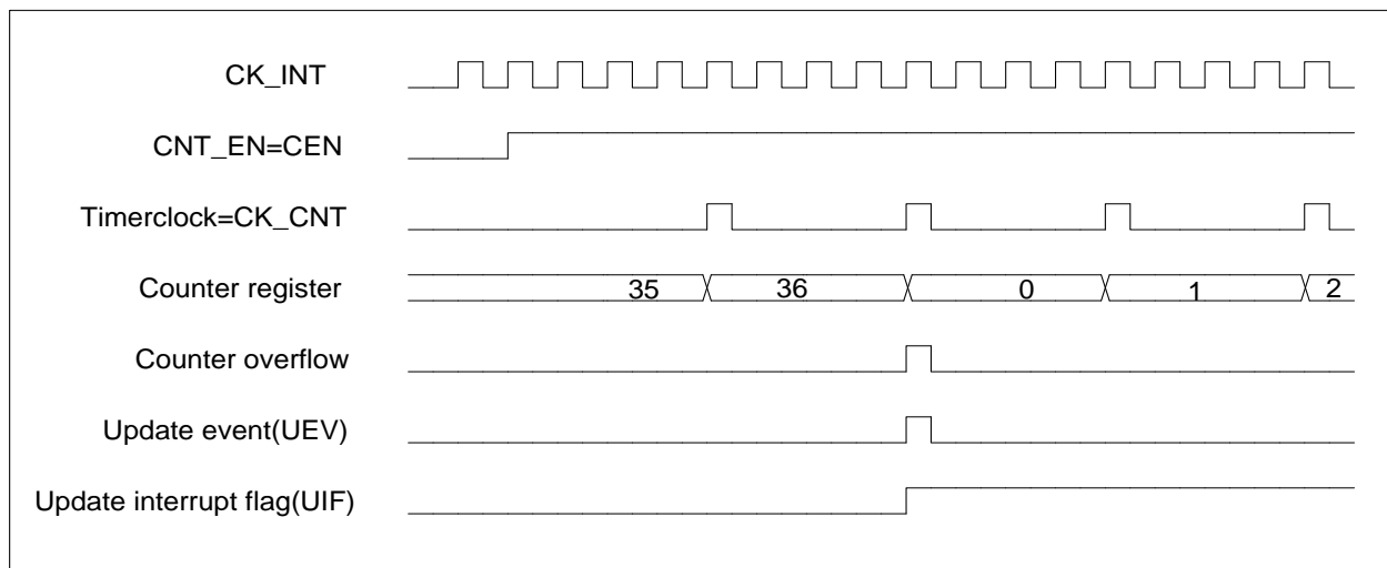
Figure 14-6 Counter timing diagram, internal clock divided by 4
