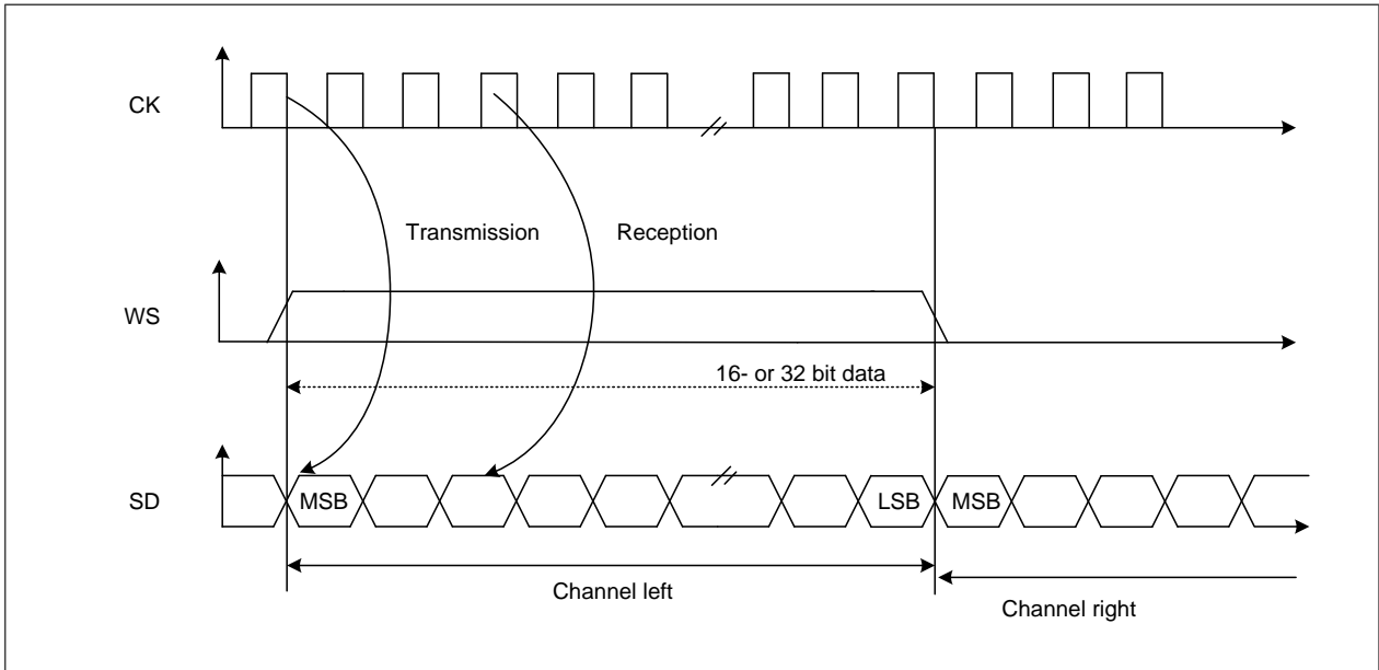
Figure 22-19 MSB justified 16-bit or 32-bit full-accuracy length with CPOL = 0
