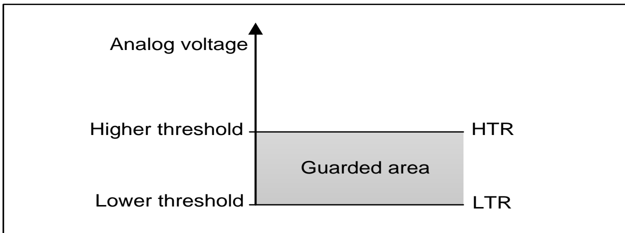
Figure 9-3 Analog watchdog guarded area
