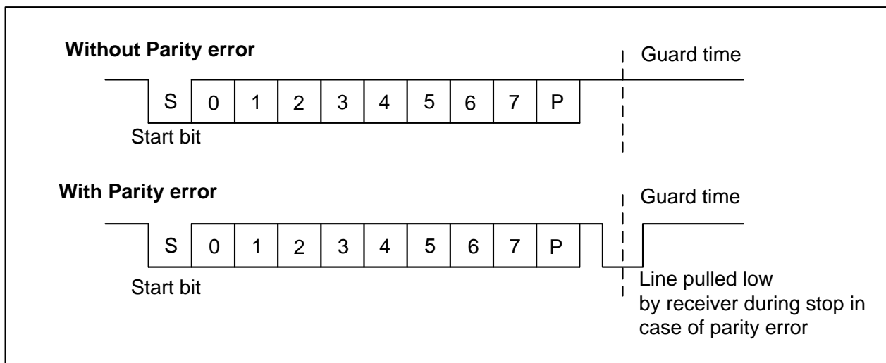
Figure 24-15 ISO 7816-3 asynchronous protocol
