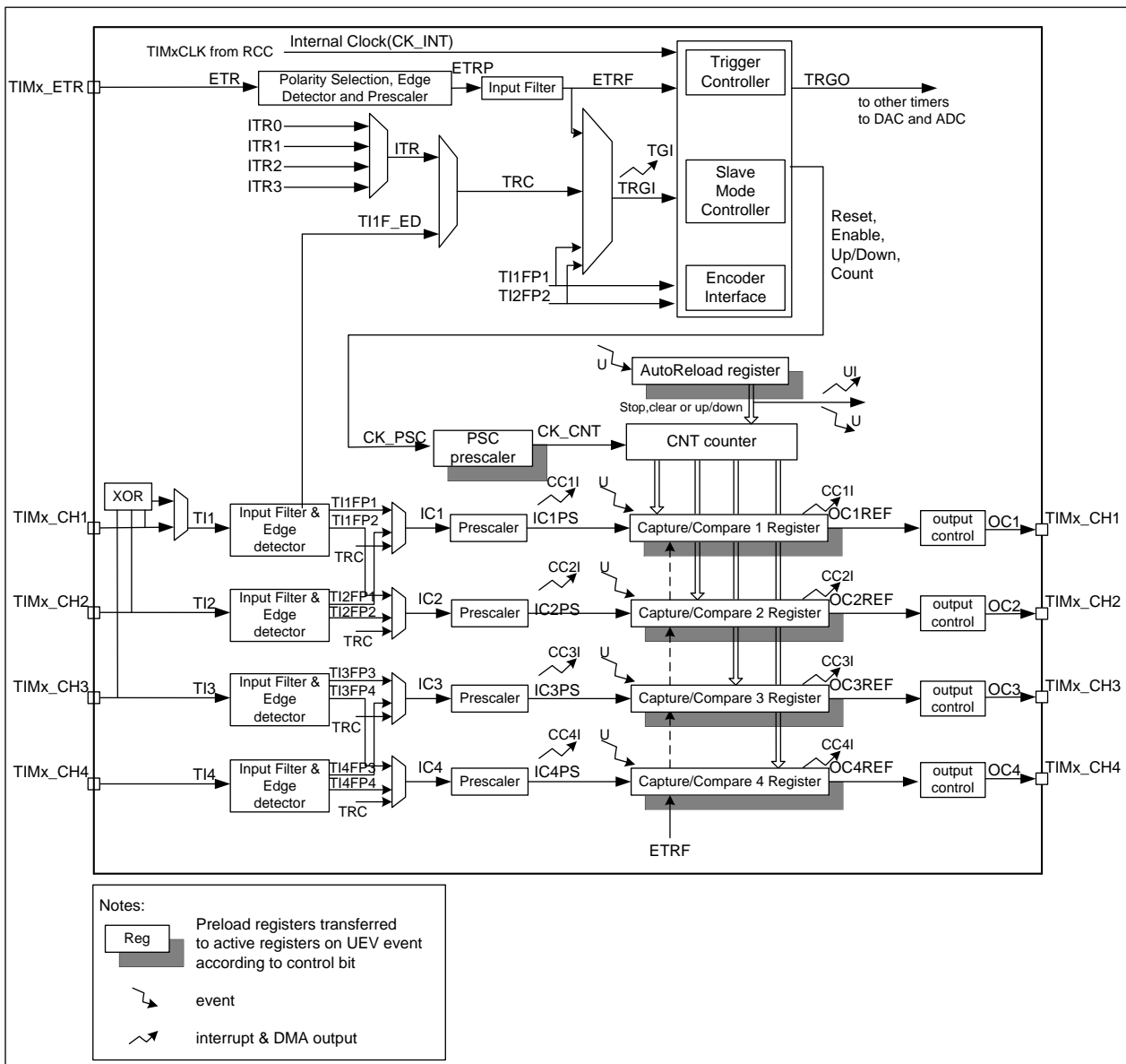
Figure 13-1 General-purpose timer block diagram
