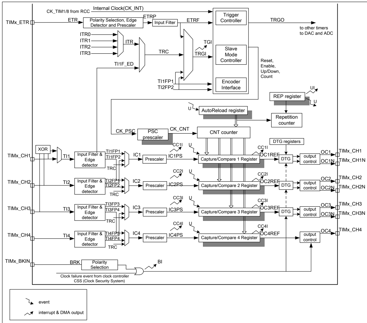
Figure 12-1 Advanced-control timer block diagram
