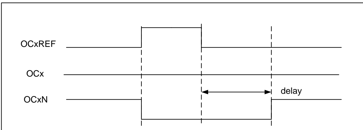
Figure 12-37 Dead-time waveforms with delay greater than the positive pulse
