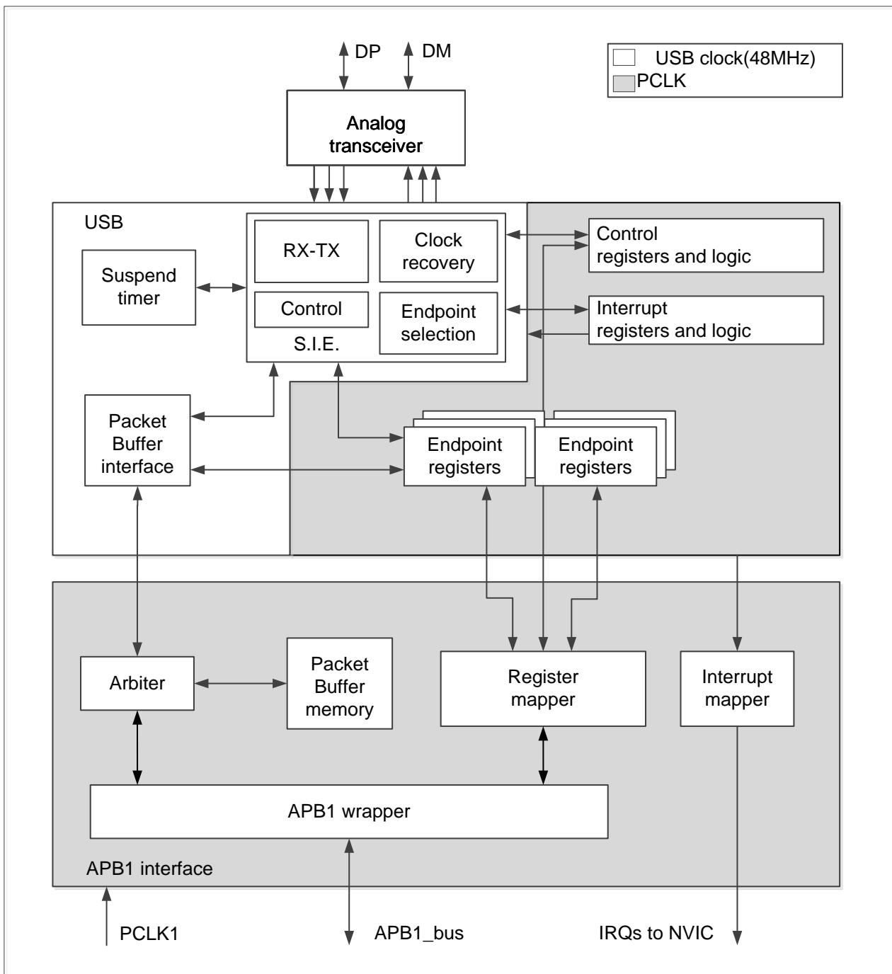
Figure 20-1 USB peripheral block diagram
