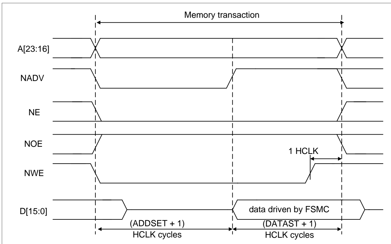
Figure 18-9 Mode B write accesses
