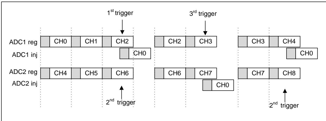
Figure 9-16 Case of trigger occurring during injected conversion
