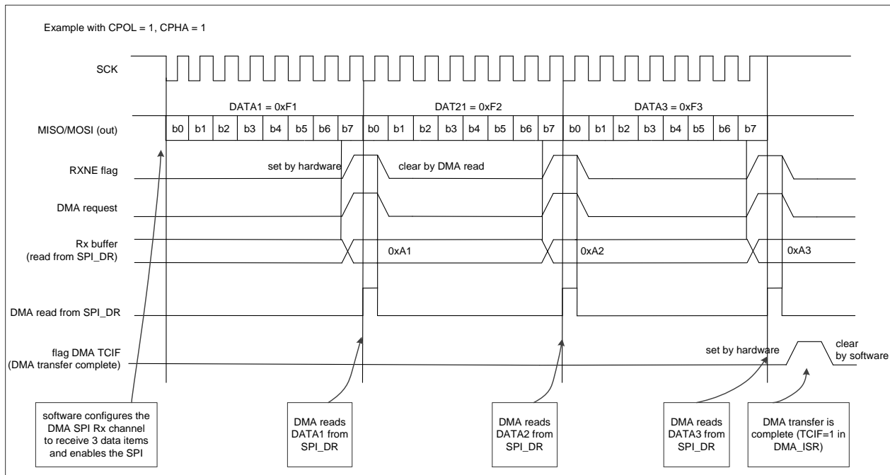
Figure 22-11 Reception using DMA
