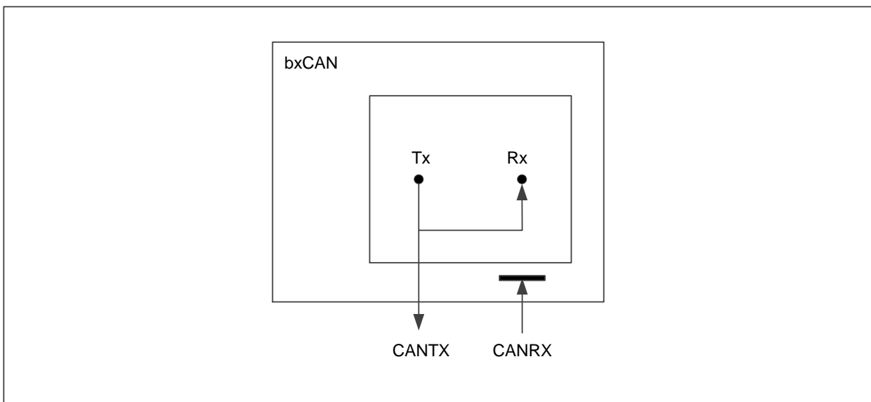
Figure 21-4 bxCAN in loop back mode
