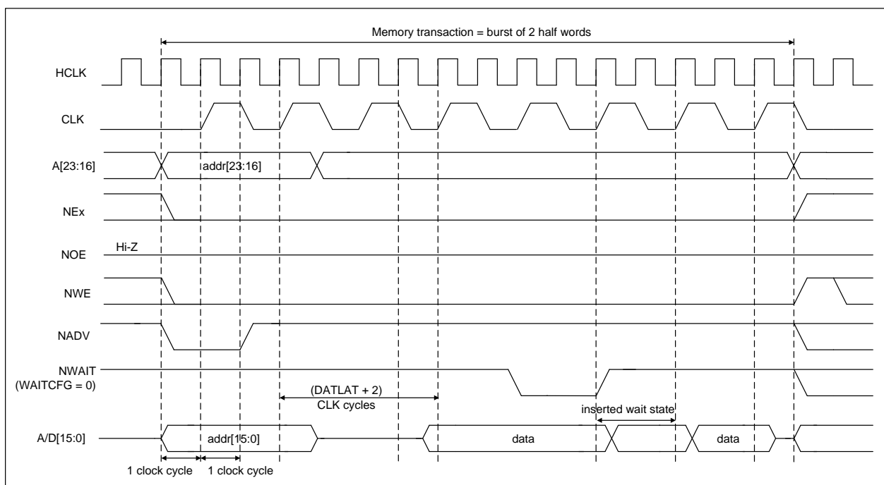
Figure 18-20 Synchronous multiplexed write mode - PSRAM (CRAM)
