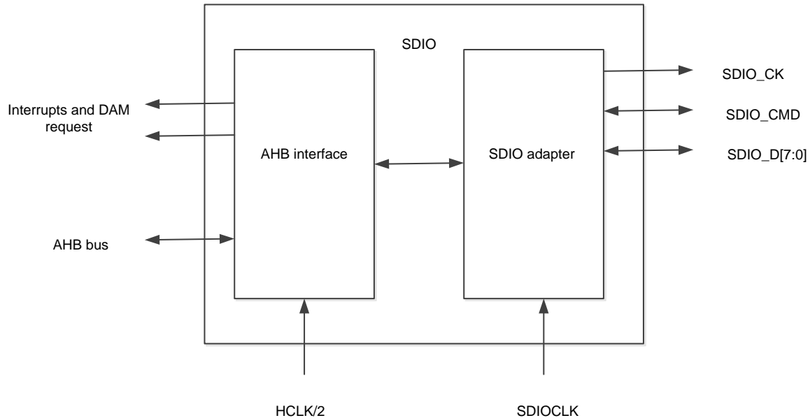
Figure 19-6 SDIO block diagram
