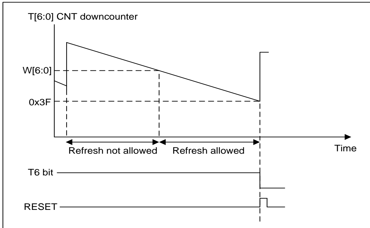
Figure 17-2 Window watchdog timing diagram
