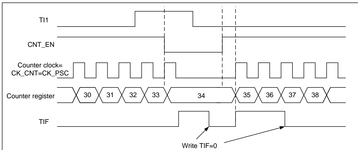
Figure 12-46 Control circuit in gated mode
