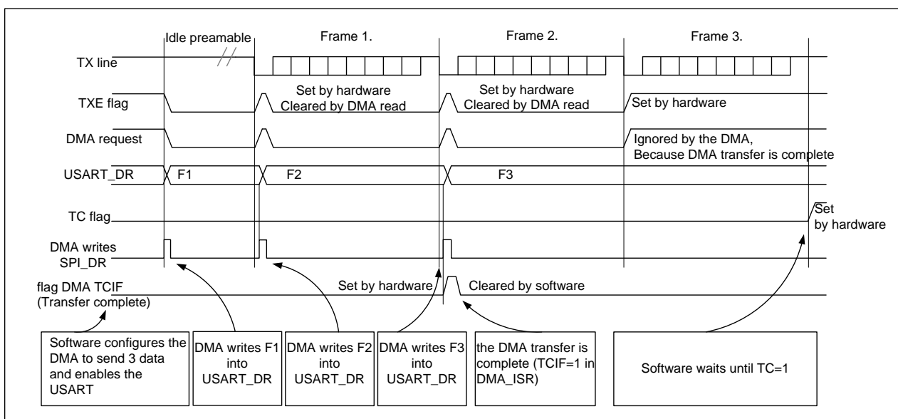
Figure 24-19 Transmission using DMA
