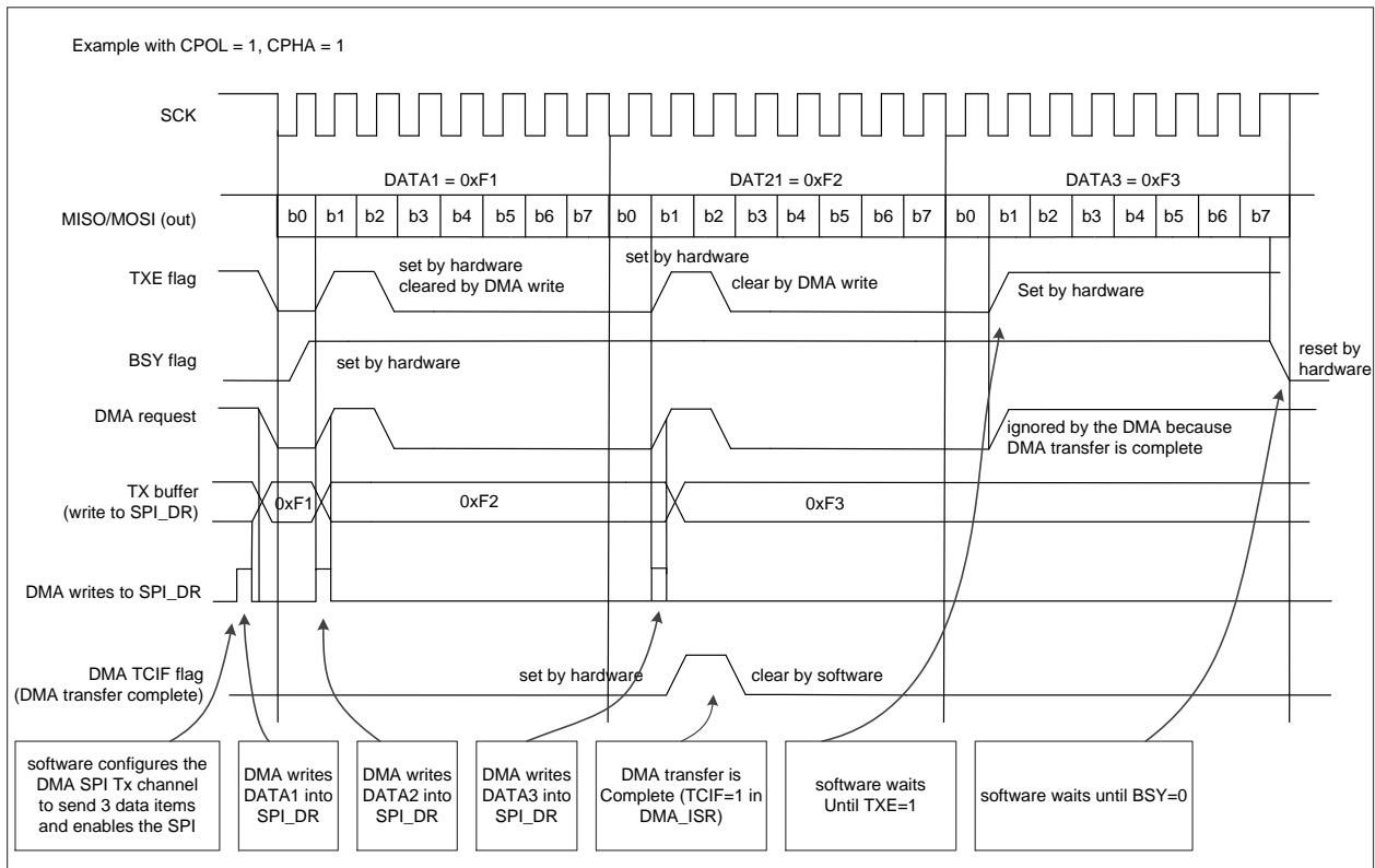
Figure 22-10 Transmission using DMA
