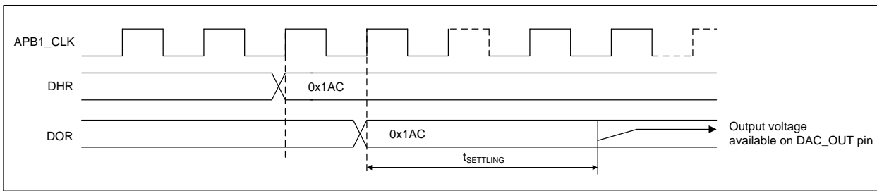
Figure 10-4 Timing diagram for conversion with trigger disabled TEN = 0
