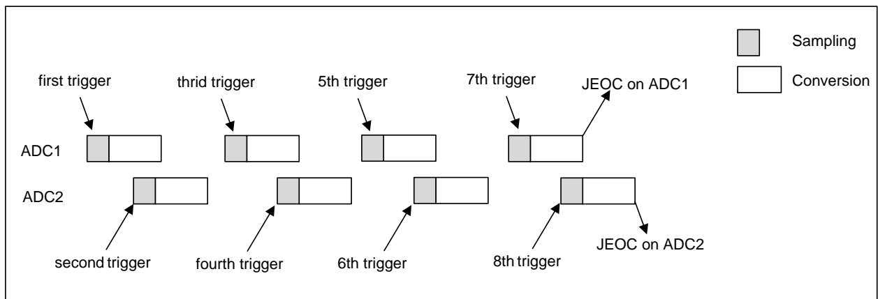
Figure 9-14 Alternate trigger: 4 injected channels (each ADC) in discontinuous model
