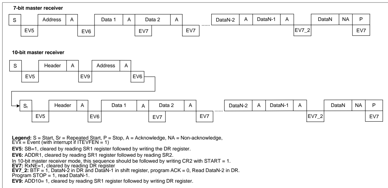
Figure 23-7 Method 2: transfer sequence diagram for master receiver when N>2
