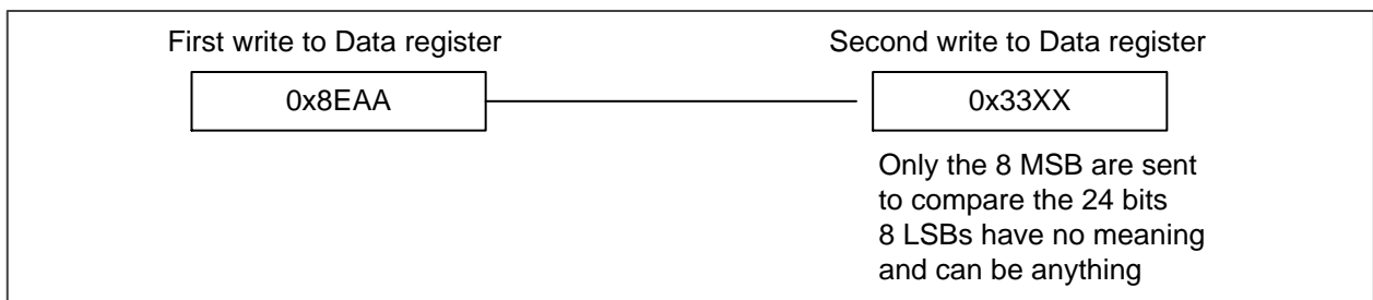
Figure 22-15 Transmitting 0x8EAA33
