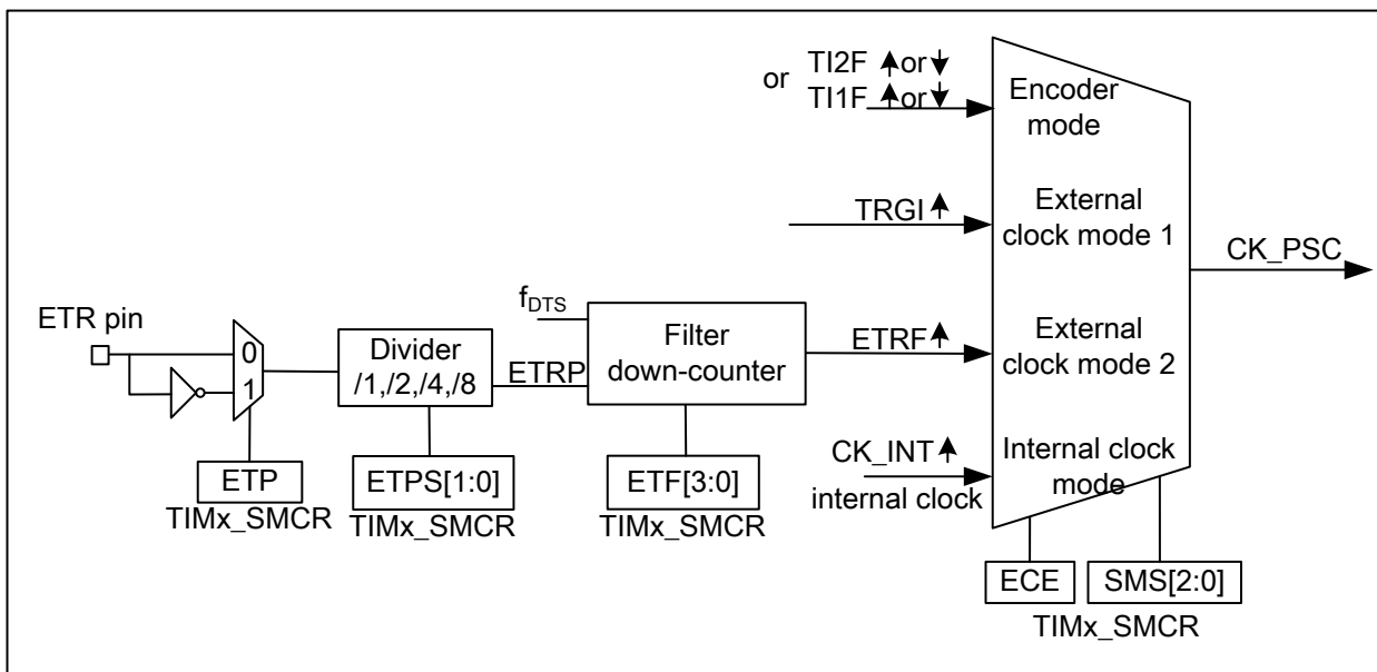
Figure 12-25 External trigger input block
