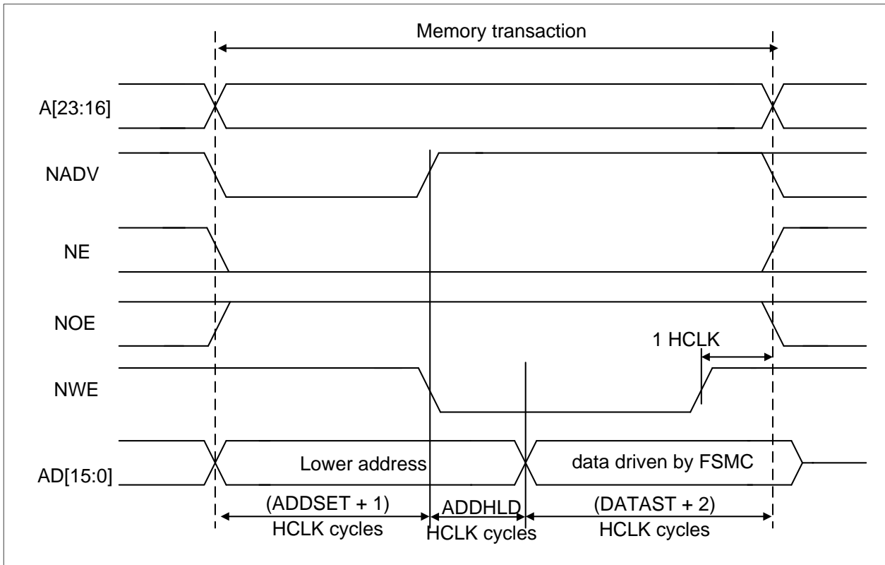
Figure 18-15 Multiplexed write accesses
