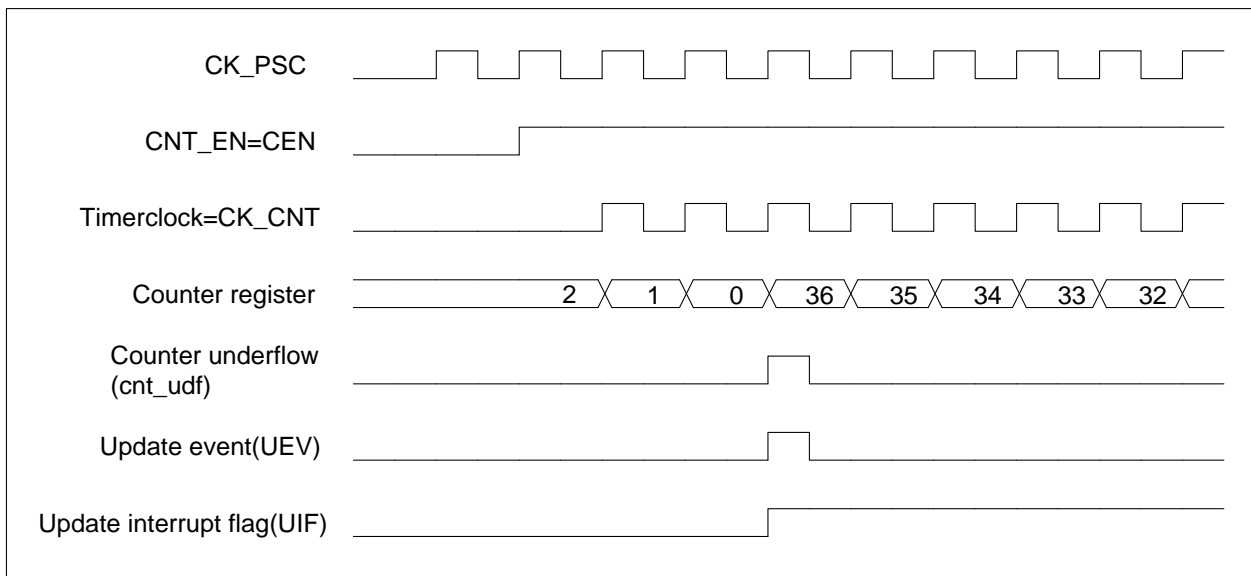
Figure 12-10 Counter timing diagram, internal clock divided by 1
