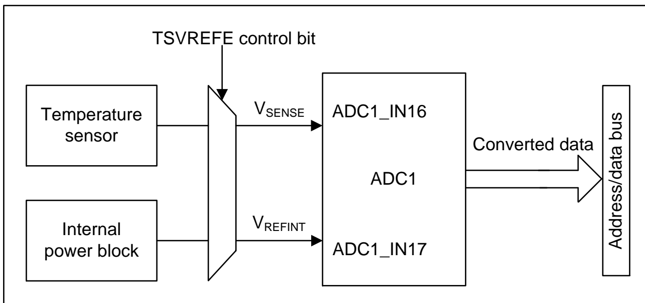
Figure 9-18 Temperature sensor and V_{REFINT} channel block diagram
