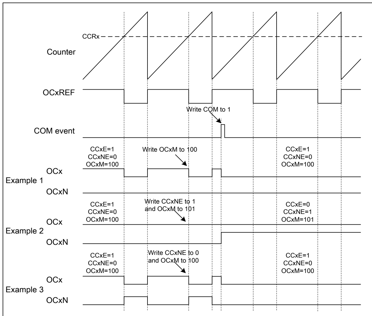
Figure 12-40 6-step generation, COM example (OSSR=1)
