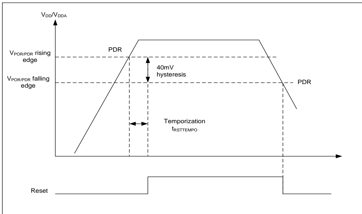
Figure 4-2 Power on reset/power down reset waveform
