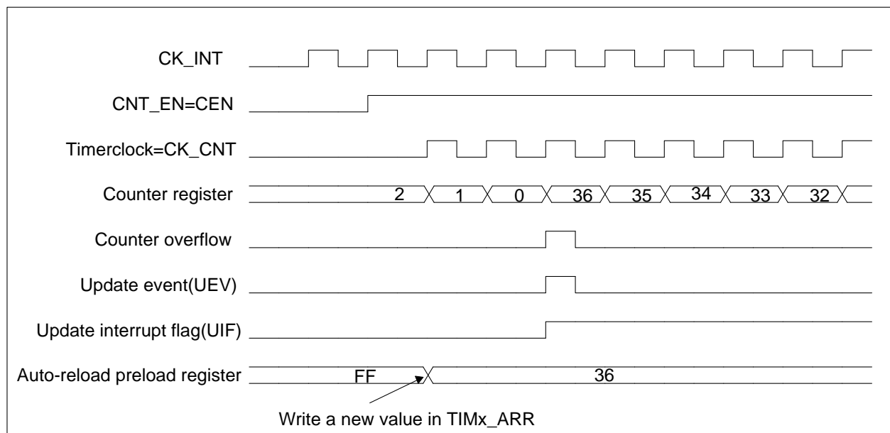
Figure 13-14 Counter timing diagram, update event
