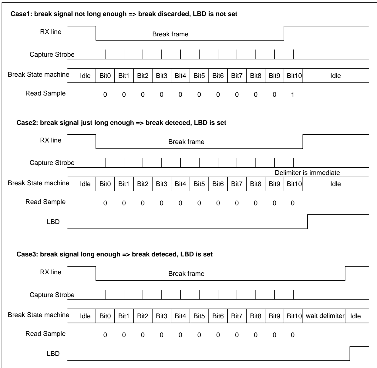
Figure 24-9 Break detection in LIN mode (11-bit break length - LBDL bit is set)
