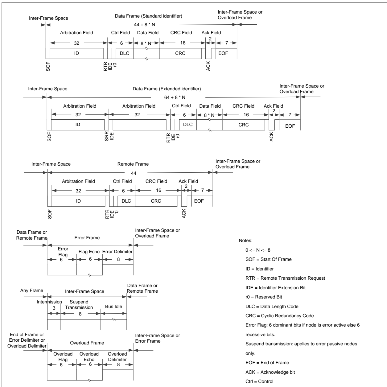
Figure 21-13 CAN frames
