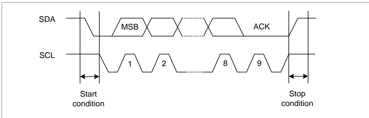
Figure 23-1 I2C bus protocol
