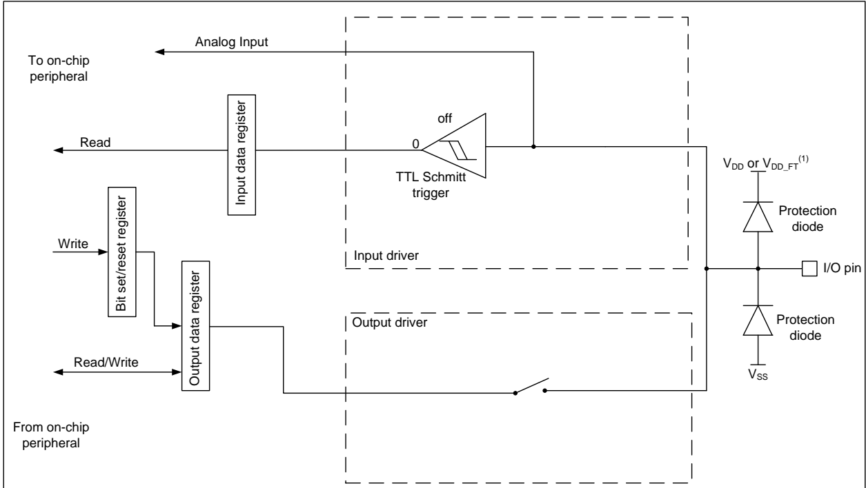
Figure 7-6 High impedance-analog configuration
