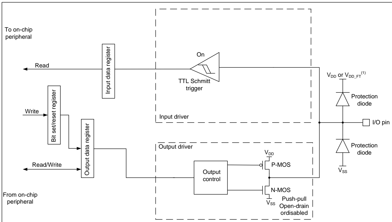
Figure 7-4 Output configuration
