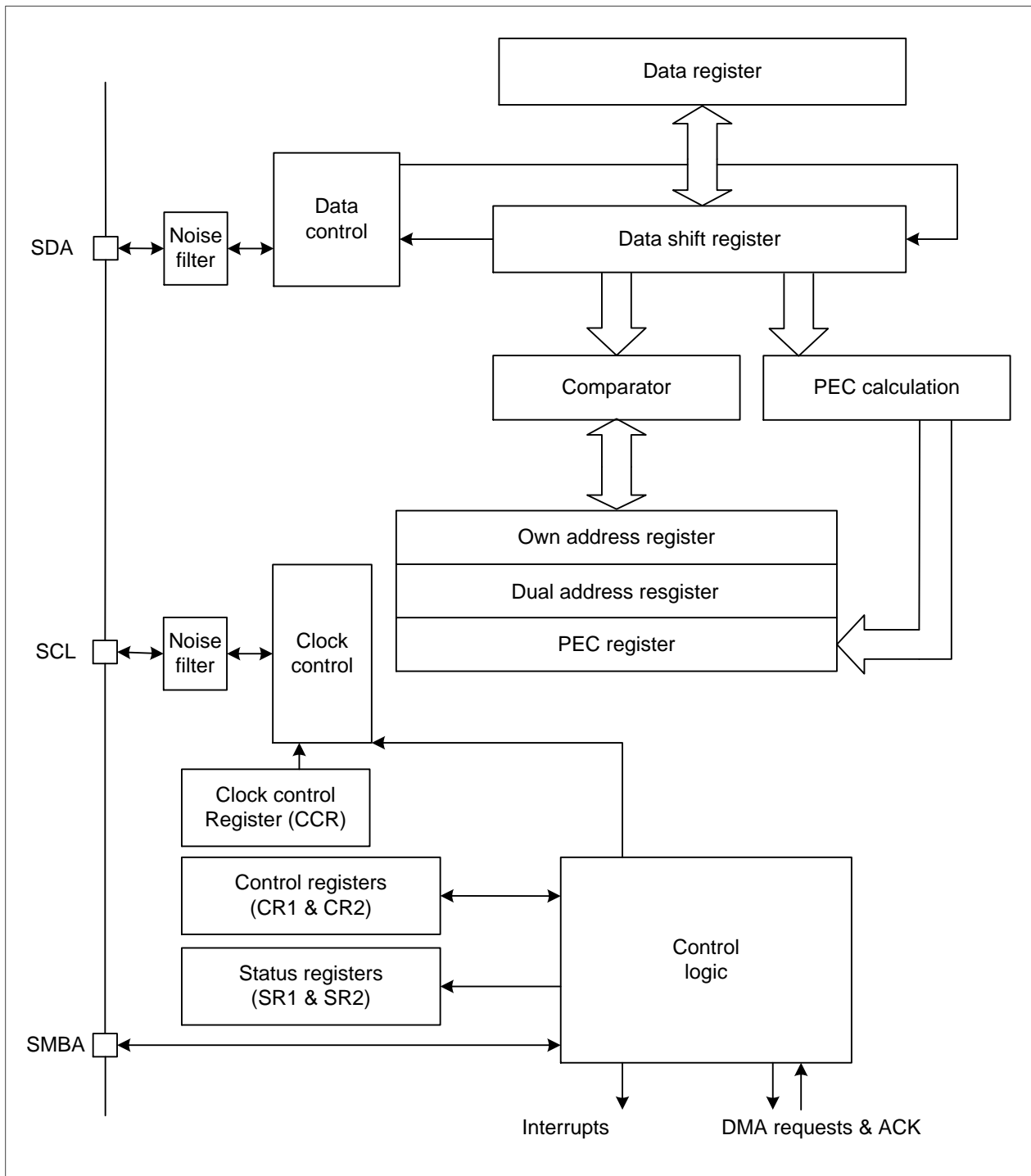
Figure 23-2 I2C block diagram
