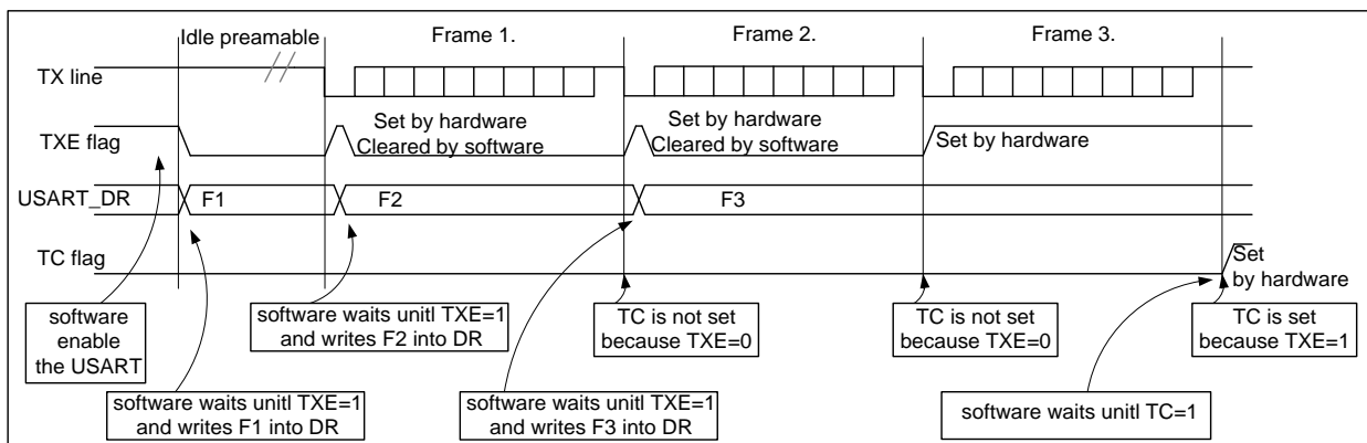
Figure 24-4 TC/TXE behavior when transmitting
