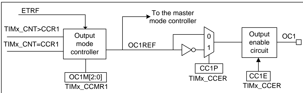
Figure 13-28 Output stage of capture/compare channel (channel 1)
