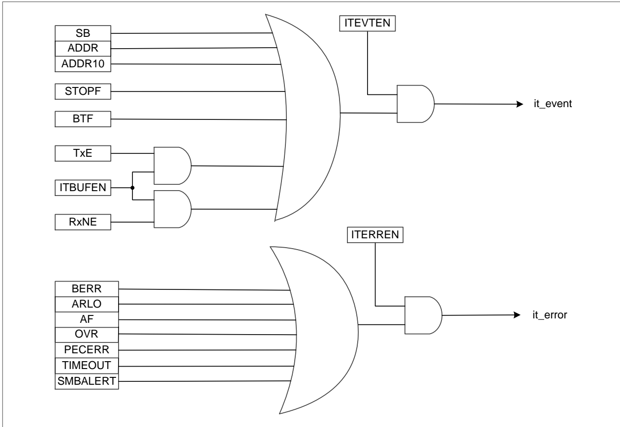
Figure 23-10 I2C interrupt mapping diagram
