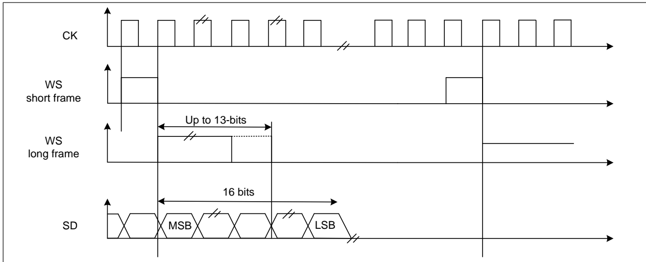
Figure 22-29 PCM standard waveforms (16-bit extended to 32-bit packet frame)
