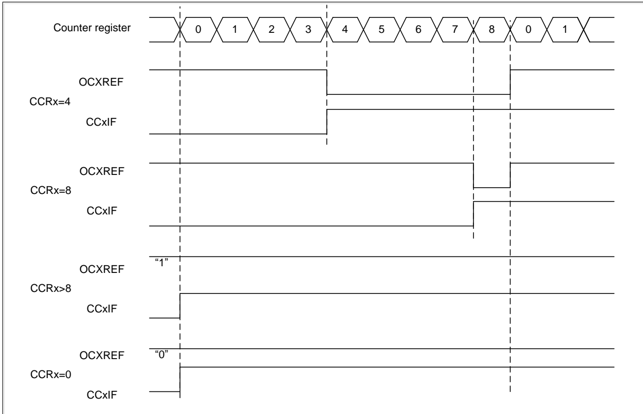
Figure 13-31 Edge-aligned PWM waveforms (ARR=8)
