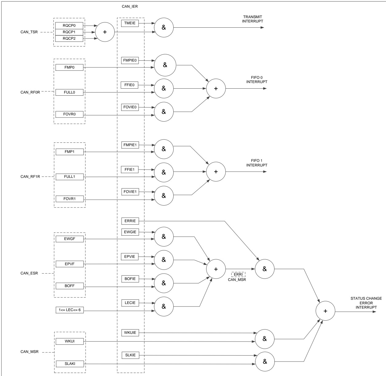
Figure 21-14 Event flags and interrupt generation
