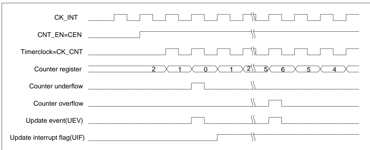
Figure 13-15 Counter timing diagram, internal clock divided by 1, TIMx_ARR = 0x6
