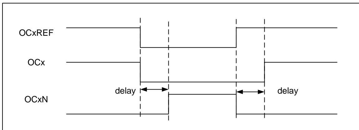
Figure 12-35 Complementary output with dead-time insertion
