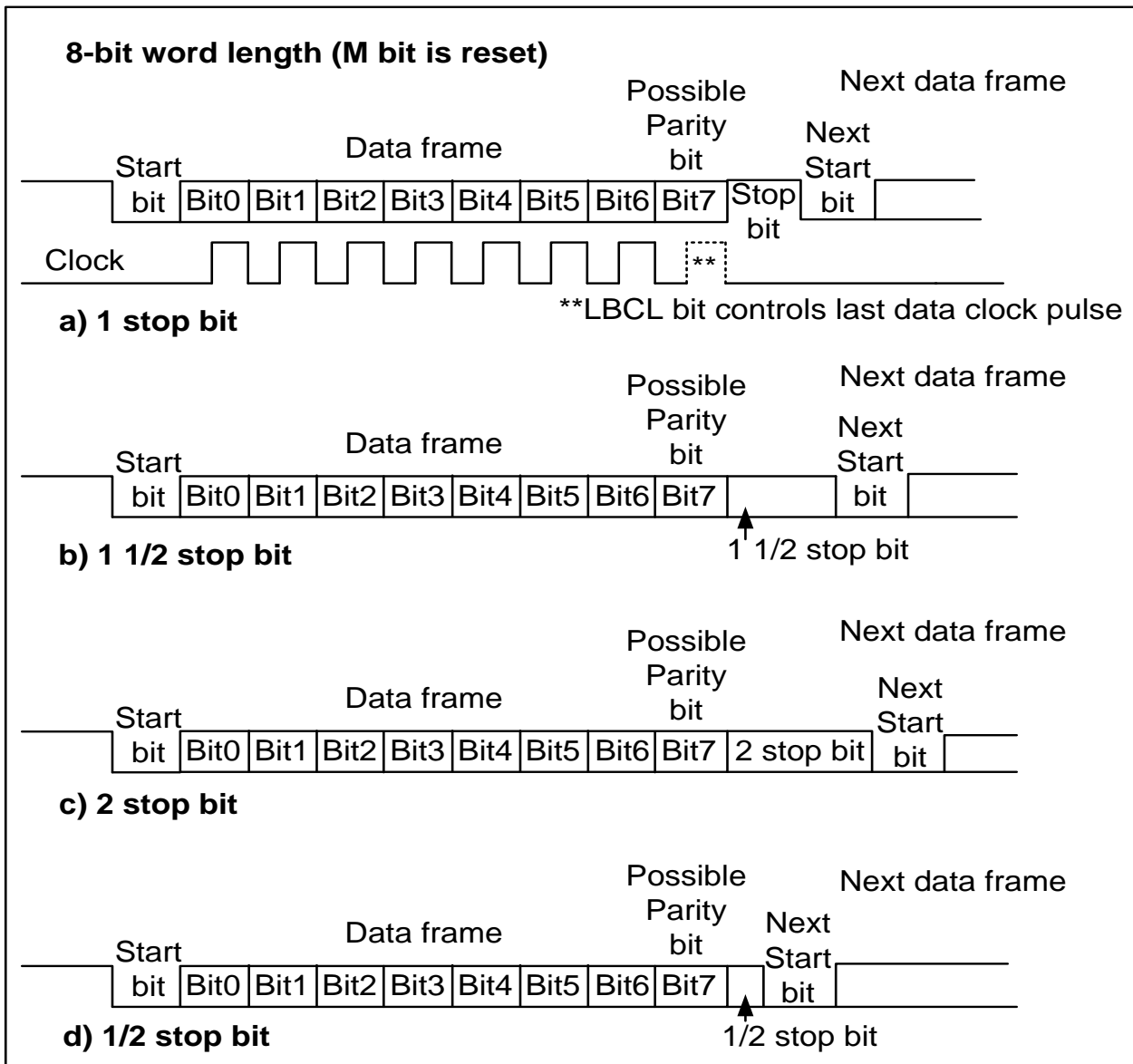
Figure 24-3 Configurable stop bits
