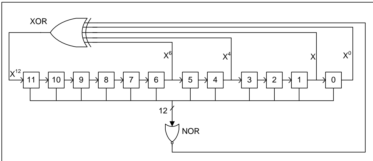
Figure 10-5 DAC LFSR register calculation algorithm
