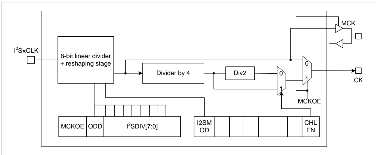
Figure 22-31 I2S clock generator architecture
