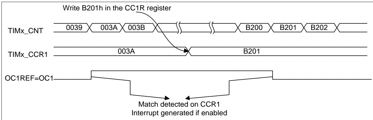
Figure 12-32 Output compare mode, toggle on OC
